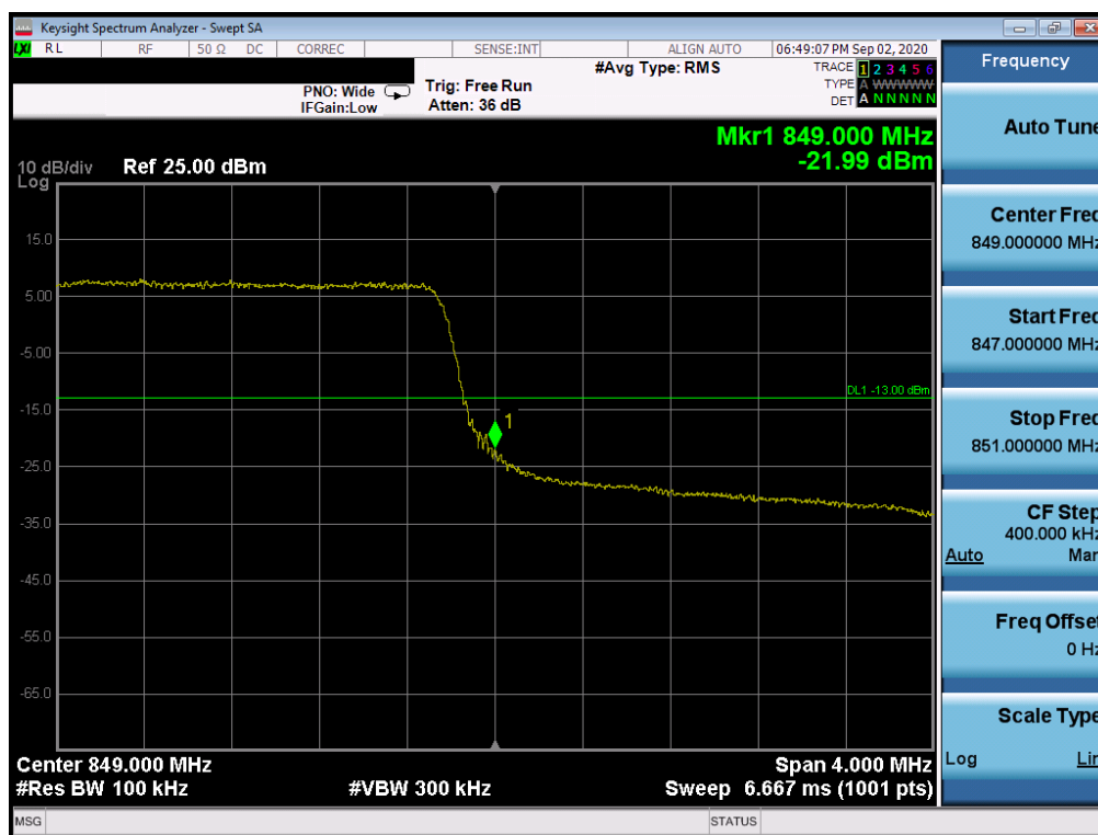
Plot 7-33. Upper Band Edge Plot (LTE Band 26/5 - 5MHz QPSK - Full RB Configuration)
