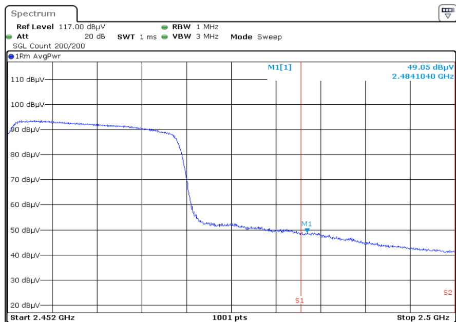
2452.0 F3 RestrictedBand Vertical AVG
