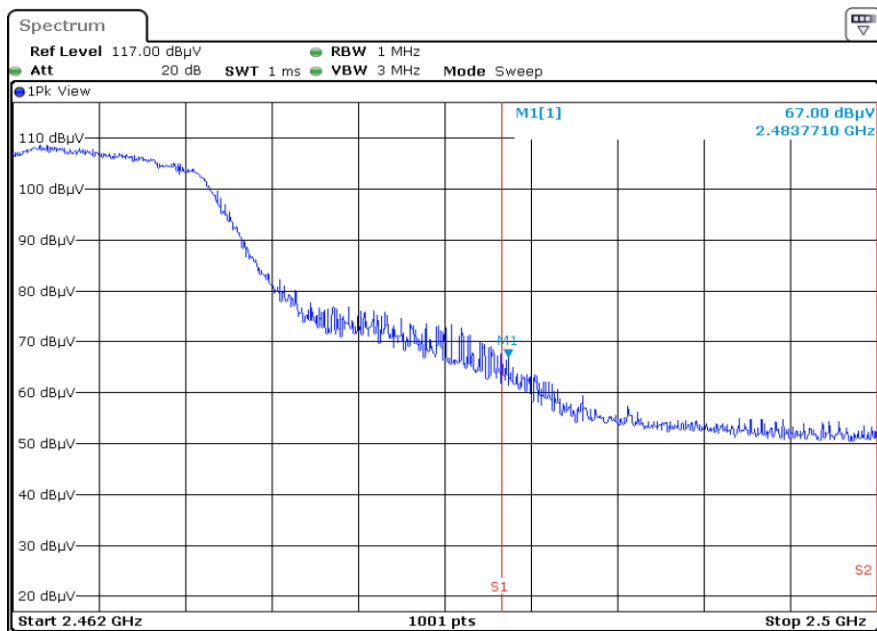
2462.0 F3 RestrictedBand Horizontal PEAK
