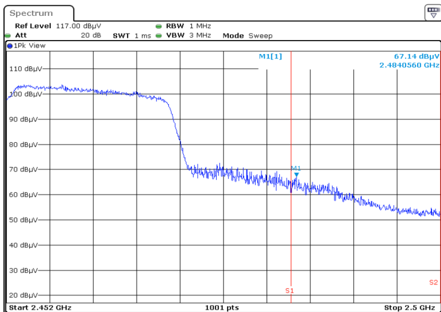
2452.0 F3 RestrictedBand Vertical PEAK
