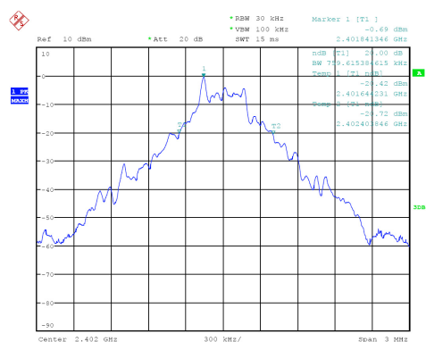
GFSK Mode 2402MHz
