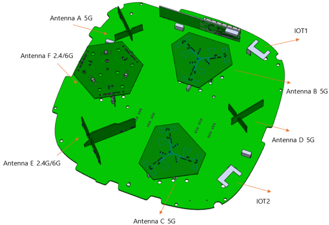
Fig. 1. Antenna Locations on the Antenna Support Board
