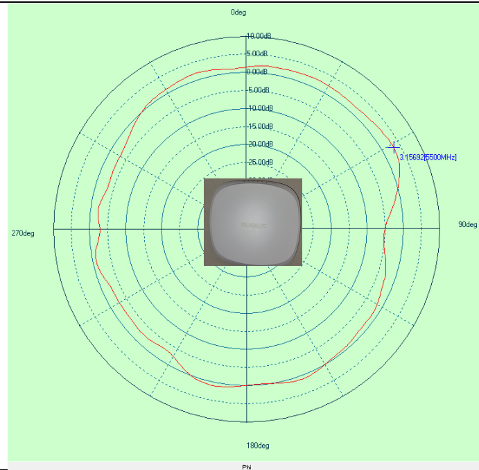
Antennas B and C, 5 GHz horizontal Max gain 3.2 dBi in 5.5 GHz UNII-2 band
