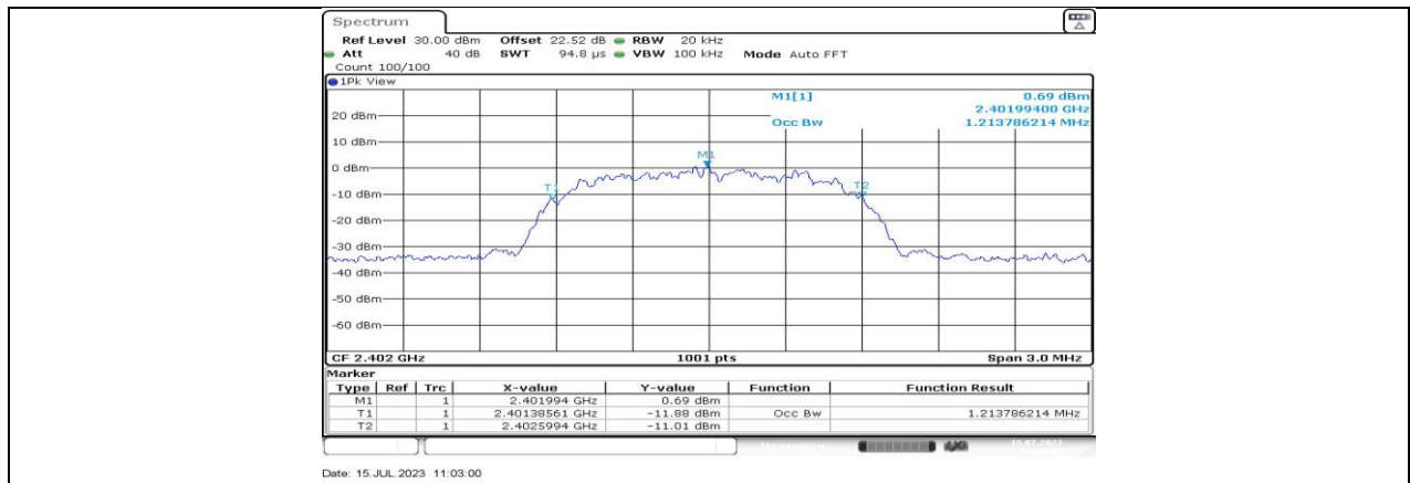
3DH5 Ant1_2402
