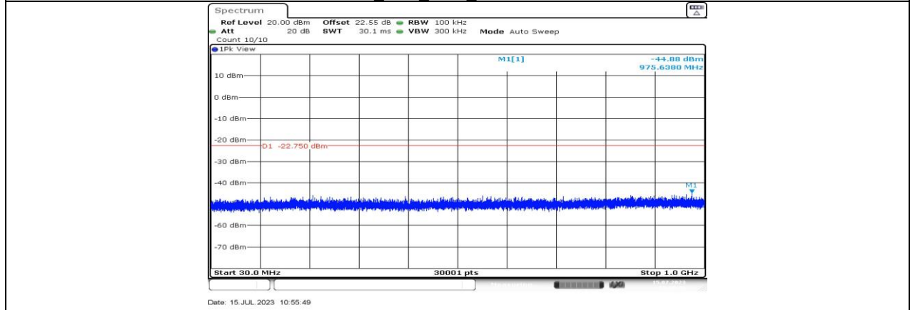
DH5_Ant1_2441_30~1000
