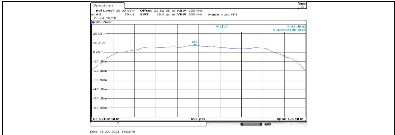
3DH5_Ant1_2402_0~Reference
