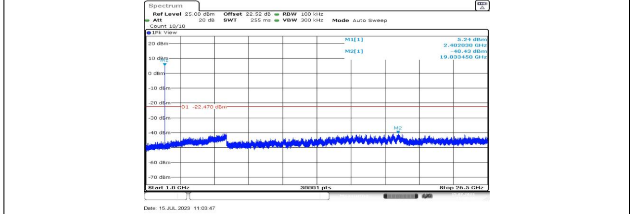
3DH5_Ant1_2402_1000~26500
