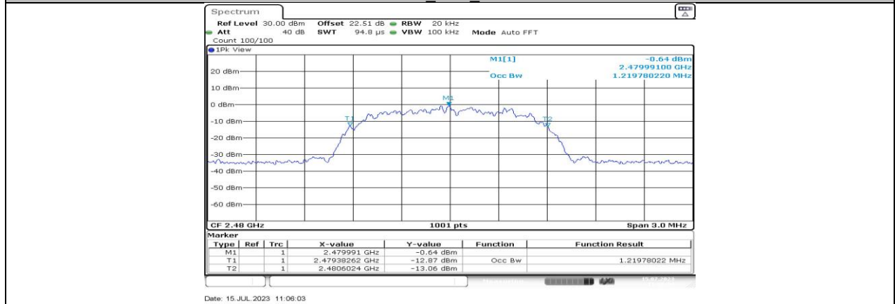
3DH5 Ant1_2480
