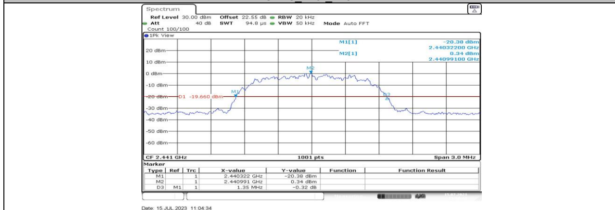
3DH5 Ant1_2441
