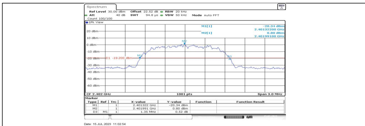
3DH5 Ant1_2402
