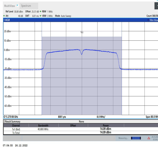
11AC40MIMO-Ant2-5270-TPC L-----13.40-85.37-0.69
