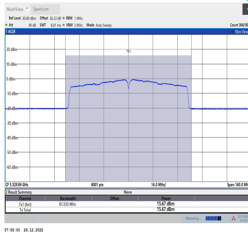
11AC80MIMO-Ant1-5530-TPC L-----14.48-76.00-1.19
