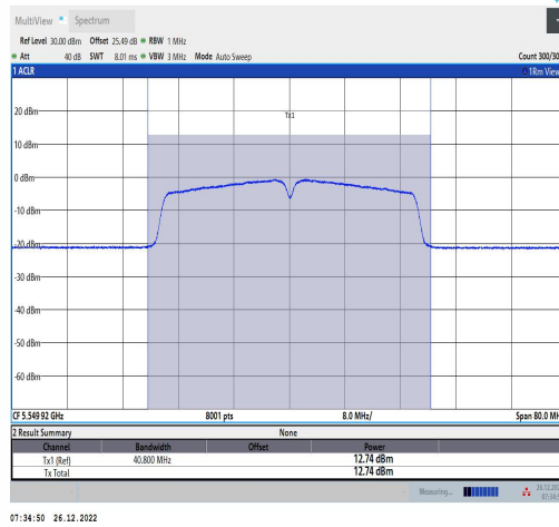
11AC40MIMO-Ant2-5550-TPC L-----12.05-85.37-0.69
