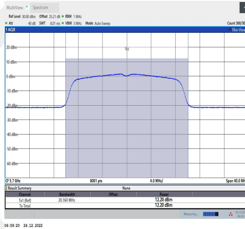
11AC20MIMO-Ant2-5700-TPC L-----11.90-93.24-0.30
