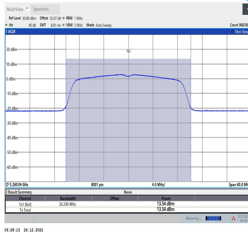
11AC20MIMO-Ant1-5260-TPC L-----13.17-91.89-0.37
