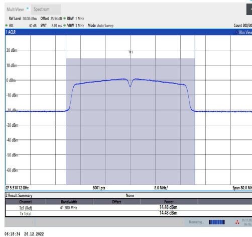
11N40MIMO-Ant1-5510-TPC L-----14.09-91.43-0.39
