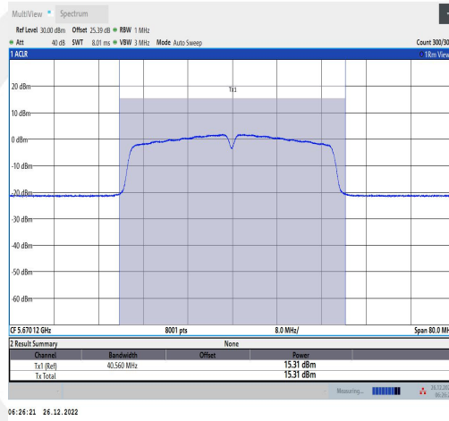
11N40MIMO-Ant2-5670-TPC L-----14.92-91.43-0.39
