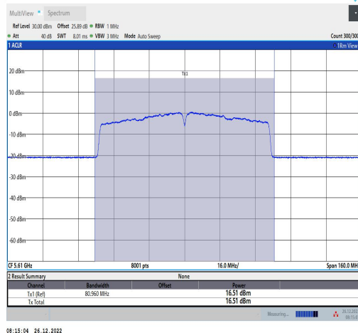
11AC80MIMO-Ant2-5610-TPC L-----15.32-76.00-1.19
