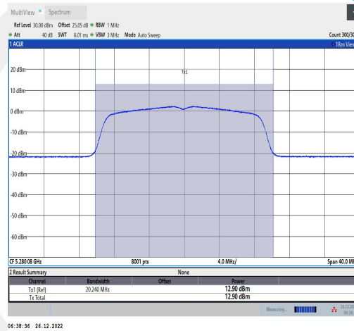
11AC20MIMO-Ant1-5280-TPC L-----12.60-93.24-0.30
