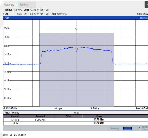
11AC80MIMO-Ant2-5290-TPC L-----13.69-79.17-1.01
