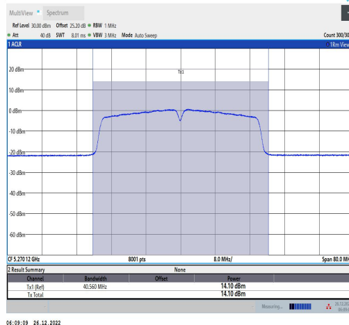
11N40MIMO-Ant2-5270-TPC L-----13.78-92.86-0.32
