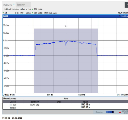
11AC80MIMO-Ant2-5530-TPC L-----14.43-76.00-1.19
