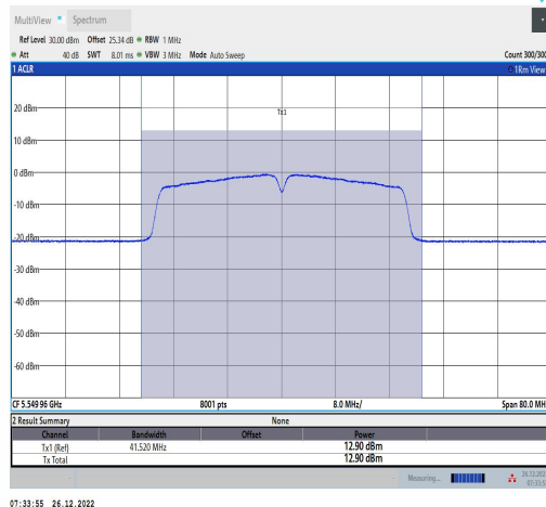
11AC40MIMO-Ant1-5550-TPC L-----12.32-87.50-0.58
