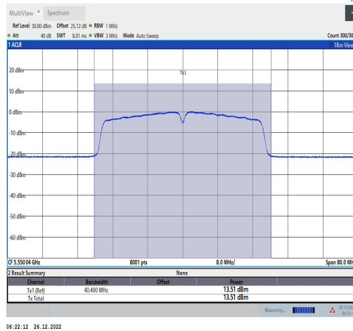
11N40MIMO-Ant2-5550-TPC L-----13.19-92.86-0.32
