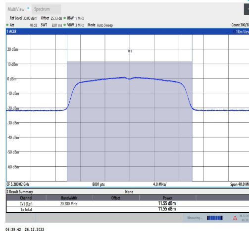
11AC20MIMO-Ant2-5280-TPC L-----11.18-91.89-0.37
