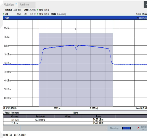
11N40MIMO-Ant2-5310-TPC L-----13.83-91.55-0.38
