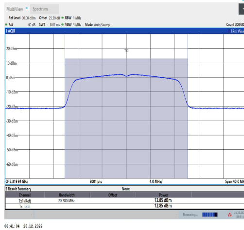
11AC20MIMO-Ant1-5320-TPC L-----12.48-91.89-0.37
