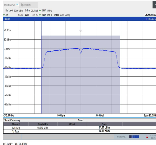
11AC40MIMO-Ant2-5670-TPC L-----13.53-87.50-0.58
