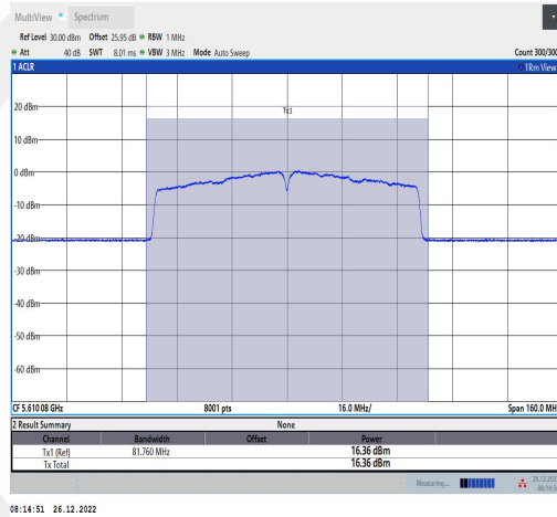
11AC80MIMO-Ant1-5610-TPC L-----15.17-76.00-1.19
