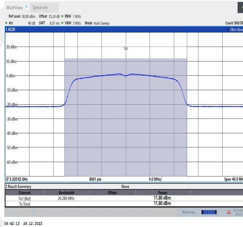
11AC20MIMO-Ant2-5320-TPC L-----11.43-91.89-0.37
