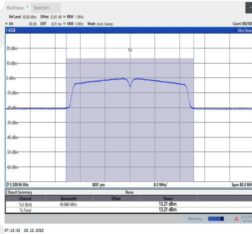
11AC40MIMO-Ant2-5510-TPC L-----12.63-87.50-0.58
