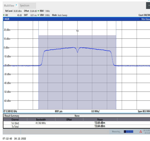
11AC40MIMO-Ant1-5510-TPC L-----12.95-85.37-0.69
