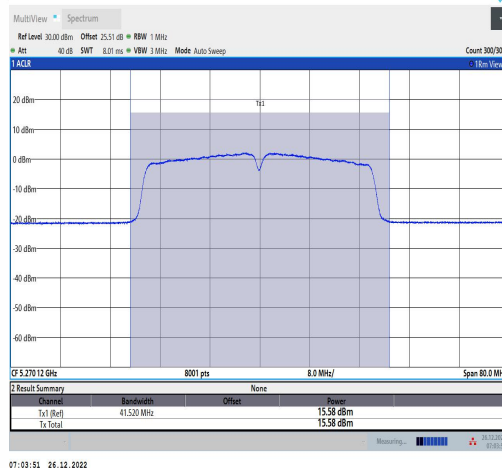
11AC40MIMO-Ant1-5270-TPC L-----14.89-85.37-0.69
