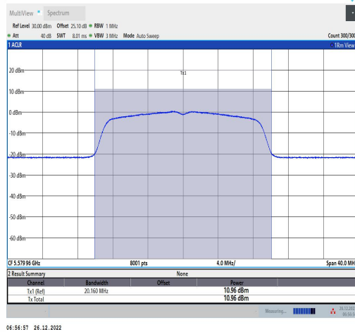
11AC20MIMO-Ant2-5580-TPC L-----10.59-91.89-0.37
