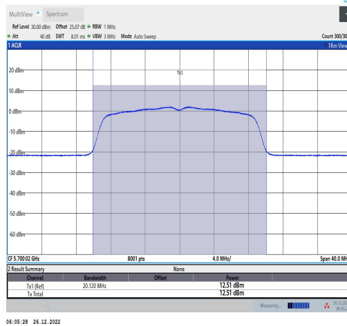
11N20MIMO-Ant2-5700-TPC L-----12.35-96.32-0.16
