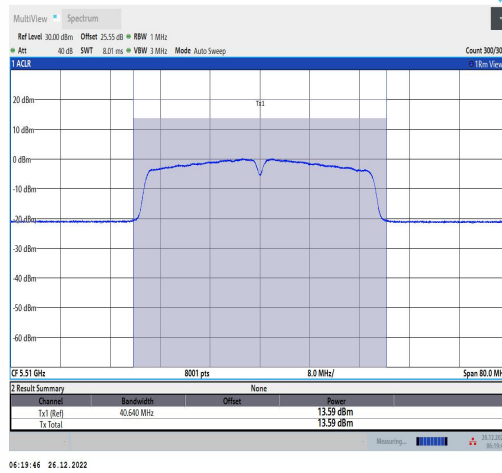
11N40MIMO-Ant2-5510-TPC L-----13.27-92.86-0.32
