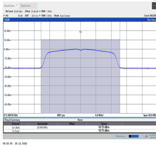
11AC20MIMO-Ant2-5500-TPC L-----10.38-91.89-0.37
