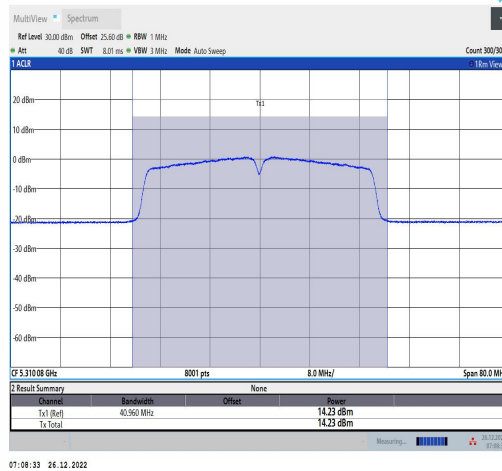
11AC40MIMO-Ant2-5310-TPC L-----13.54-85.37-0.69
