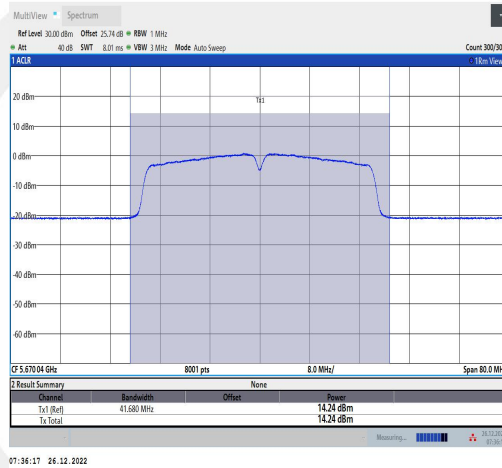
11AC40MIMO-Ant1-5670-TPC L-----13.55-85.37-0.69
