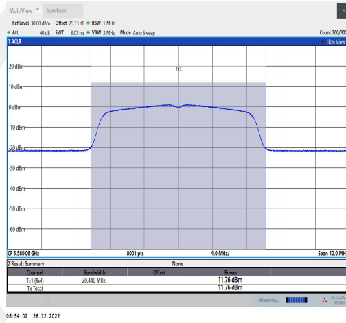
11AC20MIMO-Ant1-5580-TPC L-----11.39-91.89-0.37
