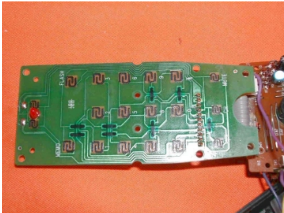
Handset PCB keypad front side
