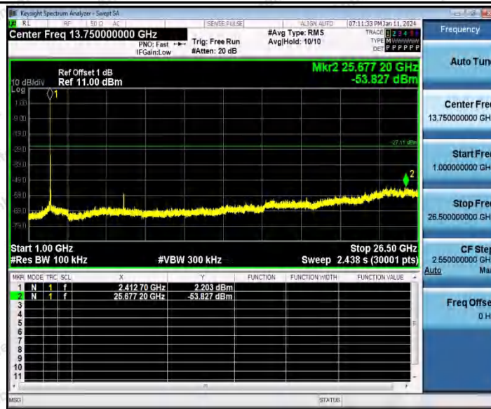
11B_Ant2_2412_0~Reference
