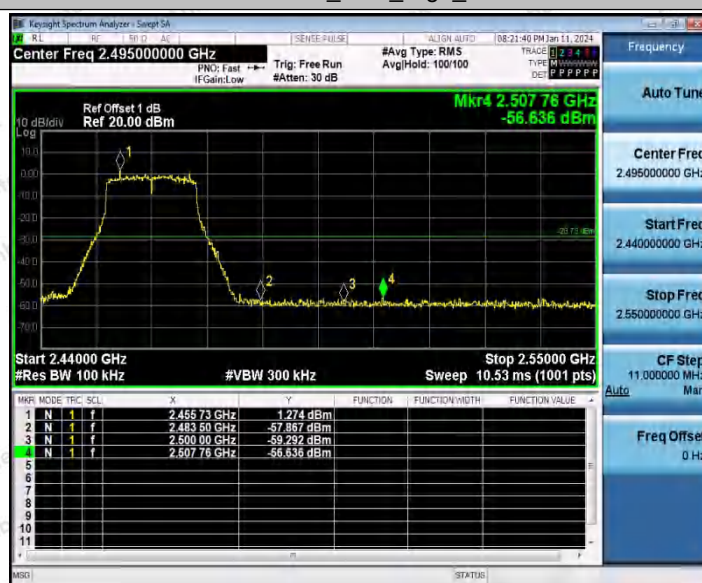
11N20SISO_Ant2_High_2462
