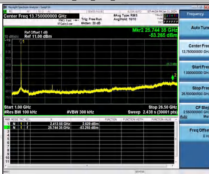
11G_Ant2_2412_0~Reference
