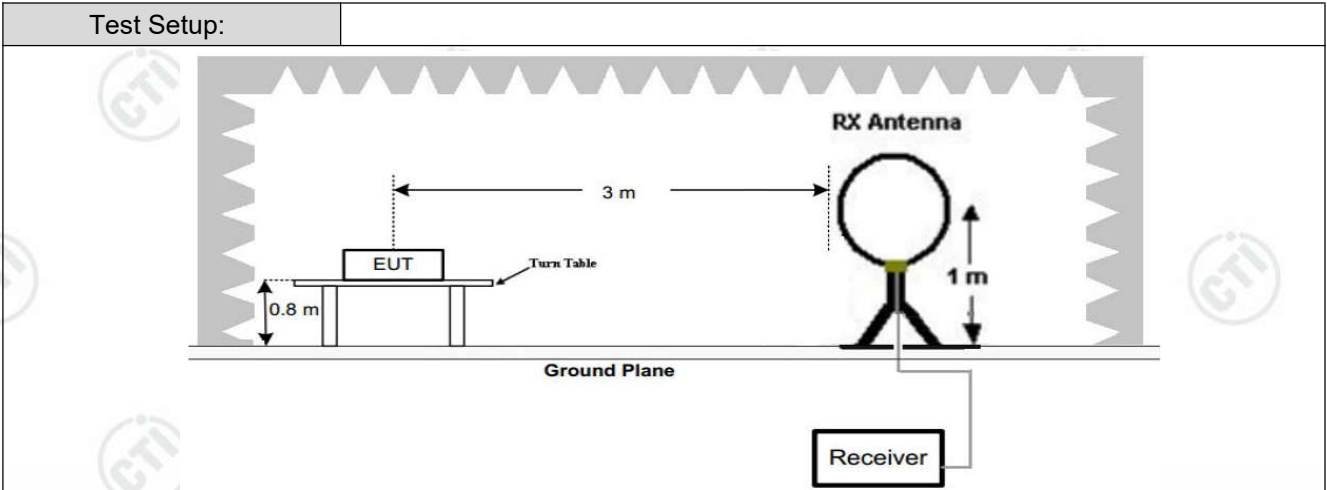
Figure 1. Below 30MHz
