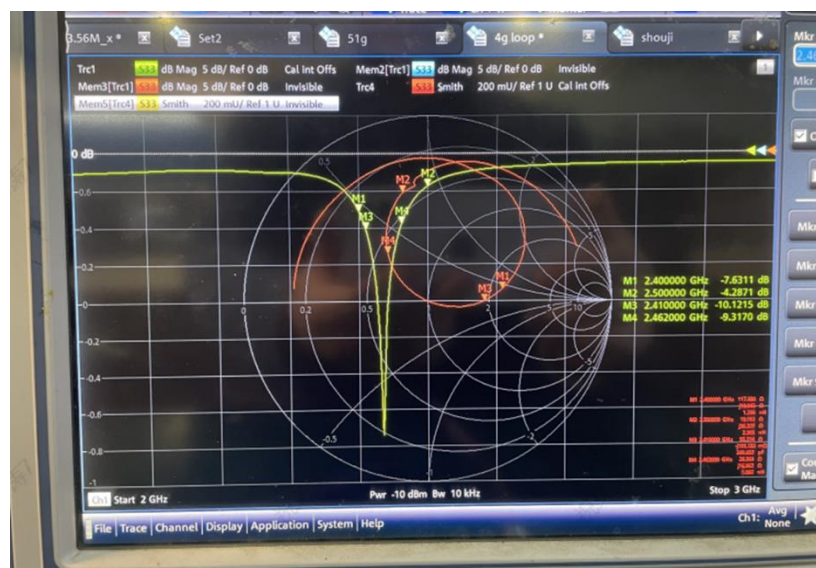
Figure 4.Return Loss
