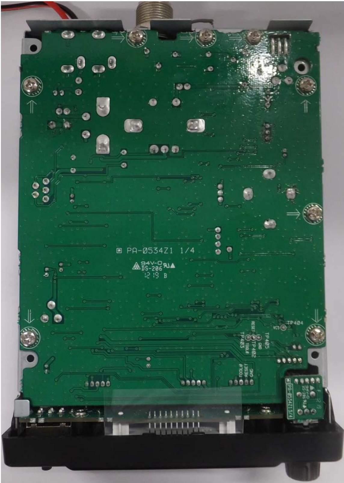
Figure E20.4 – Internal Photo – Main PCB Bottom Side
