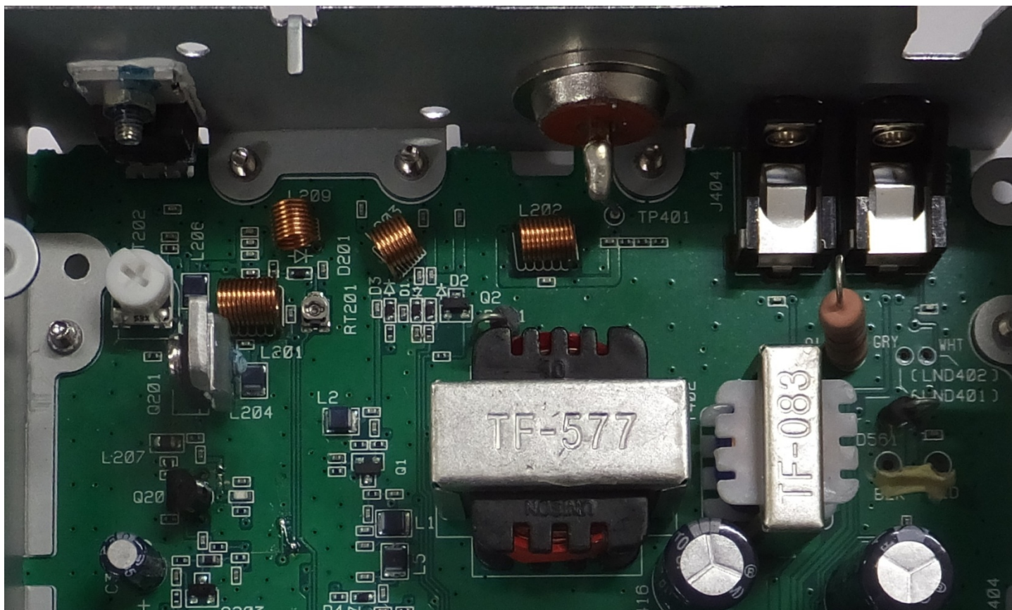
Figure E20.8 – Internal Photo – Main PCB Component Side – RF Section
