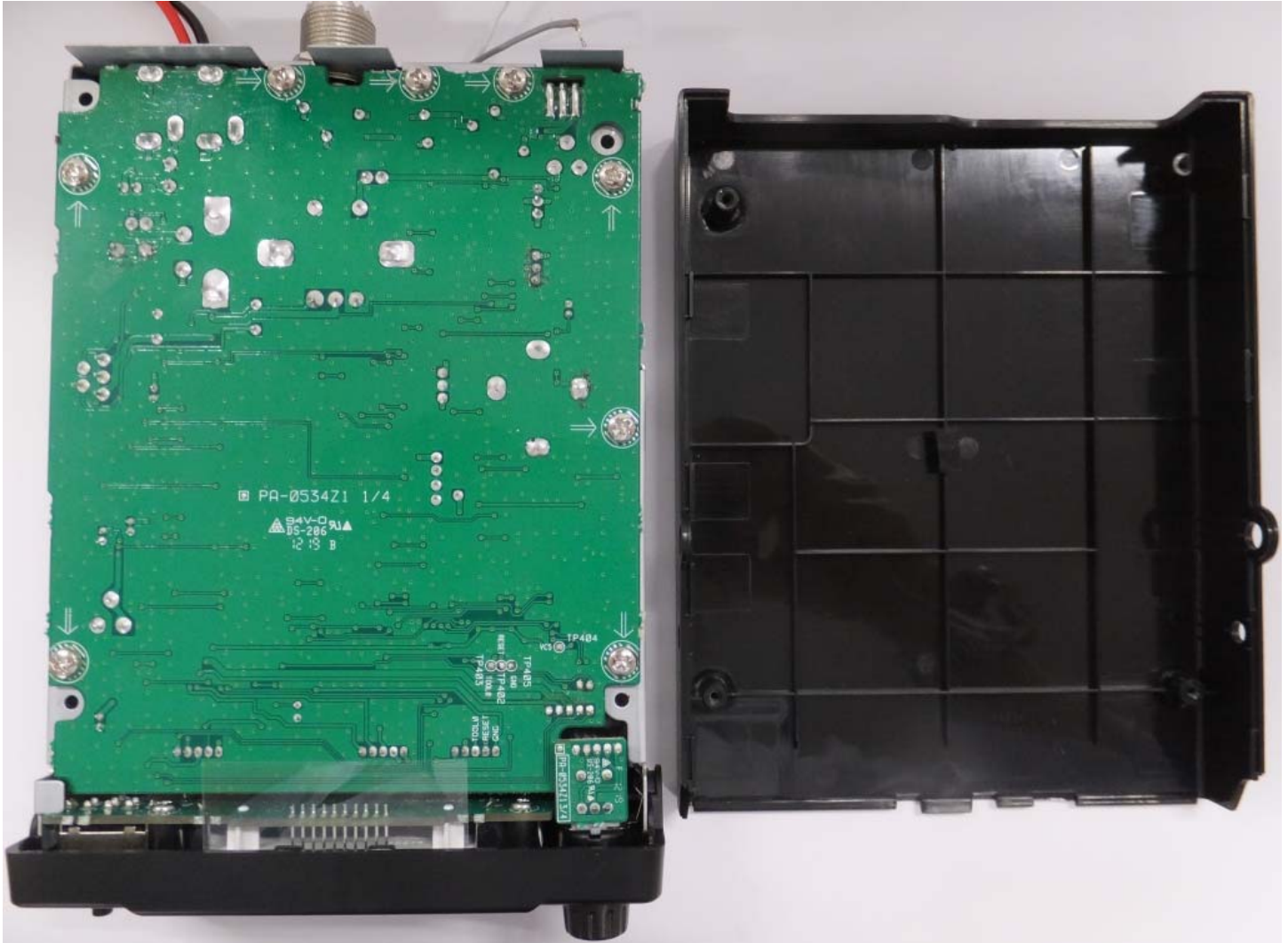
Figure E20.1 – Internal Photo – Top Cover Removed - PCB Bottom Side
