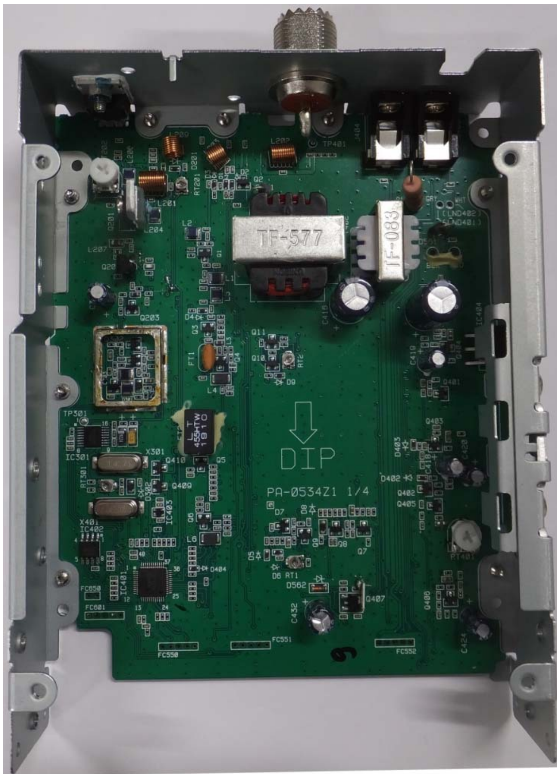
Figure E20.6 – Internal Photo – Main PCB Component Side – Shield Removed
