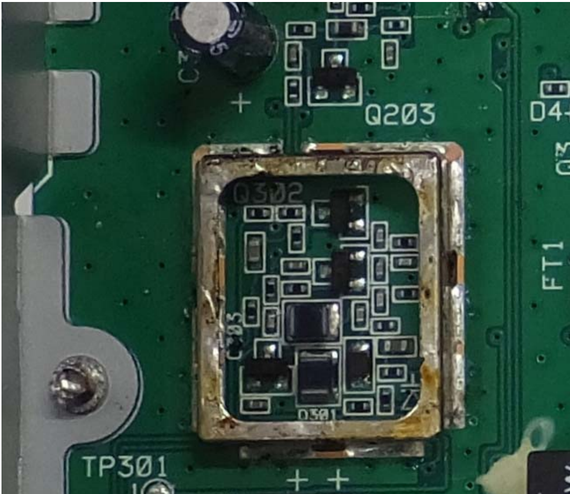
Figure E20.7 – Internal Photo – Main PCB Component Side - Shield Removed (Zoomed)
