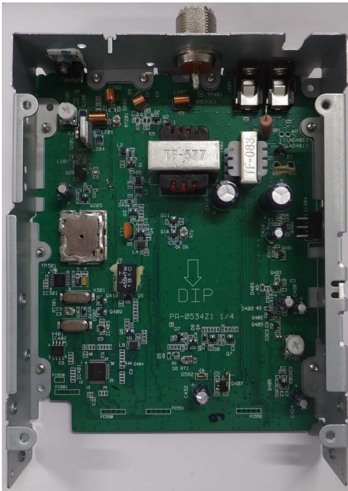
Figure E20.5 – Internal Photo – Main PCB Component Side
