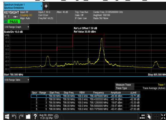
N14(5M)_DFT-s- OFDM_QPSK_Edge_1RB_Right_Mid_CH
