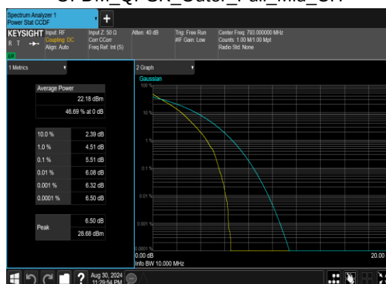
N14(10M)_DFT-s- OFDM_QPSK_Outer_Full_Mid_CH
