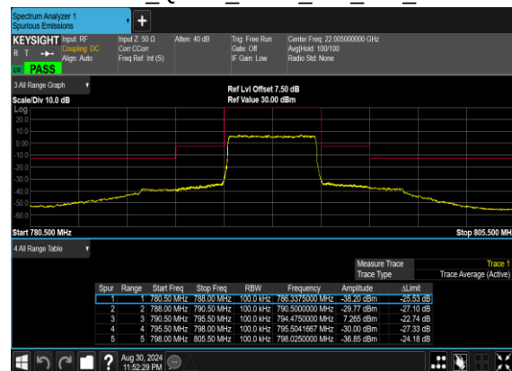
N14(5M)_DFT-s- OFDM_QPSK_Outer_Full_Mid_CH
