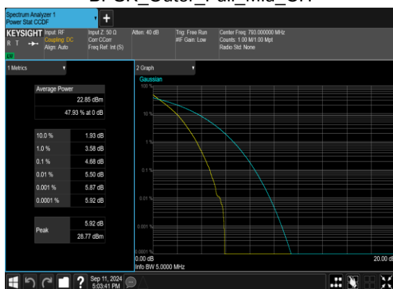
N14(5M)_DFT-s-OFDM_PI_2- BPSK_Outer_Full_Mid_CH
