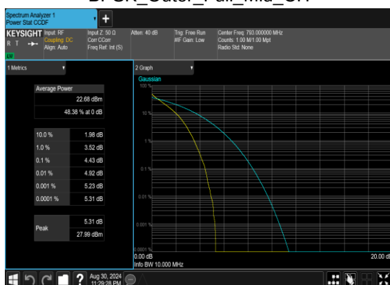
N14(10M)_DFT-s-OFDM_PI_2- BPSK_Outer_Full_Mid_CH
