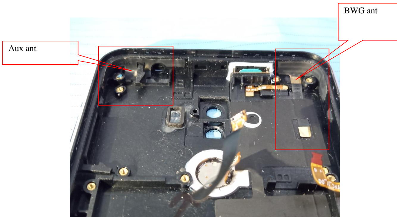
EUT –Antenna 1 View
