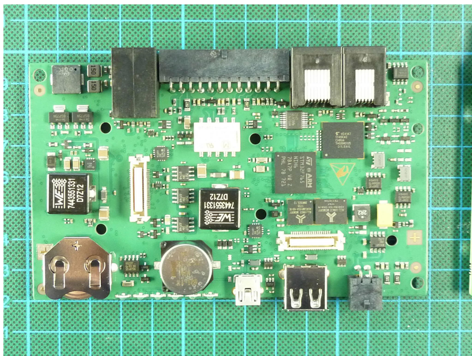
EUT main unit PCB A bottom view
