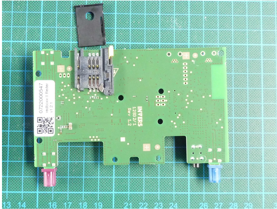
EUT main unit PCB B bottom view
