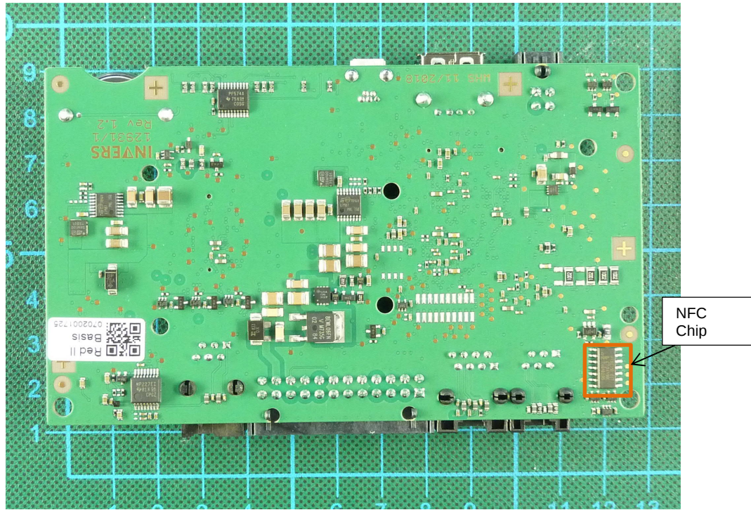
EUT main unit PCB A top view
