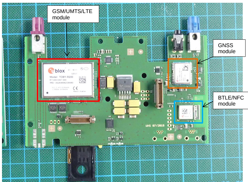
EUT main unit PCB B bottom view
