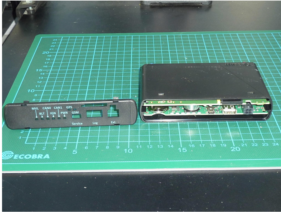
EUT main unit inside view 1
