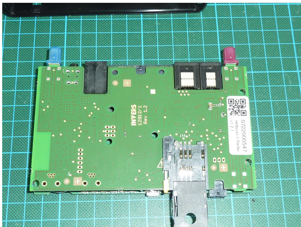
EUT main unit PCB's view 1
