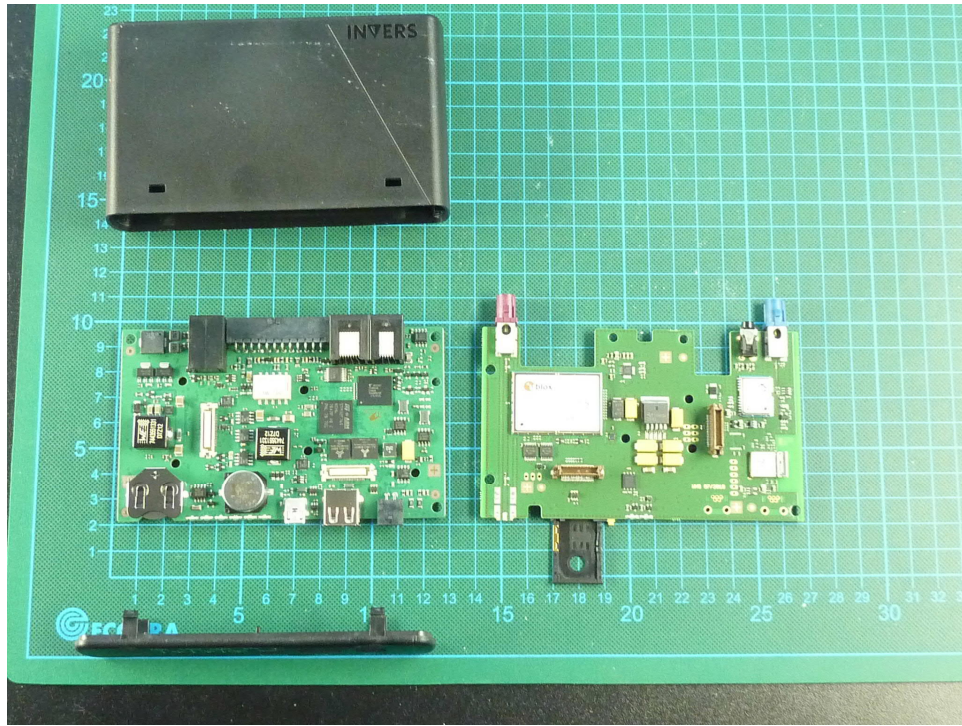
EUT main unit inside view 3
