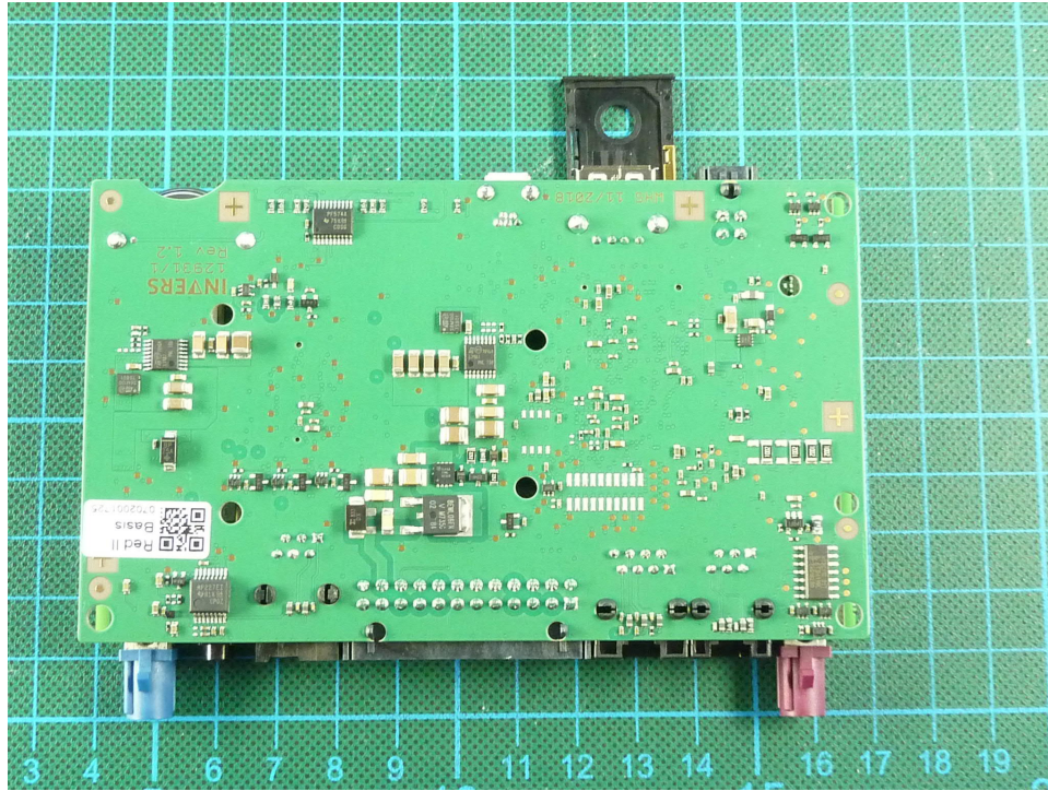
EUT main unit PCB's view 2
