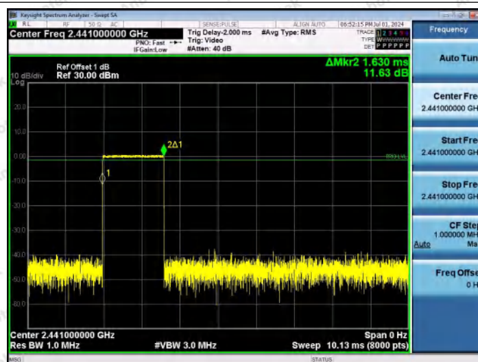
DH3-Ant1-Hop-PASS
