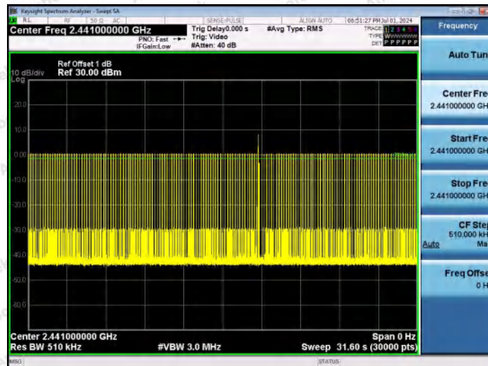
DH1-Ant1-Hop-PASS
