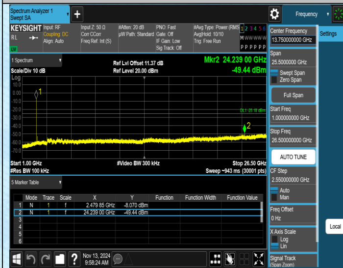
3DH5-Ant1-2480-1000~26500-PASS
