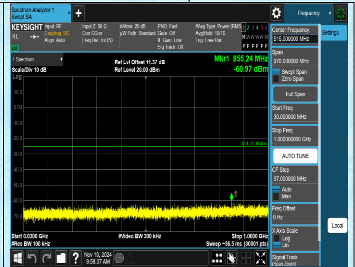
3DH5-Ant1-2480-30~1000-PASS
