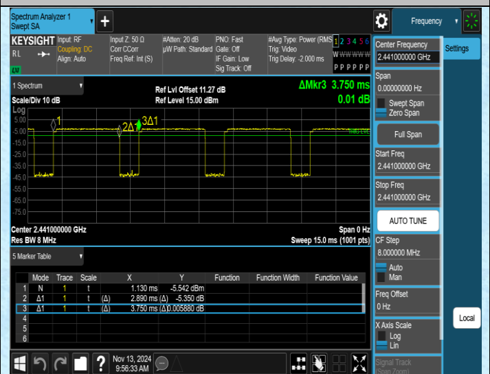
NTNV-3DH5-Ant1-2441
