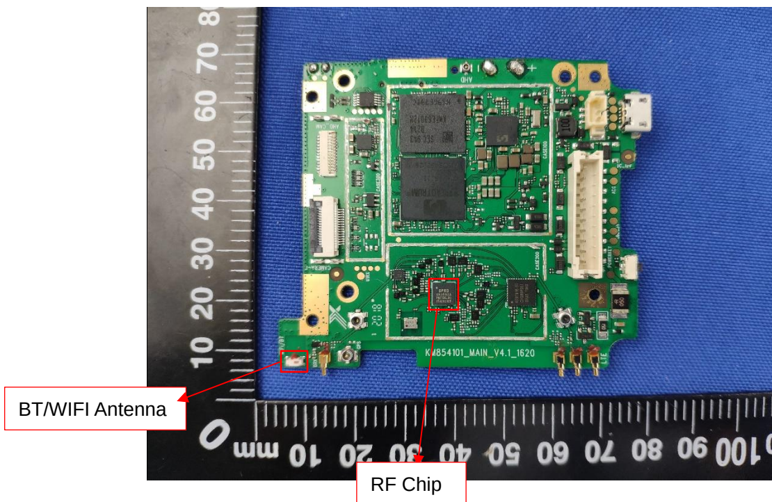
MAIN BOARD TOP VIEW (WITHOUT SHIELDING)
