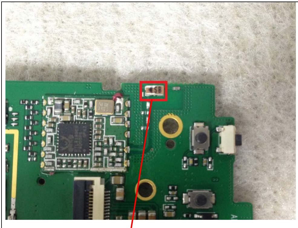
Chip Antenna
