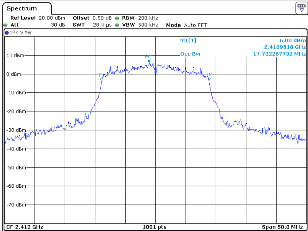
802.11 HT20_Low Channel
