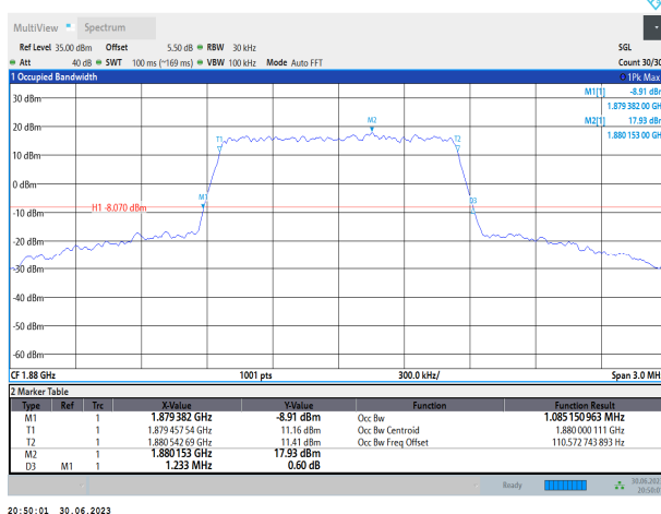
Band2-1.4MHz-QPSK-18900-6RB#0
