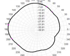
Total(H+V), Max: -1.62dB, Crd=13.29
