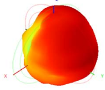
2490.0MHz H+V, ER: 41.4%
