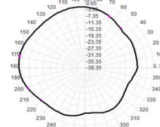
Total(H+V), Max: -1.32dB, Crd=11.26
