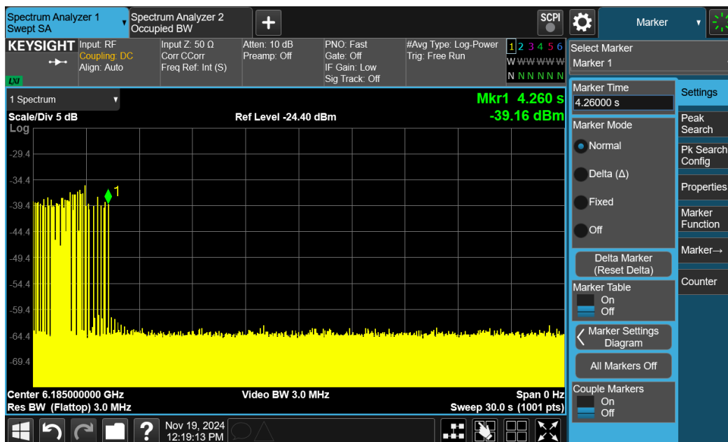
Plot 6: AWGN Signal Detection Upper Edge 160MHz
