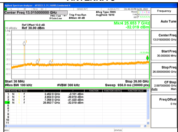
OUT-OF-BAND HIGH CHANNEL 9 ANTENNA 3
