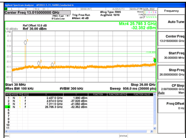
OUT-OF-BAND MID CHANNEL 6 ANTENNA 3
