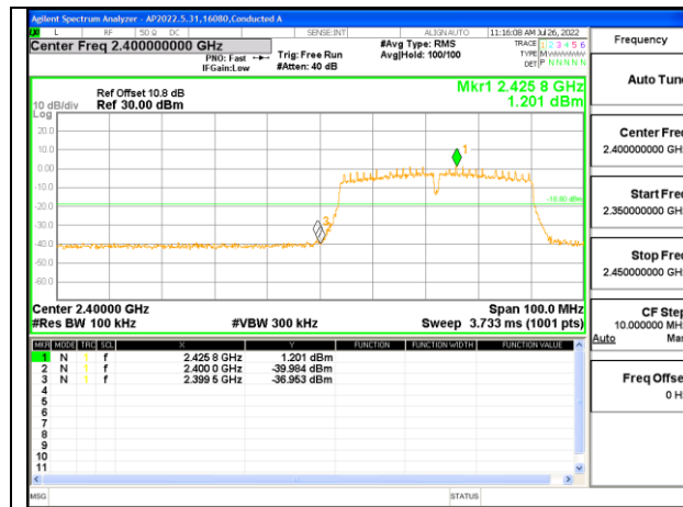
LOW CHANNEL 3 BANDEDGE ANTENNA 2
