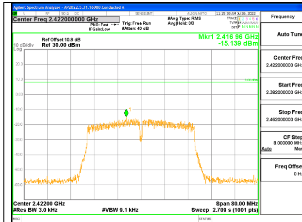
LOW CHANNEL 3 ANTENNA 2
