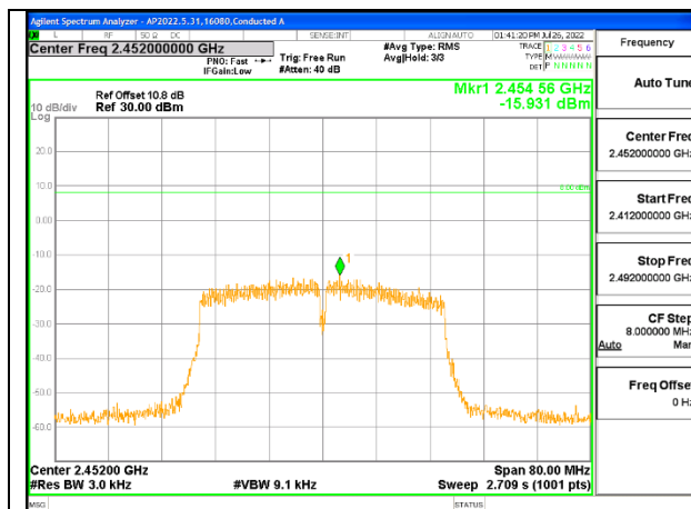
HIGH CHANNEL 9 ANTENNA 2
