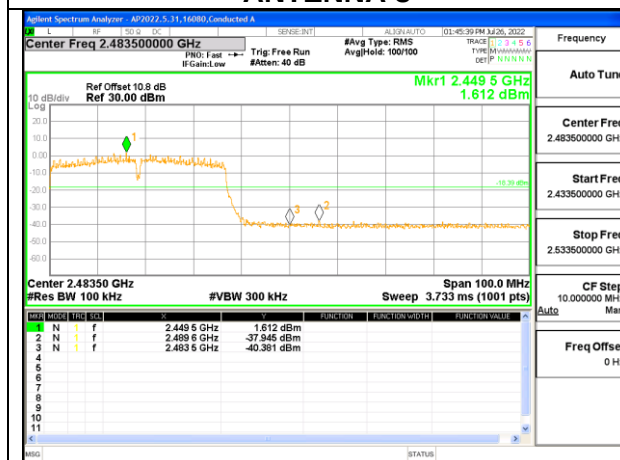
HIGH CHANNEL 9 BANDEDGE ANTENNA 3
