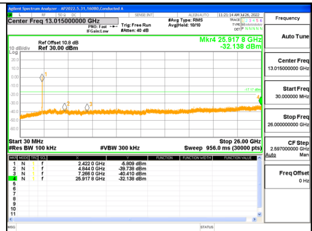
OUT-OF-BAND LOW CHANNEL 3 ANTENNA 3
