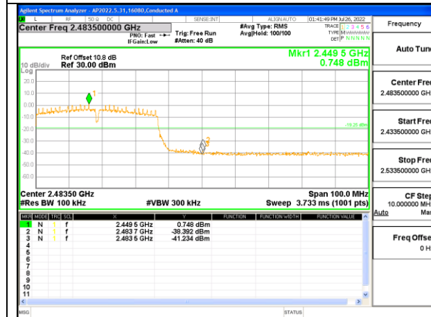
HIGH CHANNEL 9 BANDEDGE ANTENNA 2
