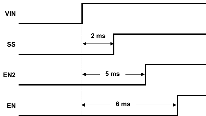
Figure 6-3. Nominal Start-Up Sequence Using SPI With SS (MCU Controls EN2)
