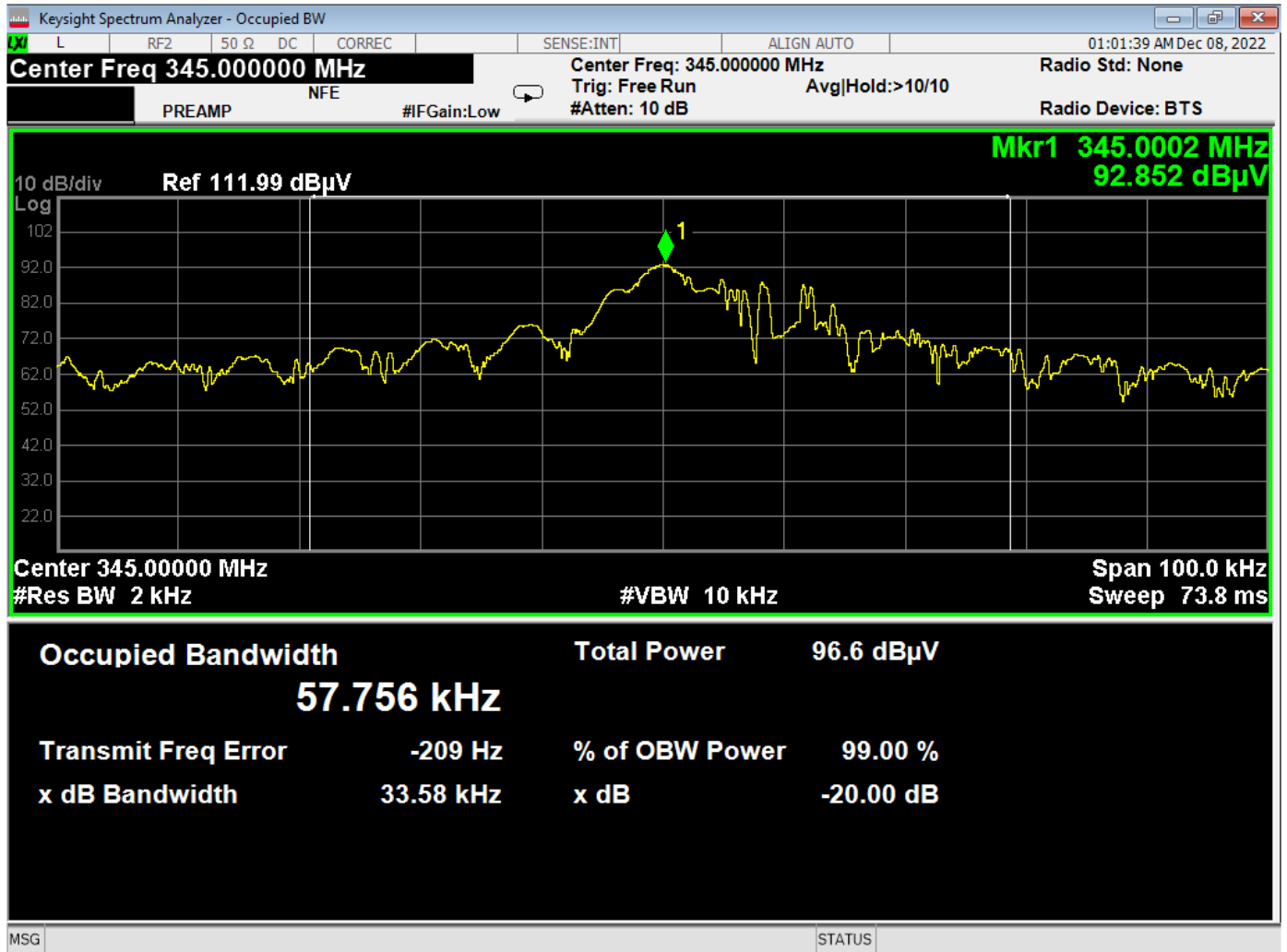
99% Bandwidth Plot – With External Sensor Adapter
