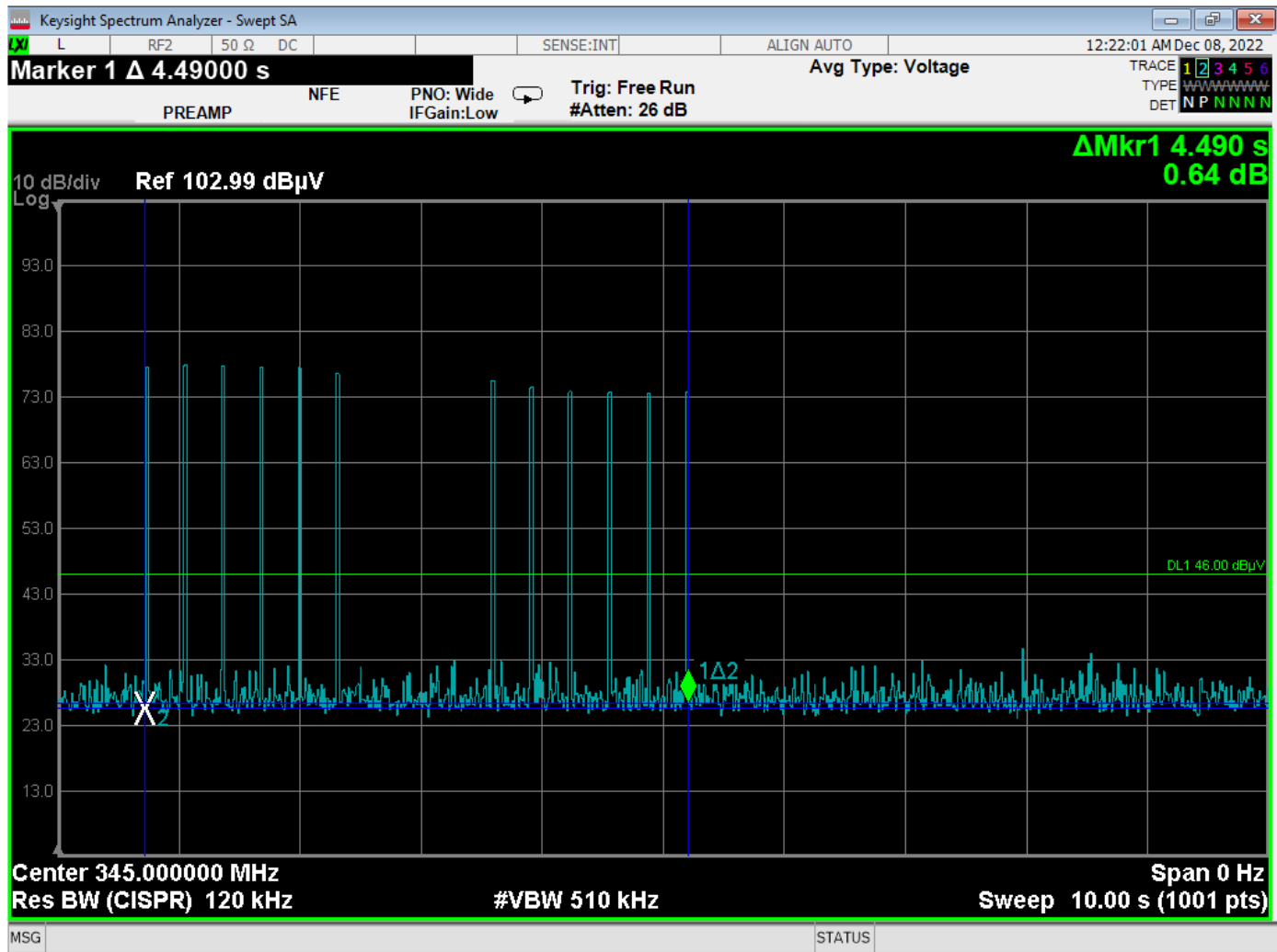
Plot Showing Actual Time of Transmission 4.49 seconds
