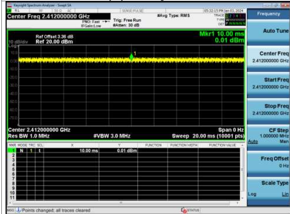
Duty Cycle NVNT g 2412MHz
