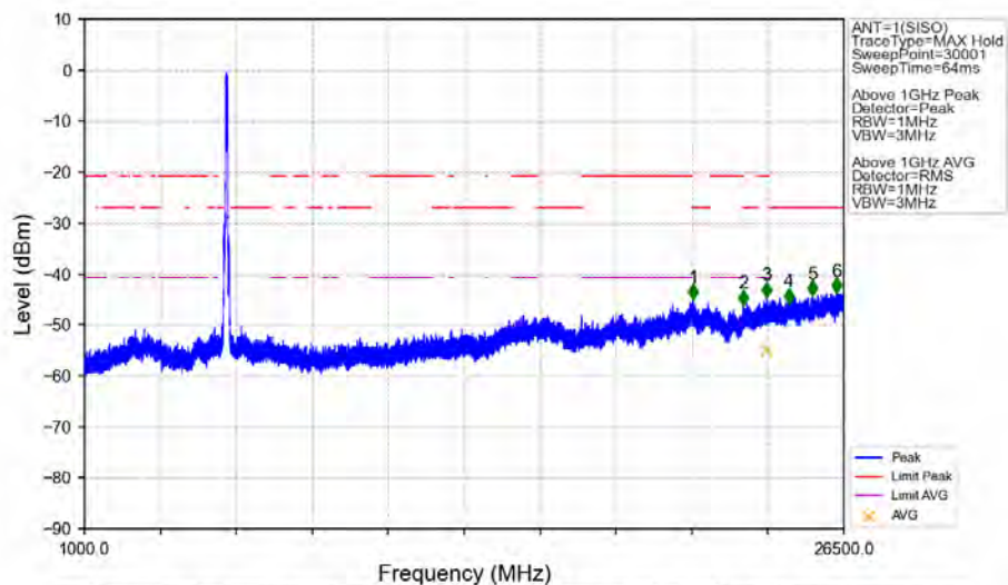
802.11ac(VHT80)_MCH_5775MHz_Ant1_NTNV
