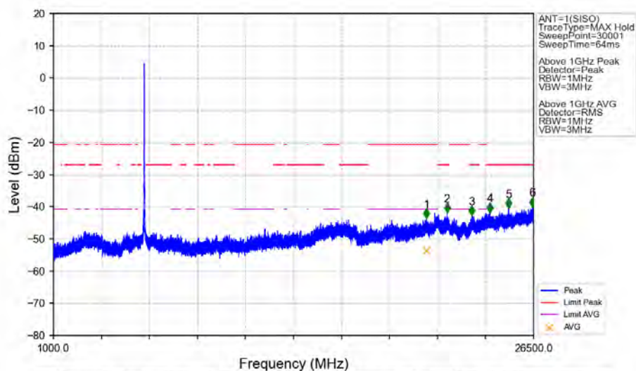
802.11ac(VHT20)_HCH_5825MHz_Ant1_NTNV
