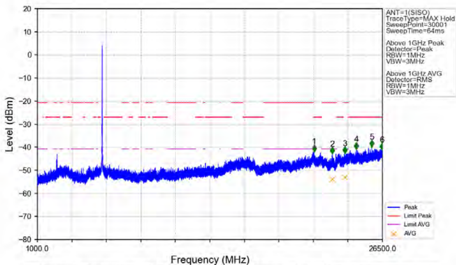
802.11ac(VHT20)_MCH_5785MHz_Ant1_NTNV
