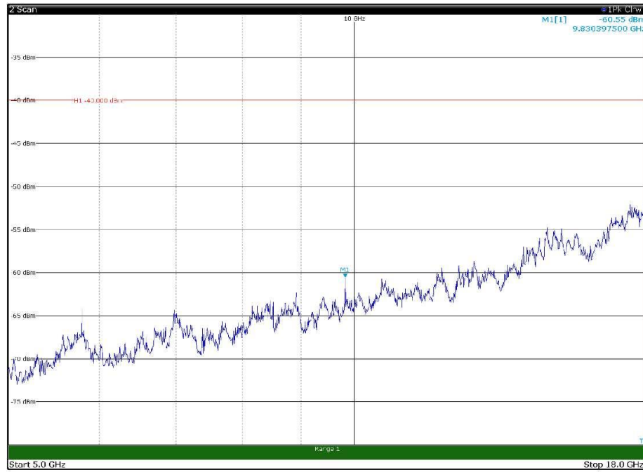
Channel: TOP, Modulation: 64QAM, BW=5MHz, Range: 5GHz - 18GHz, Polarization: Horizontal
