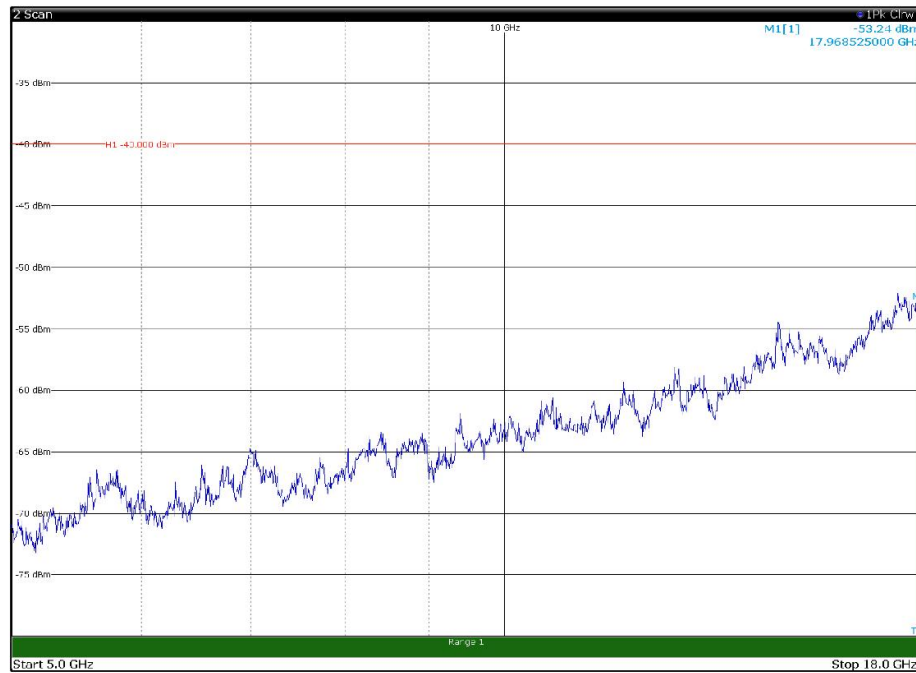
Channel: TOP, Modulation: 64QAM, BW=5MHz, Range: 5GHz - 18GHz, Polarization: Vertical
