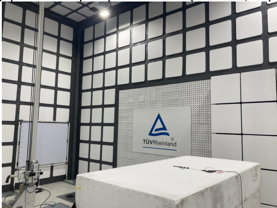
Photograph 70: Test Setup for Spurious Emissions (Back View 4, WiFi)
