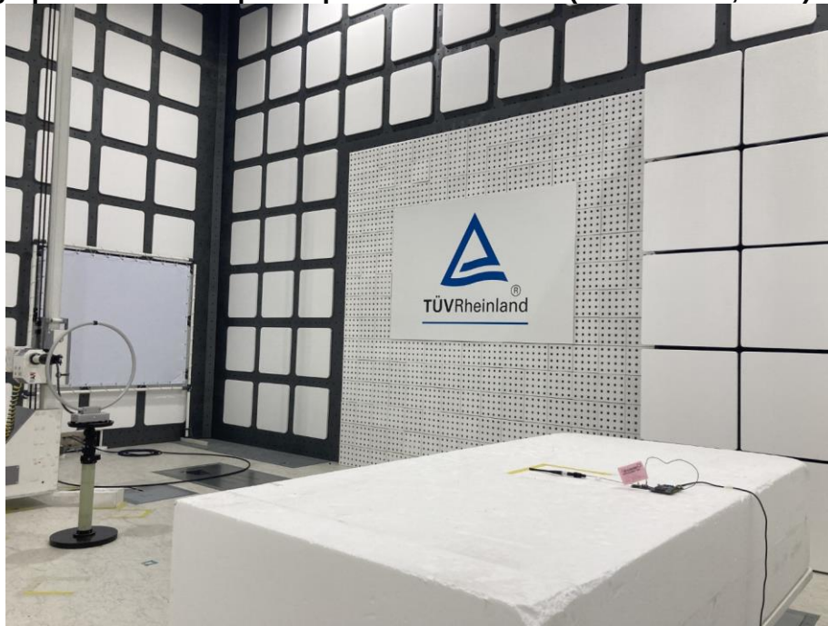
Photograph 68: Test Setup for Spurious Emissions (Back View 2, WiFi)
