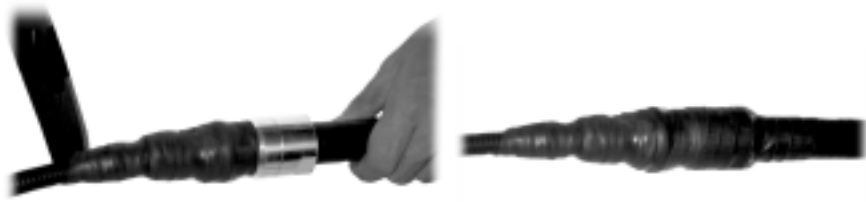
Fig. 8.6-11 Schematic Diagram of Wrapping Waterproof Adhesive Tape (2)
