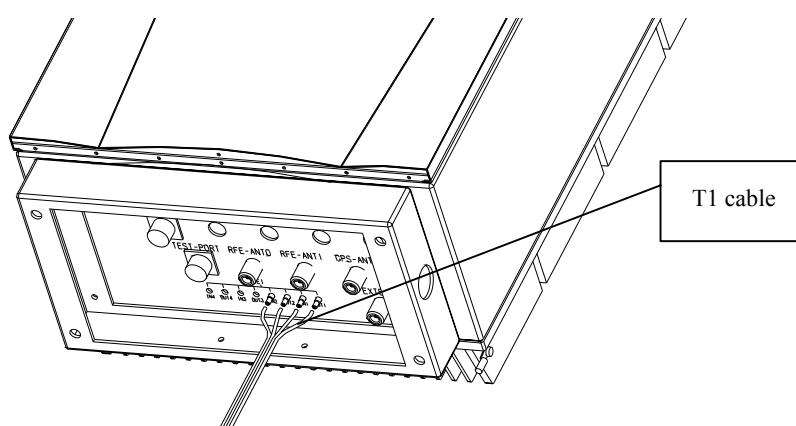
Fig. 7.2-7 Connection of T1 Cables
