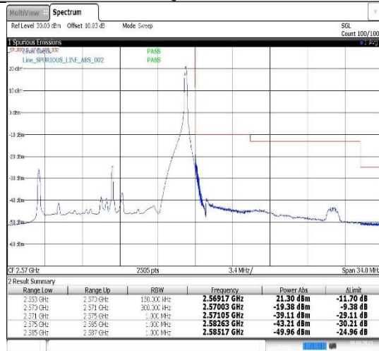
Band7-15MHz-QPSK-21375-1RB#74
