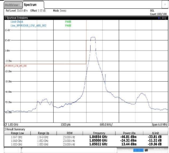
Band25-1.4MHz-QPSK-26047-1RB#0
