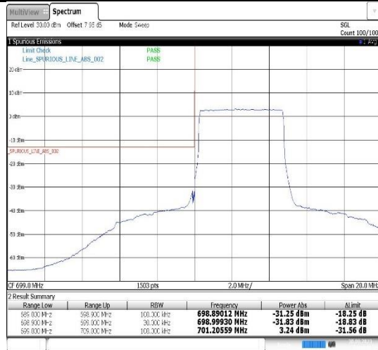
Band12-10MHz-QPSK-23060-50RB#0
