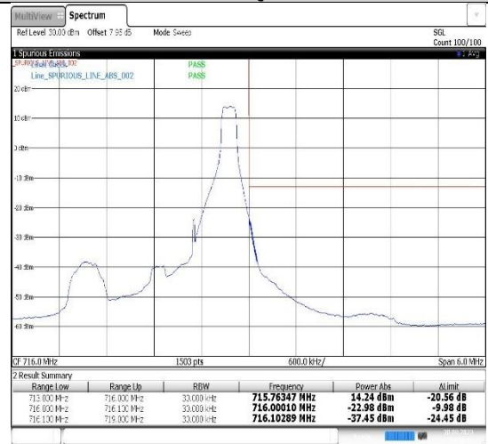
Band12-1.4MHz-16QAM-23173-1RB#5
