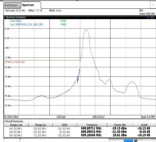
Band12-1.4MHz-QPSK-23017-1RB#0
