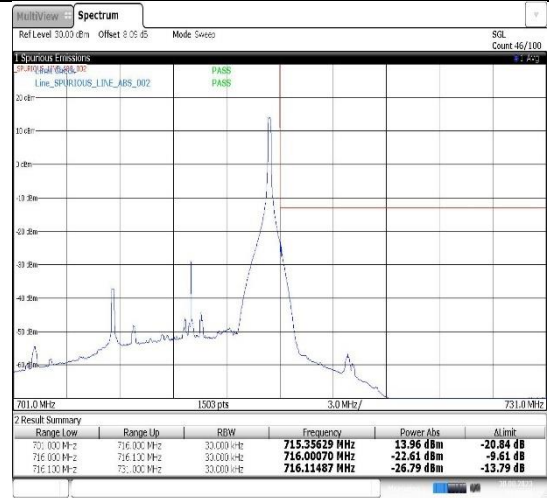
Band17-10MHz-16QAM-23800-1RB#49
