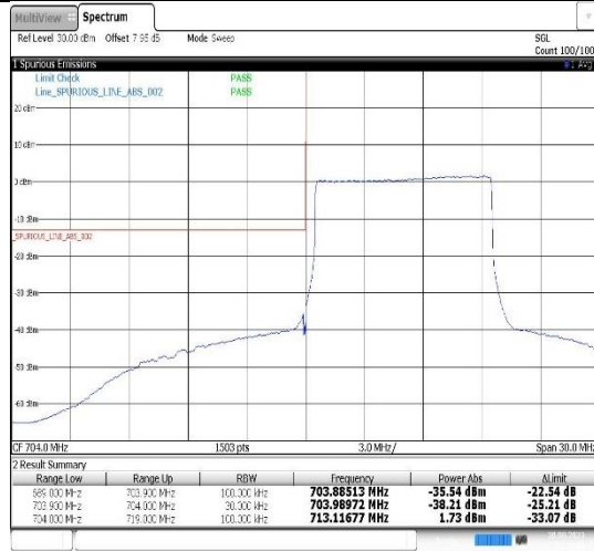
Band17-10MHz-16QAM-23780-50RB#0
