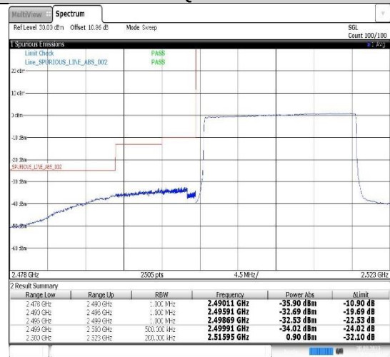
Band7-20MHz-16QAM-20850-100RB#0
