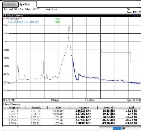
Band7-15MHz-QPSK-20825-1RB#0
