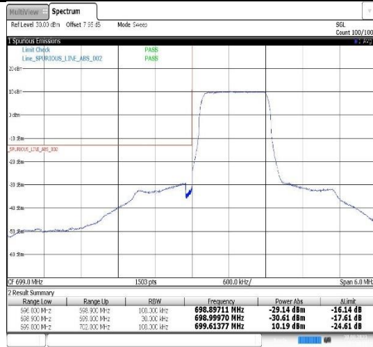
Band12-1.4MHz-QPSK-23173-6RB#0
