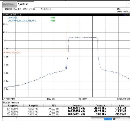
Band17-5MHz-16QAM-23755-25RB#0
