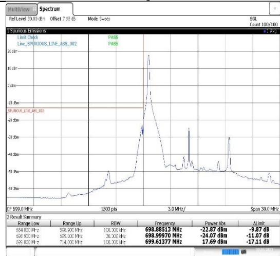
Band12-10MHz-16QAM-23060-1RB#0
