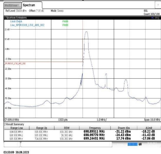
Band12-3MHz-16QAM-23165-1RB#14
