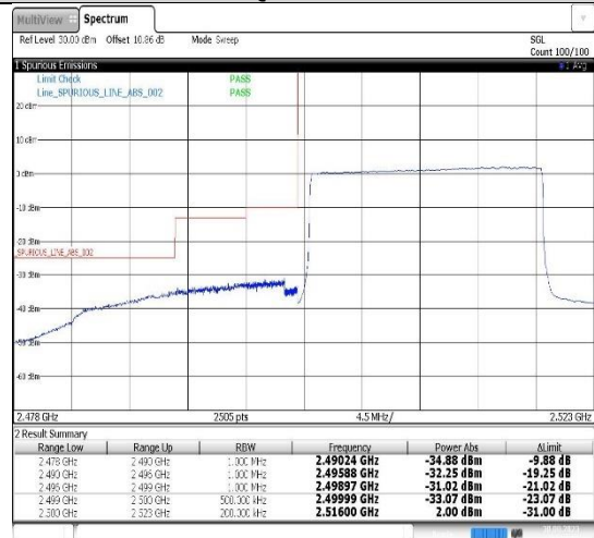
Band7-20MHz-QPSK-20850-100RB#0
