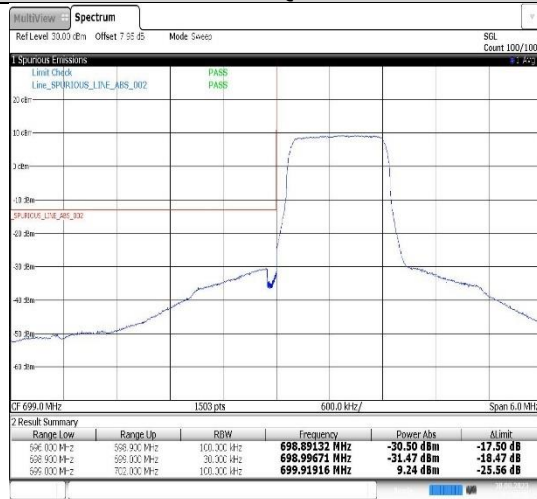
Band12-1.4MHz-16QAM-23017-6RB#0
