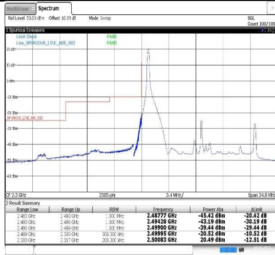
Band7-15MHz-16QAM-21375-1RB#74
