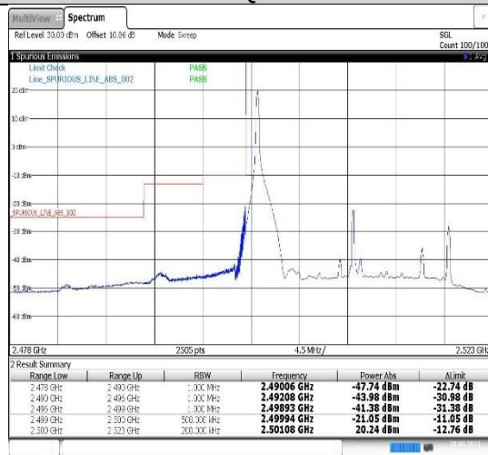
Band7-20MHz-16QAM-20850-1RB#0
