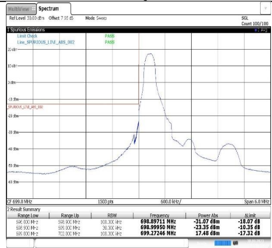
Band12-1.4MHz-16QAM-23017-1RB#0
