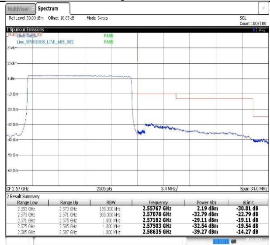
Band7-15MHz-QPSK-21375-75RB#0
