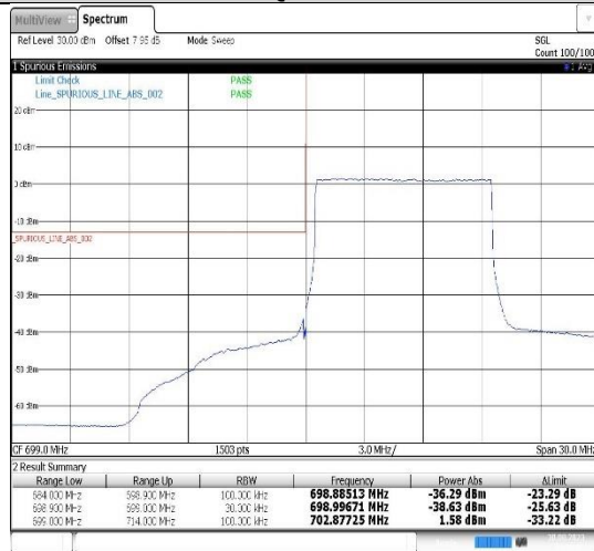
Band12-10MHz-QPSK-23060-50RB#0
