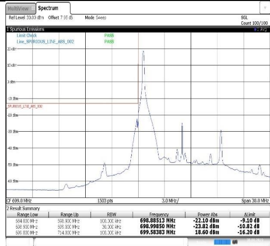
Band12-10MHz-16QAM-23060-1RB#0
