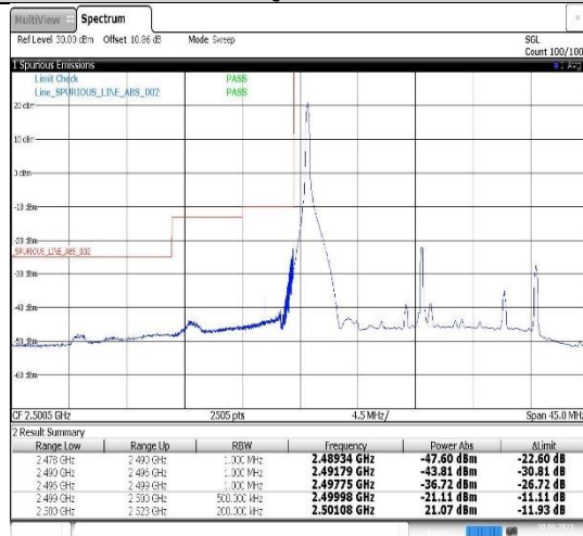
Band7-20MHz-QPSK-20850-1RB#0
