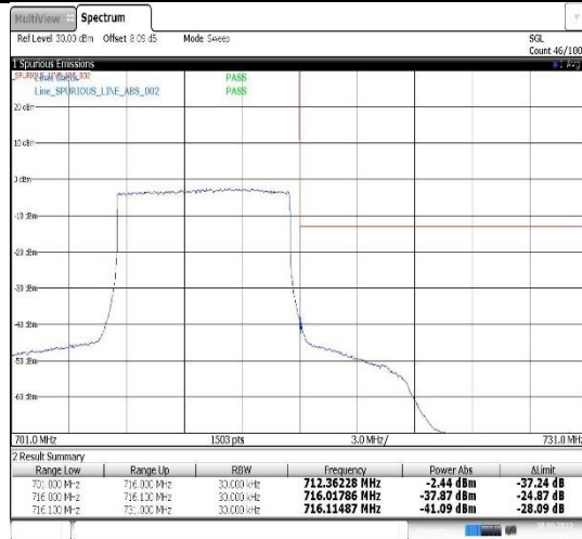
Band17-10MHz-16QAM-23780-50RB#0
