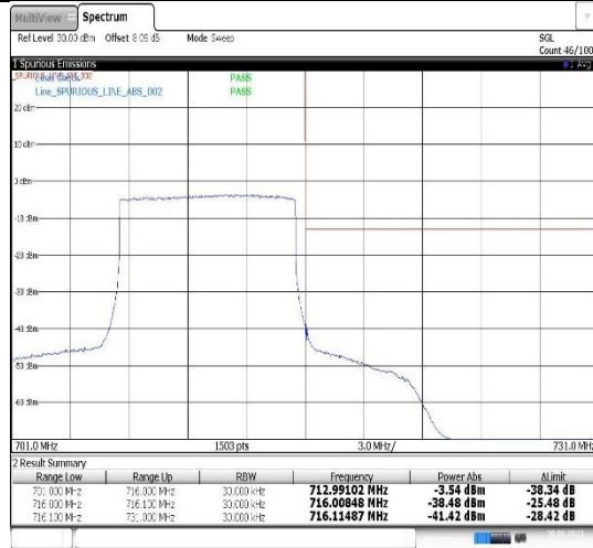
Band17-10MHz-16QAM-23800-50RB#0
