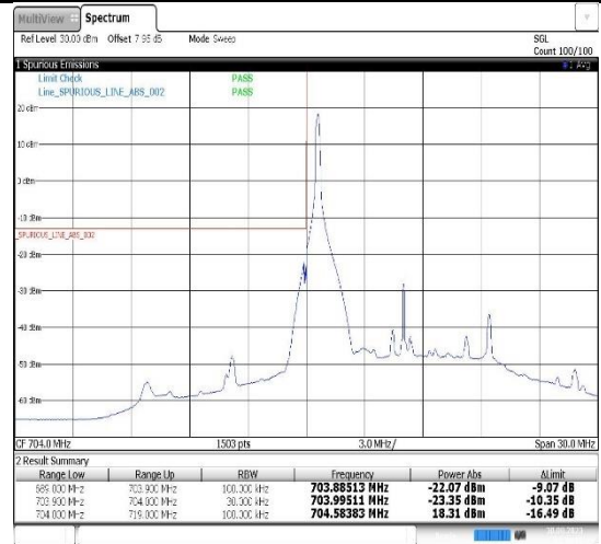
Band17-10MHz-16QAM-23800-1RB#49
