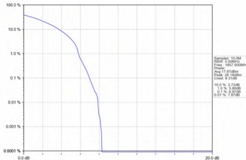
n25_15kHz_SISO_NTV_15MHz_DFT-s-OFDM_16_QAM_1857.5MHz_Outer_Full
