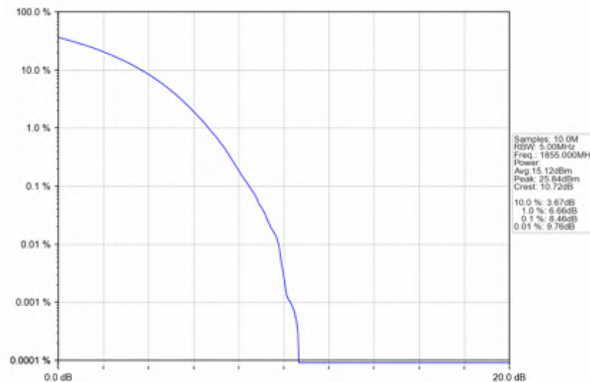
n25_15kHz_SISO_NTNV_10MHz_CP-OFDM 256 QAM_1855MHz_Outer_Full
