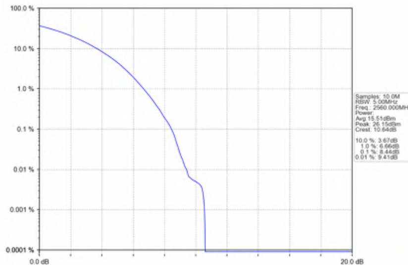
n7_30kHz_SISO_NTNV_20MHz_CP-OFDM 16 QAM_2560MHz_Outer_Full
