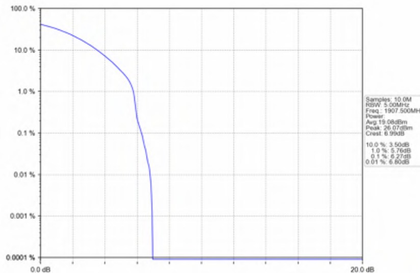
n25_15kHz_SISO_NTNV_15MHz_DFT-s-OFDM QPSK_1907.5MHz_Outer_Full
