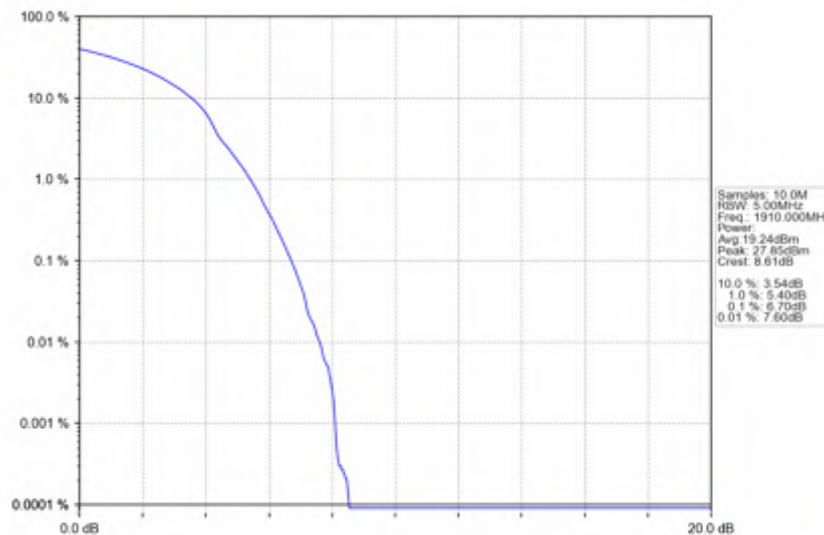
n25 30kHz SISO NTNv 10MHz DFT-s-OFDM 64 QAM 1910MHz Outer Full
