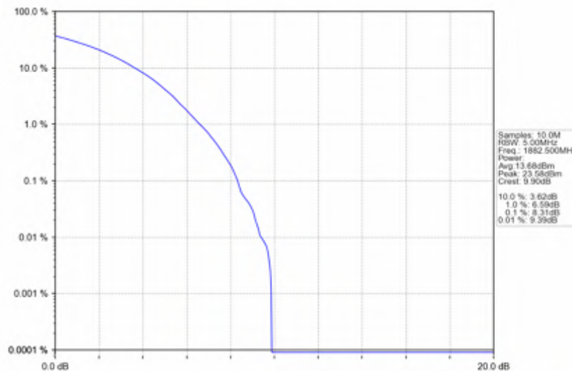
n25_15kHz_SISO_NTNV_30MHz_CP-OFDM_16_QAM_1882.5MHz_Outer_Full
