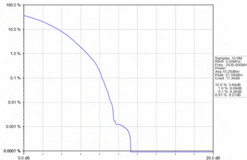
n7_30kHz_SISO_NTNV_30MHz_CP-OFDM_256_QAM_2535MHz_Outer_Full
