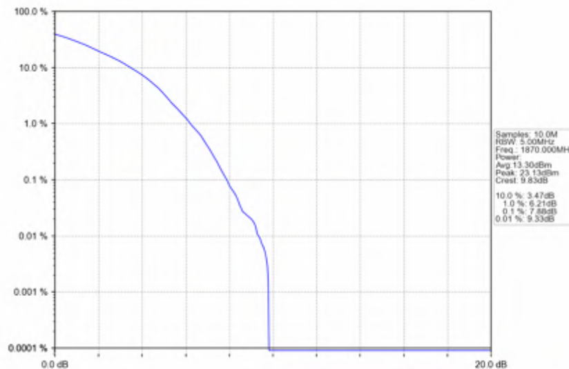
n25_15kHz_SISO_NTNV_40MHz_DFT-s-OFDM_16_QAM_1870MHz_Outer_Full
