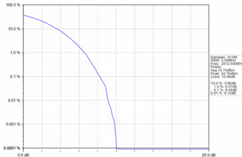
n7_30kHz_SISO_NTNV_25MHz_CP-OFDM QPSK_2512.5MHz_Outer_Full
