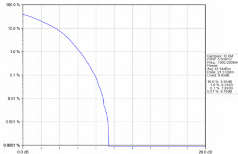
n25_15kHz_SISO_NTNV_30MHz_DFT-s-OFDM 256 QAM_1900MHz_Outer_Full
