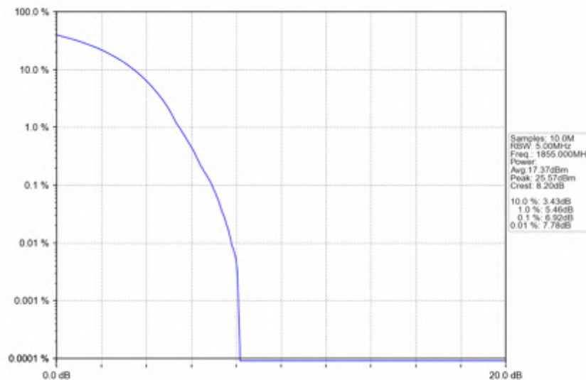
n25_15kHz_SISO_NTNV_10MHz_DFT-s-OFDM_256_QAM_1855MHz_Outer_Full
