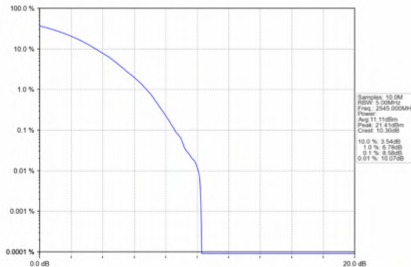
n7_30kHz_SISO_NTNV_50MHz_CP-OFDM 64 QAM_2545MHz_Outer_Full
