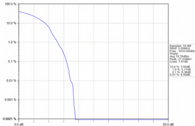
n25_30kHz_SISO_NTNV_10MHz_DFT-s-OFDM_16 QAM_1910MHz_Outer_Full
