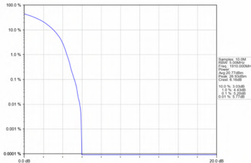
n25_30kHz_SISO_NTNV_10MHz_DFT-s-OFDM QPSK_1910MHz_Outer_Full
