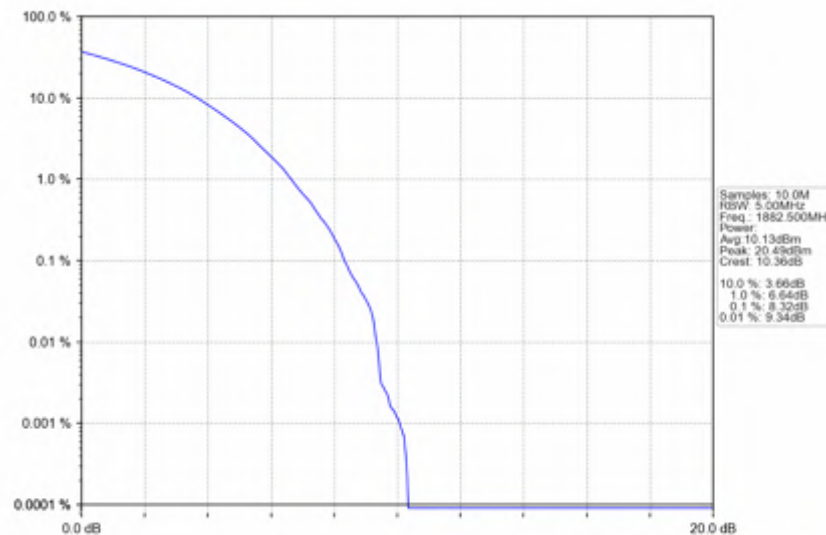
n25_15kHz_SISO_NTNV_30MHz_CP-OFDM 256 QAM_1882.5MHz_Outer_Full
