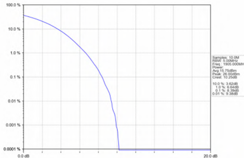
n25_15kHz_SISO_NTNV_20MHz_CP-OFDM QPSK_1905MHz_Outer_Full
