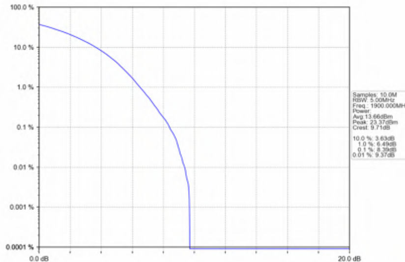
n25_15kHz_SISO_NTNV_30MHz_CP-OFDM QPSK_1900MHz_Outer_Full
