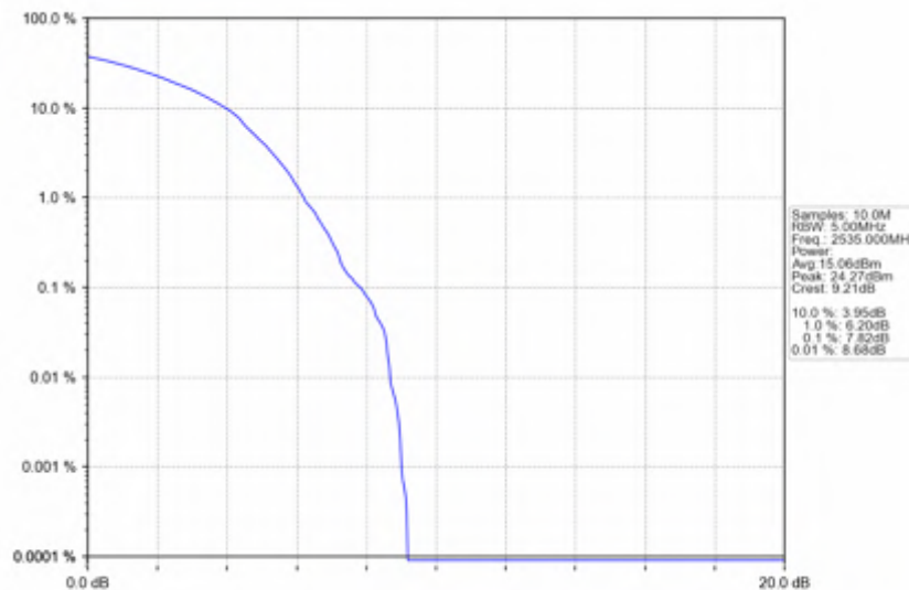
n7_30kHz_SISO_NTNV_30MHz_DFT-s-OFDM_16_QAM_2535MHz_Outer_Full
