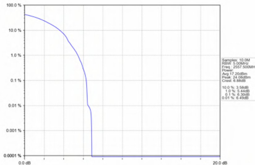
n7_30kHz_SISO_NTNV_25MHz_DFT-s-OFDM PI/2 BPSK_2557.5MHz_Outer_Full
