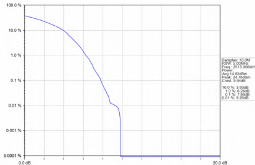
n7_30kHz_SISO_NTNV_30MHz_DFT-s-OFDM_64_QAM_2515MHz_Outer_Full
