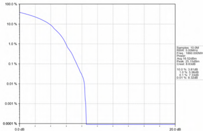
n25_15kHz_SISO_NTNV_20MHz_DFT-s-OFDM_16_QAM_1860MHz_Outer_Full
