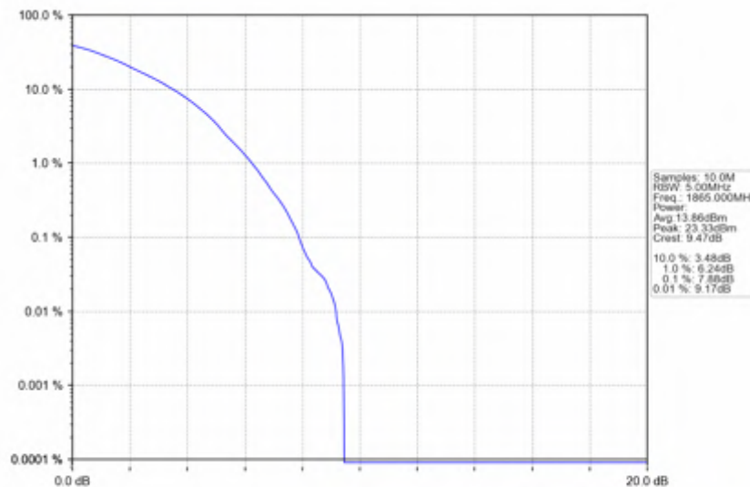
n25_15kHz_SISO_NTNV_30MHz_DFT-s-OFDM_64_QAM_1865MHz_Outer_Full
