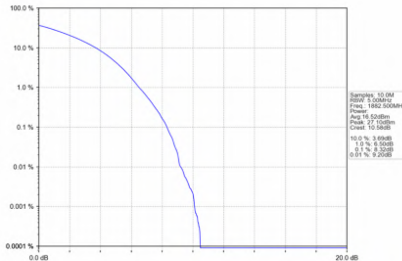
n25_15kHz_SISO_NTNV_15MHz_CP-OFDM_QPSK_1882.5MHz_Outer_Full
