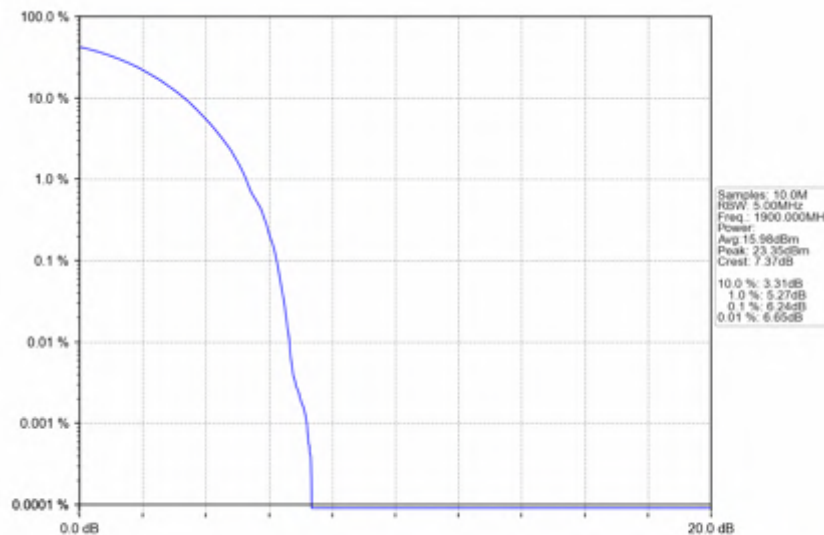
n25_15kHz_SISO_NTNV_30MHz_DFT-s-OFDM PI/2 BPSK_1900MHz_Outer_Full
