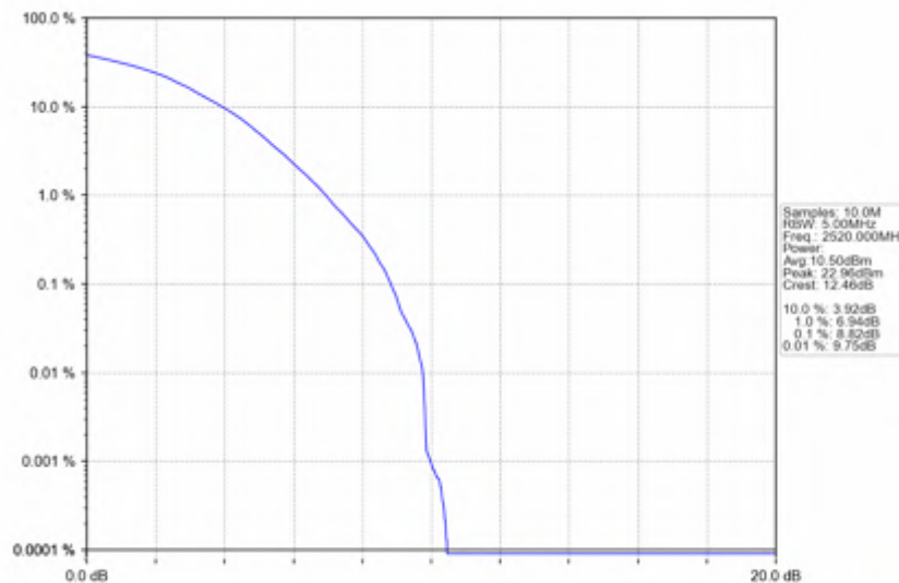
n7_30kHz_SISO_NTNV_40MHz_DFT-s-OFDM_256_QAM_2520MHz_Outer_Full
