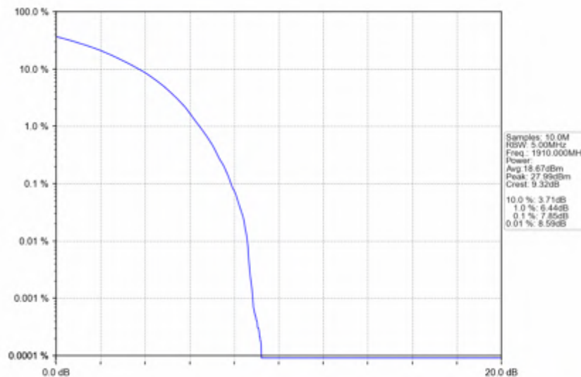
n25_30kHz_SISO_NTNV_10MHz_CP-OFDM QPSK_1910MHz_Outer_Full
