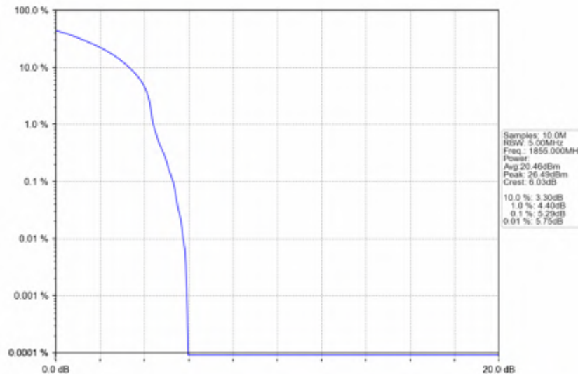
n25_30kHz_SISO_NTNV_10MHz_DFT-s-OFDM QPSK_1855MHz_Outer_Full
