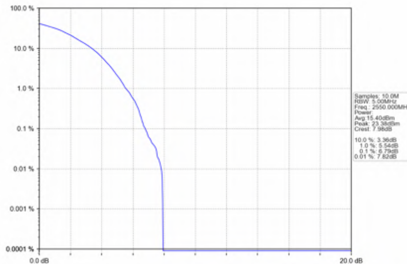
n7_30kHz_SISO_NTNV_40MHz_DFT-s-OFDM PI/2 BPSK_2550MHz_Outer_Full
