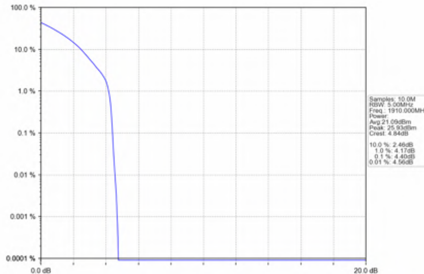
n25_30kHz_SISO_NTNV_10MHz_DFT-s-OFDM PI/2 BPSK_1910MHz_Outer_Full
