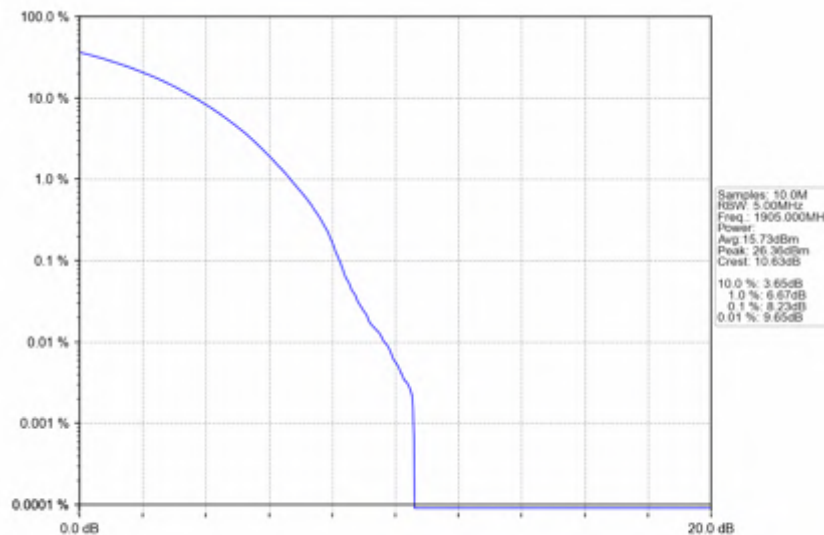
n25_15kHz_SISO_NTNV_20MHz_CP-OFDM 16 QAM_1905MHz_Outer_Full
