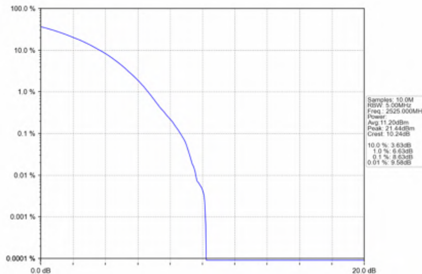
n7_30kHz_SISO_NTNV_50MHz_CP-OFDM 64 QAM_2525MHz_Outer_Full
