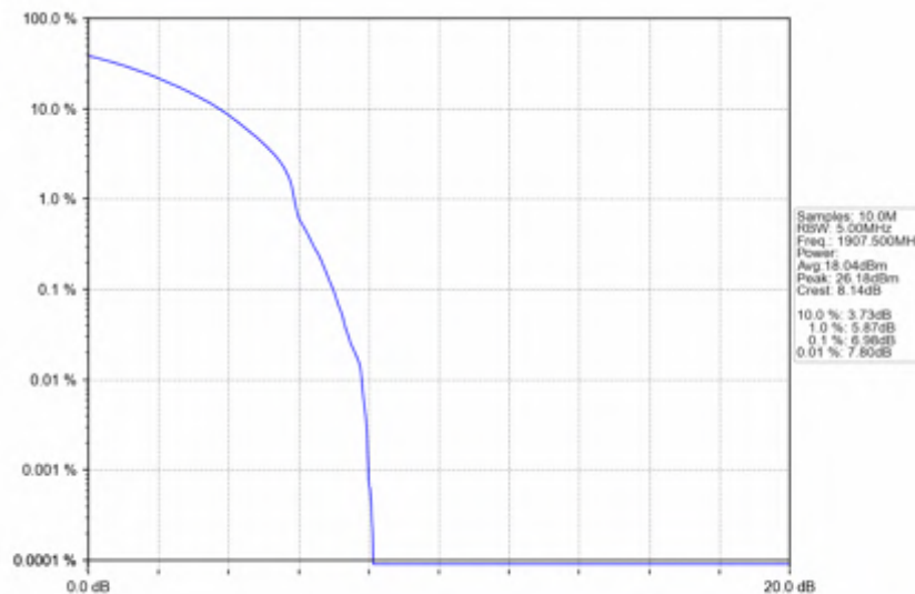
n25_15kHz_SISO_NTV_15MHz_DFT-s-OFDM 16 QAM_1907.5MHz_Outer_Full
