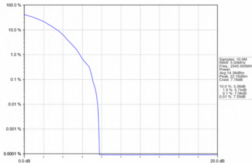
n7_30kHz_SISO_NTNV_50MHz_DFT-s-OFDM PI/2 BPSK_2545MHz_Outer_Full
