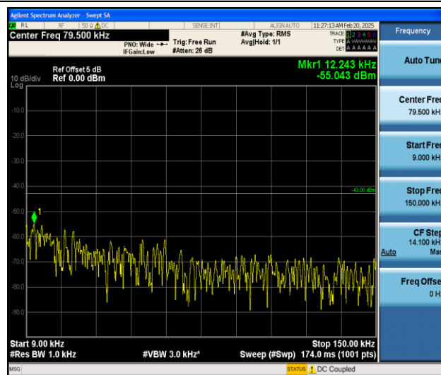
Band25_3MHz_QPSK_26055_1RB#0_0.009~0.15_0.009~0.15
