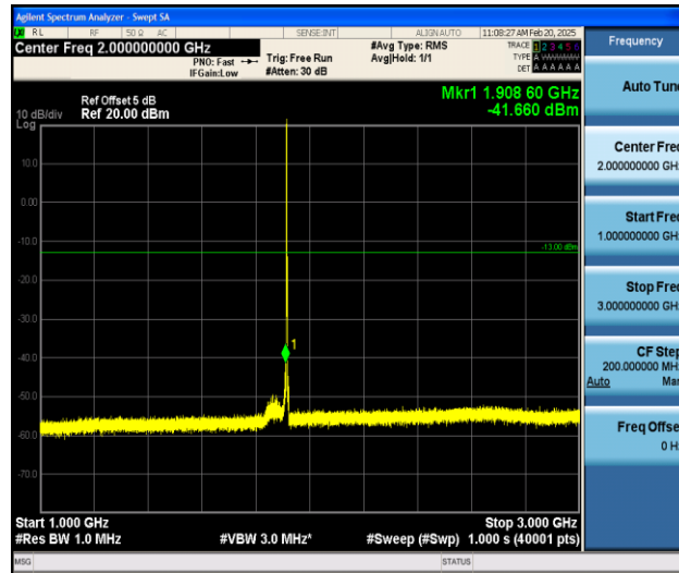
Band25_1.4MHz_16QAM_26683_1RB#0_1000~3000_1000~3000
