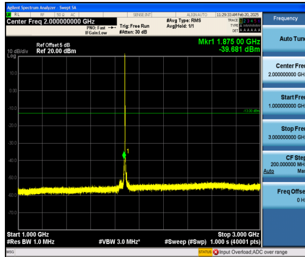
Band25_3MHz_QPSK_26365_1RB#0_1000~3000_1000~3000
