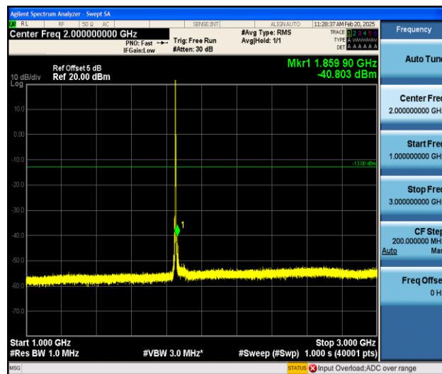
Band25_3MHz_16QAM_26055_1RB#0_1000~3000_1000~3000
