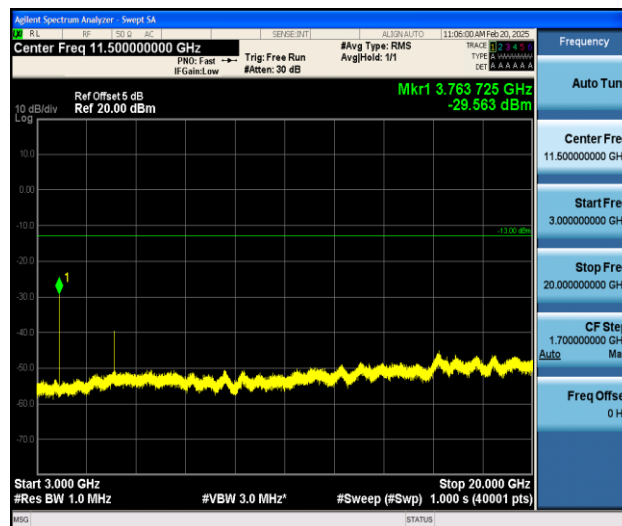
Band25_1.4MHz_QPSK_26365_1RB#0_3000~20000_3000~20000
