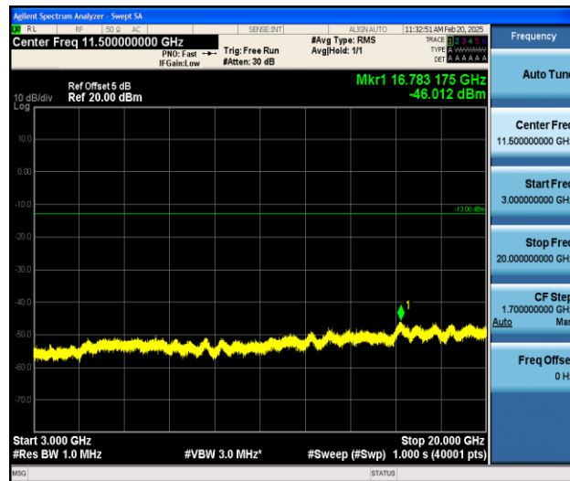
Band25_3MHz_16QAM_26675_1RB#0_3000~20000_3000~20000
