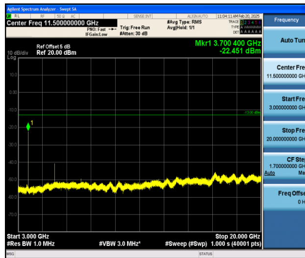
Band25_1.4MHz_QPSK_26047_1RB#0_3000~20000_3000~20000
