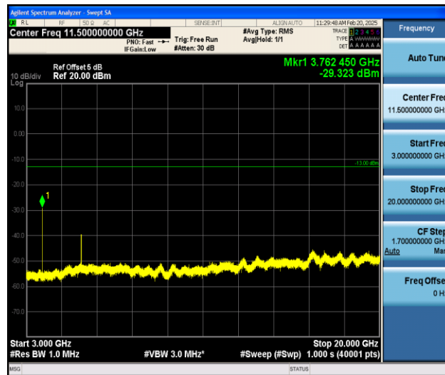
Band25_3MHz_QPSK_26365_1RB#0_3000~20000_3000~20000
