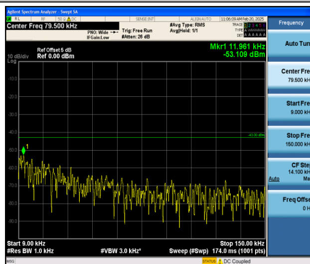
Band25_1.4MHz_16QAM_26365_1RB#0_0.009~0.15_0.009~0.15
