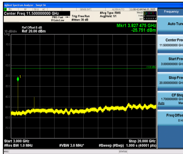
Band25_1.4MHz_16QAM_26683_1RB#0_3000~20000_3000~20000
