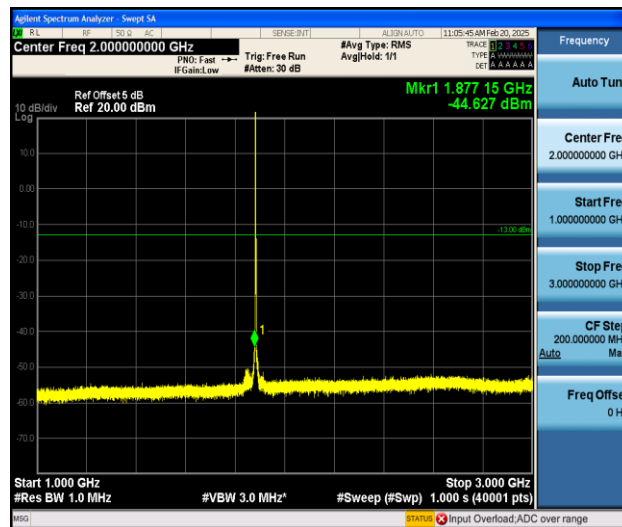
Band25_1.4MHz_QPSK_26365_1RB#0_1000~3000_1000~3000
