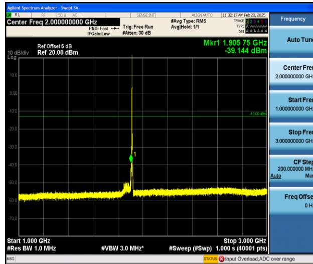
Band25_3MHz_16QAM_26675_1RB#0_1000~3000_1000~3000
