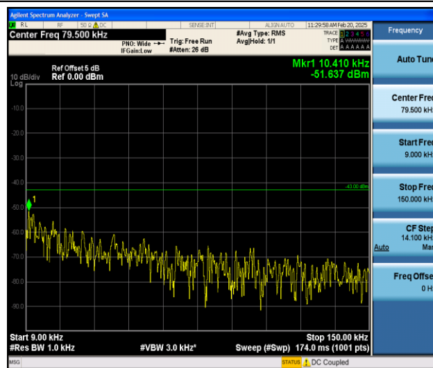
Band25_3MHz_16QAM_26365_1RB#0_0.009~0.15_0.009~0.15
