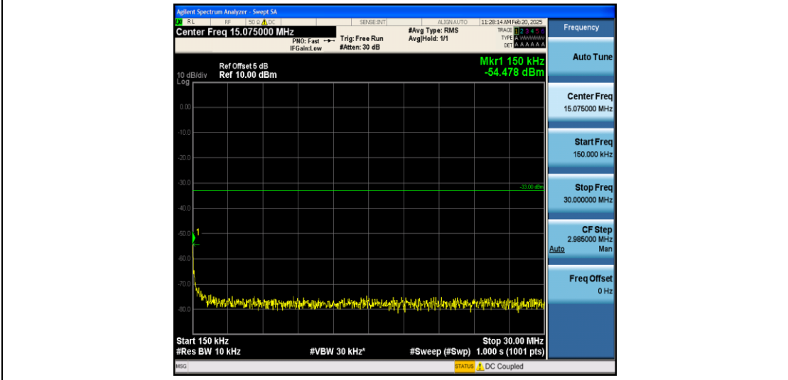
Band25_3MHz_16QAM_26055_1RB#0_0.15~30_0.15~30
