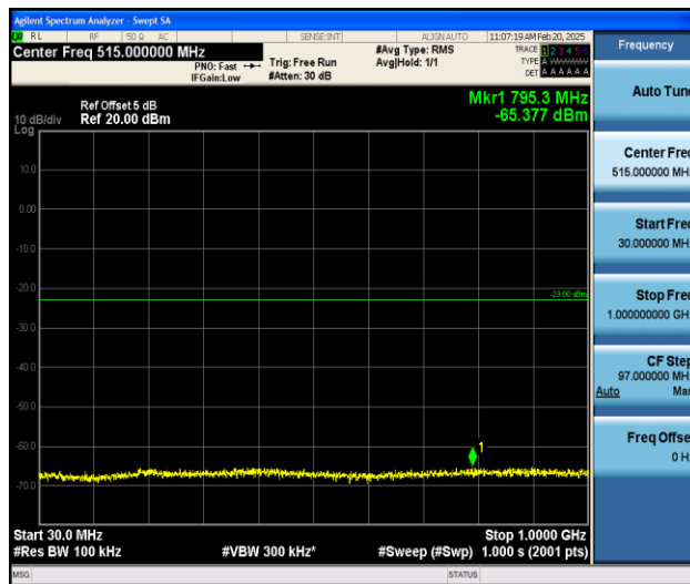
Band25_1.4MHz_QPSK_26683_1RB#0_30~1000_30~1000
