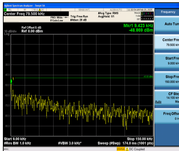
Band25_3MHz_QPSK_26675_1RB#0_0.009~0.15_0.009~0.15
