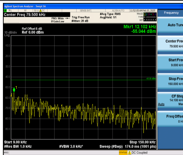
Band25_5MHz_QPSK_26065_1RB#0_0.009~0.15_0.009~0.15
