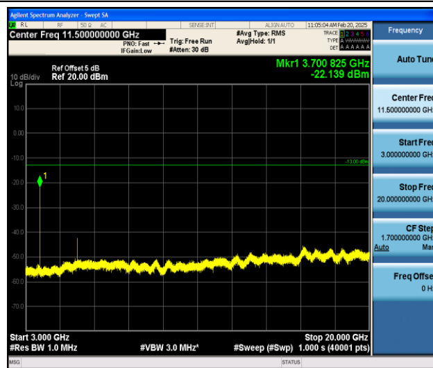
Band25_1.4MHz_16QAM_26047_1RB#0_3000~20000_3000~20000
