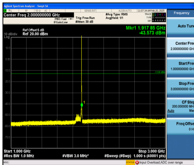
Band25_1.4MHz_QPSK_26683_1RB#0_1000~3000_1000~3000
