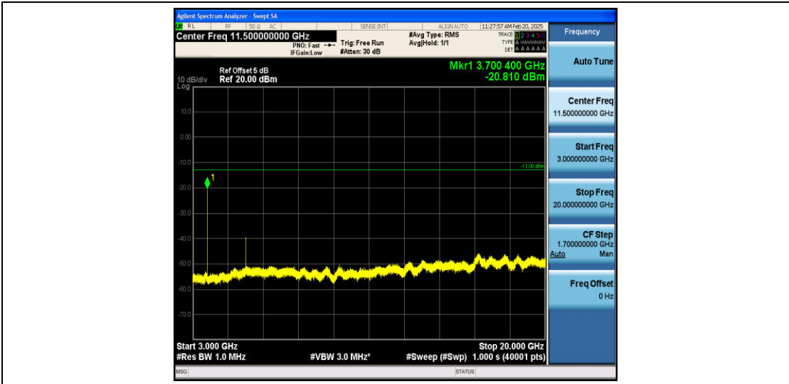
Band25_3MHz_QPSK_26055_1RB#0_3000~20000_3000~20000
