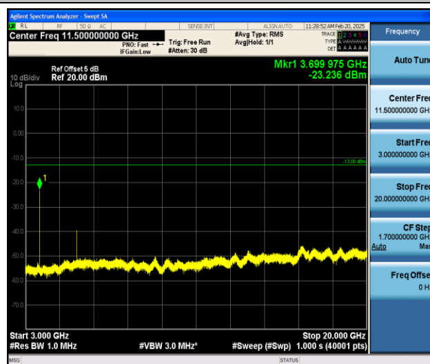
Band25_3MHz_16QAM_26055_1RB#0_3000~20000_3000~20000
