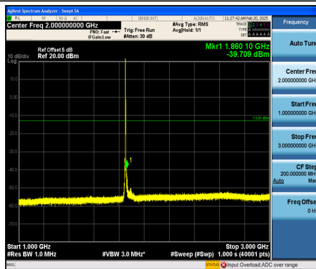
Band25_3MHz_QPSK_26055_1RB#0_1000~3000_1000~3000
