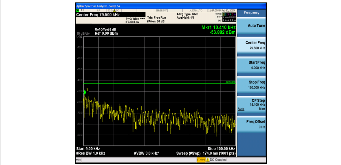
Band25_1.4MHz_QPSK_26683_1RB#0_0.009~0.15_0.009~0.15
