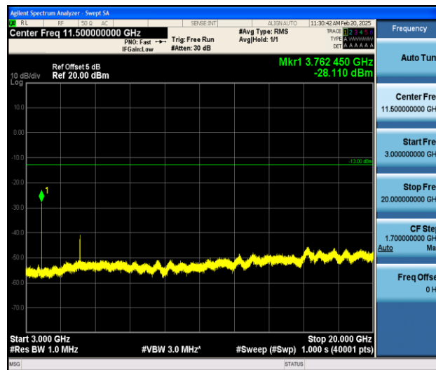
Band25_3MHz_16QAM_26365_1RB#0_3000~20000_3000~20000
