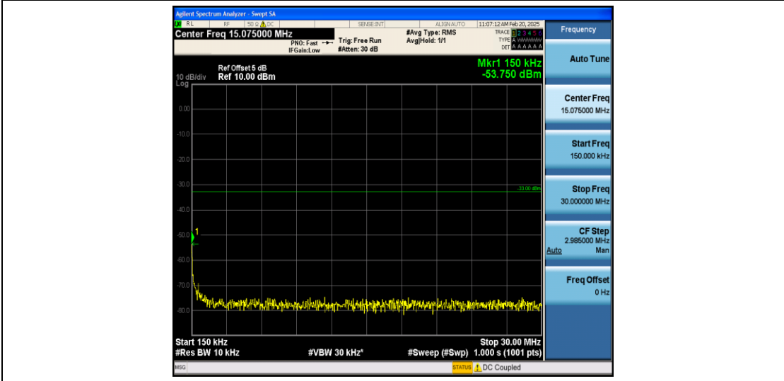
Band25_1.4MHz_QPSK_26683_1RB#0_0.15~30_0.15~30
