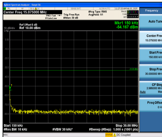
Band25_3MHz_QPSK_26055_1RB#0_0.15~30_0.15~30
