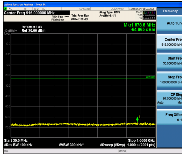
Band25_1.4MHz_16QAM_26047_1RB#0_30~1000_30~1000
