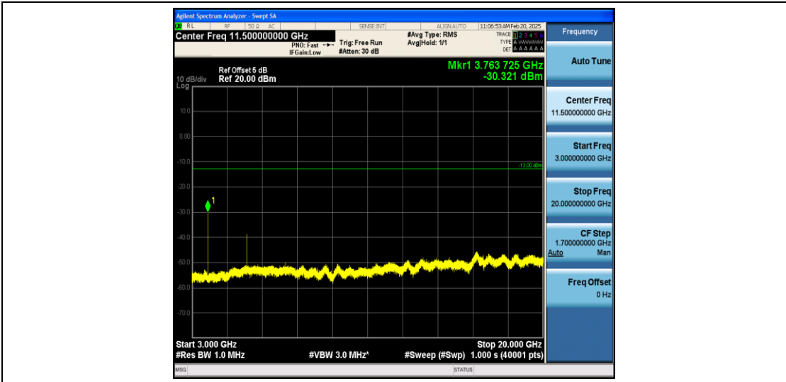
Band25_1.4MHz_16QAM_26365_1RB#0_3000~20000_3000~20000
