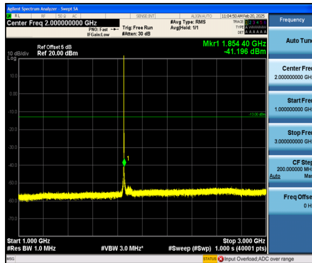
Band25_1.4MHz_16QAM_26047_1RB#0_1000~3000_1000~3000
