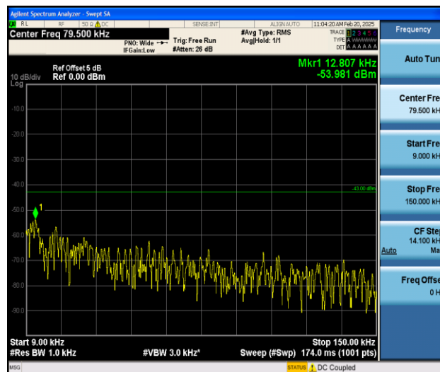
Band25_1.4MHz_16QAM_26047_1RB#0_0.009~0.15_0.009~0.15
