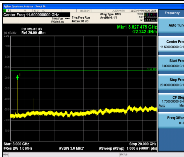
Band25_1.4MHz_QPSK_26683_1RB#0_3000~20000_3000~20000
