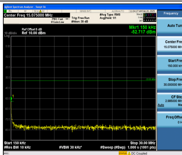
Band25_1.4MHz_16QAM_26047_1RB#0_0.15~30_0.15~30
