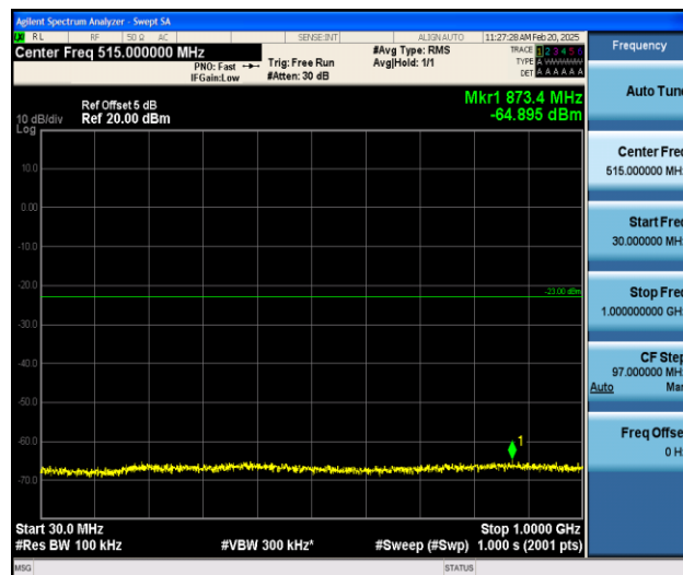
Band25_3MHz_QPSK_26055_1RB#0_30~1000_30~1000
