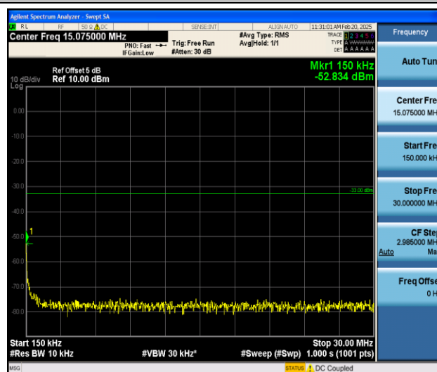
Band25_3MHz_QPSK_26675_1RB#0_0.15~30_0.15~30
