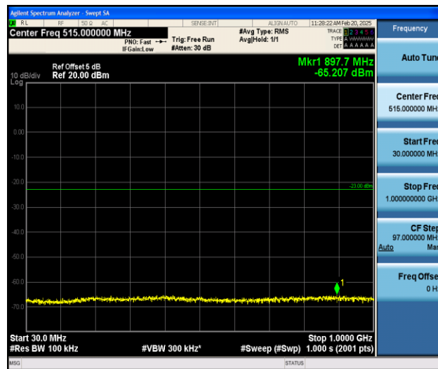
Band25_3MHz_16QAM_26055_1RB#0_30~1000_30~1000
