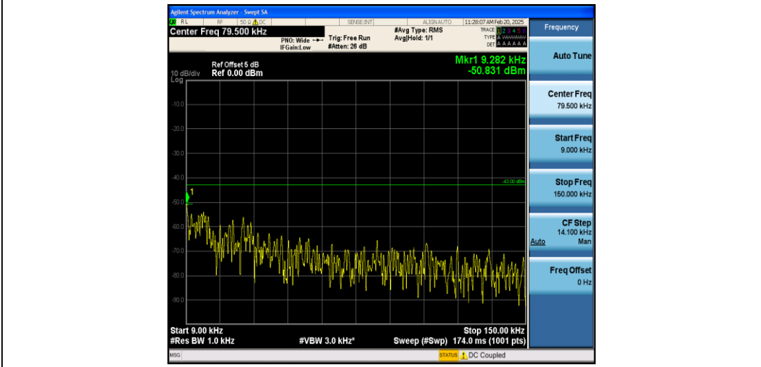
Band25_3MHz_16QAM_26055_1RB#0_0.009~0.15_0.009~0.15
