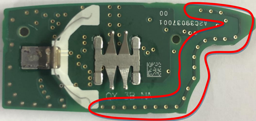
PCB Antenna
