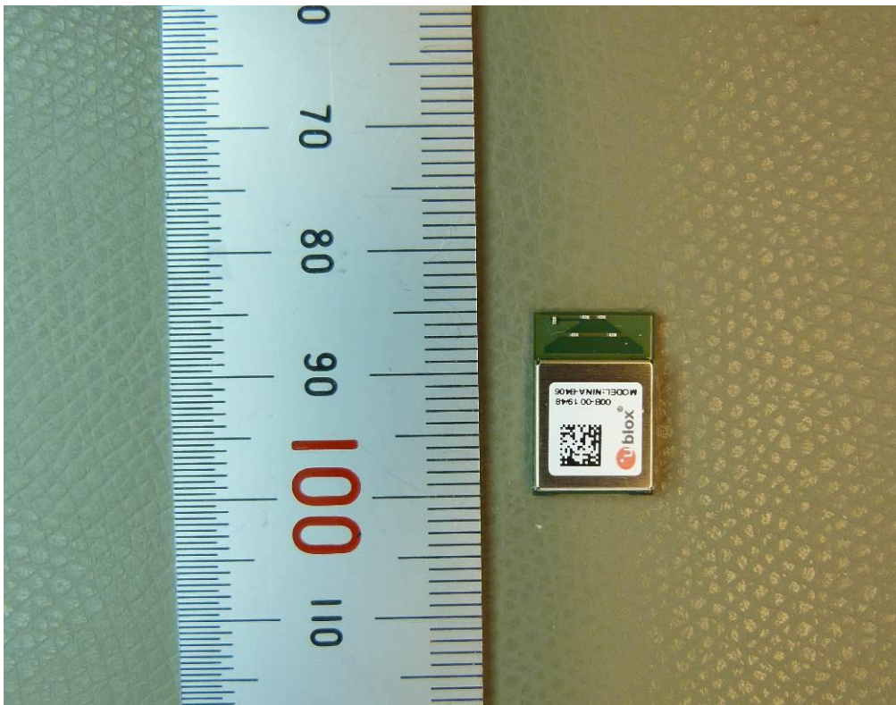
TOP VIEW OF EUT (NINA-B406)
