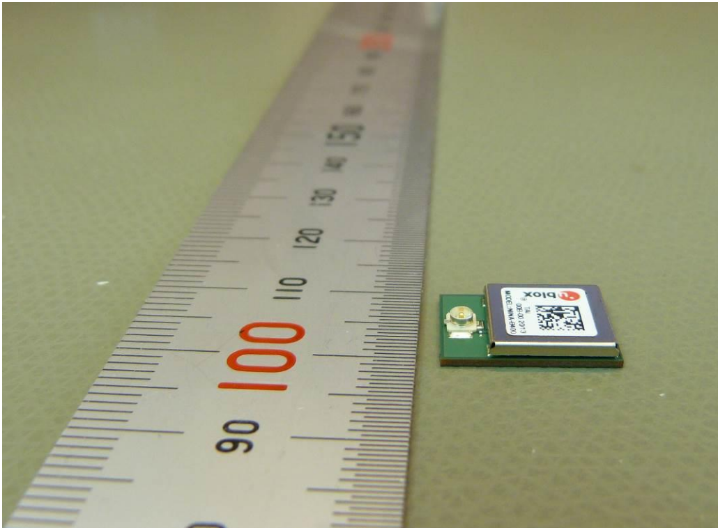
RIGHT VIEW OF EUT (NINA-B400)
