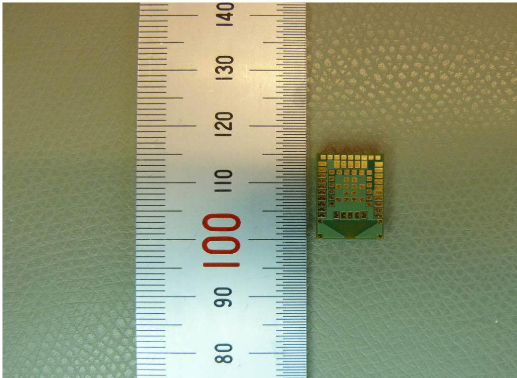
FRONT VIEW OF EUT (NINA-B416)
