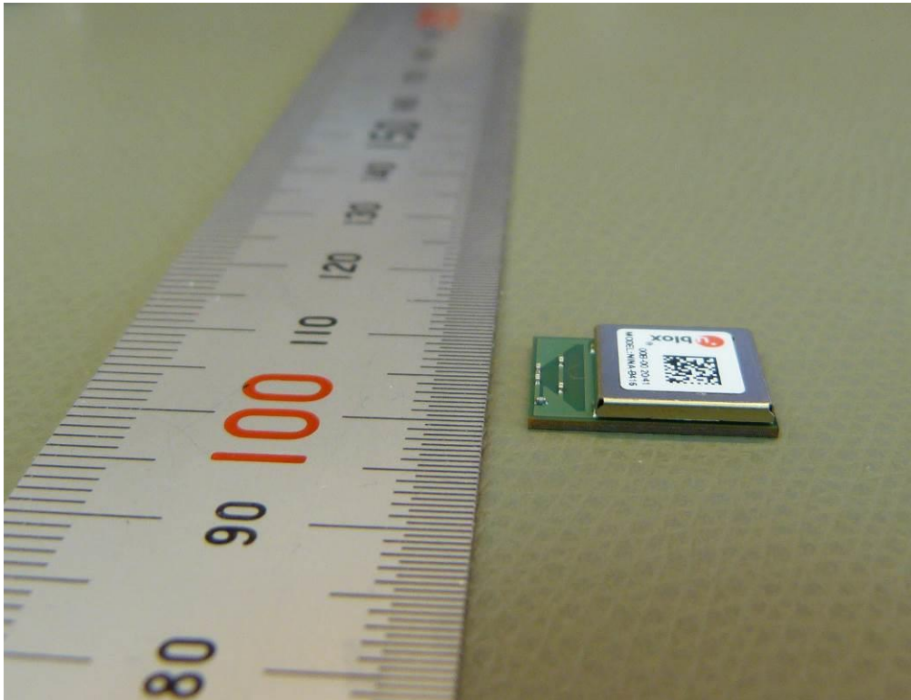
RIGHT VIEW OF EUT (NINA-B416)
