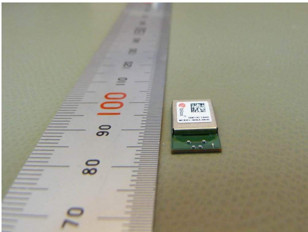
FRONT VIEW OF EUT (NINA-B406)
