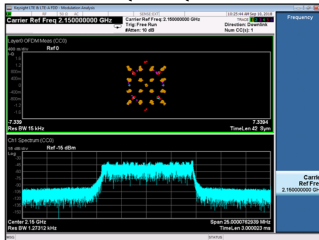
QPSK+16QAM
