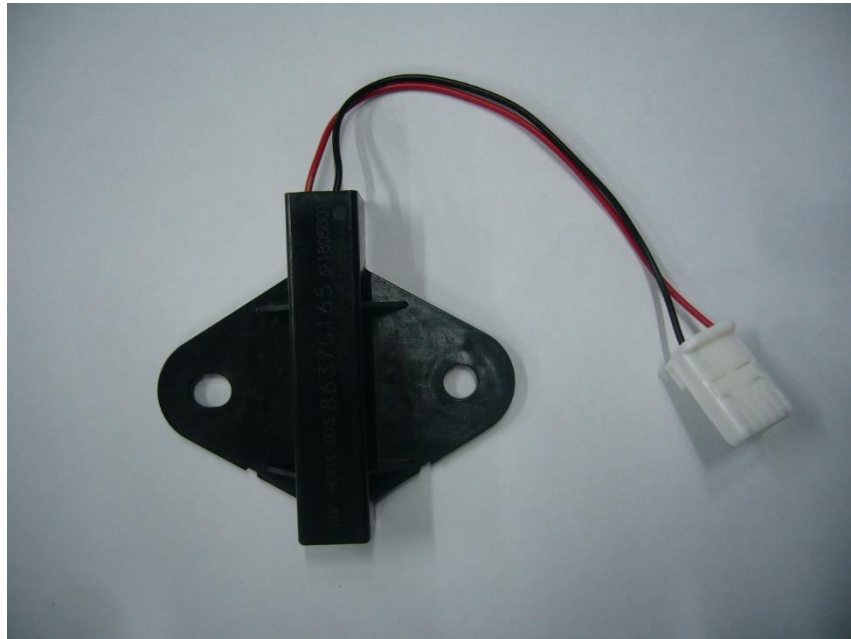
Figure 8.13 CGF-M004-T03 appearance (front view)
