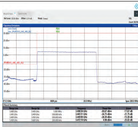
1-N78-3450-3550-PC1-30-90-L-3-DFT-PI2BPSK-Outer_Full-240@0-Ant1-1--PASS-see graph
