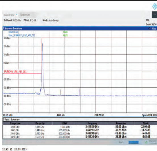
1-N78-3450-3550-PC1-30-50-L-4-CP-QPSK-Edge_1RB_Left-1@0-Ant1-1--PASS-see graph
