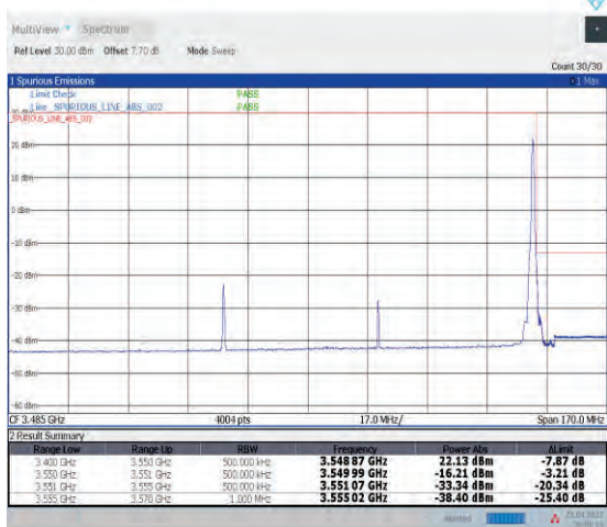
1-N78-3450-3550--30-90-H-5-CP-QPSK-Edge_1RB_Right-1@244-Ant1-PASS-see graph
