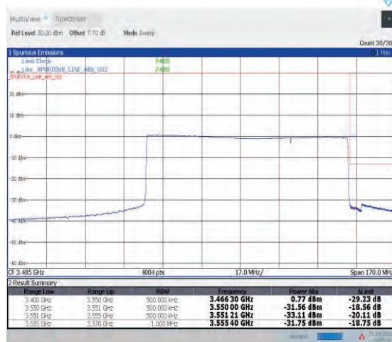
1-N78-3450-3550--30-90-H-6-CP-QPSK-Outer_Full-245@0-Ant1-PASS-see graph
