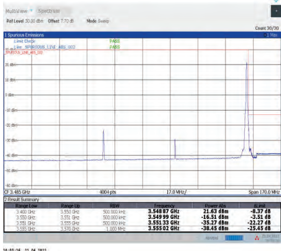
1-N78-3450-3550--30-90-H-2-DFT-PI2BPSK-Edge_1R_B_Right-1@244-Ant1-PASS-see graph
