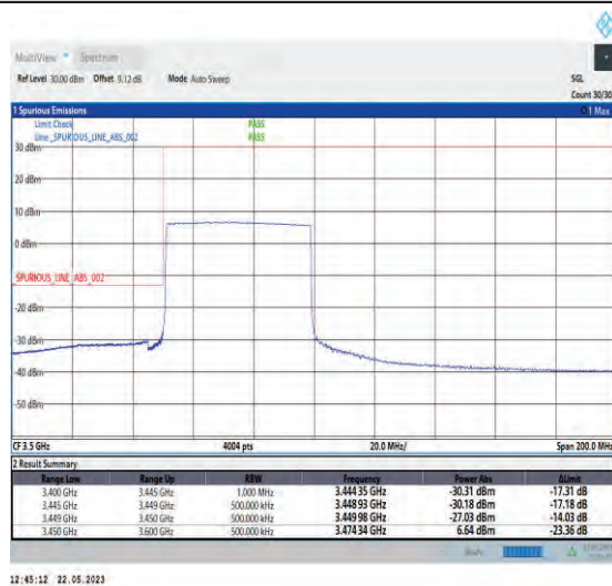
1-N78-3450-3550-PC1-30-50-L-6-CP-QPSK-Outer_Full-133@0-Ant1-1--PASS-see graph
