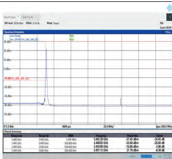
1-N78-3450-3550-PC1-30-90-L-1-DFT-PI2BPSK-Edge_1RB_Left-1@0-Ant1-1--PASS-see graph
