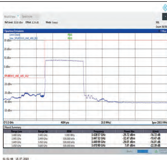
1-N78-3450-3550-PC1-30-50-L-3-DFT-PI2BPSK-Outer_Full-128@0-Ant1-1--PASS-see graph
