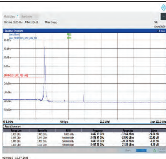
1-N78-3450-3550-PC1-30-50-L-1-DFT-PI2BPSK-Edge_1RB_Left-1@0-Ant1-1--PASS-see graph
