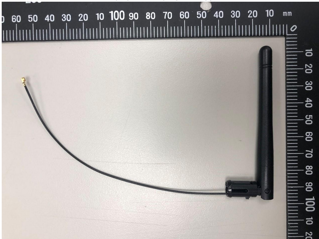
Ant No.2: RFA-02-C2H1-D034
