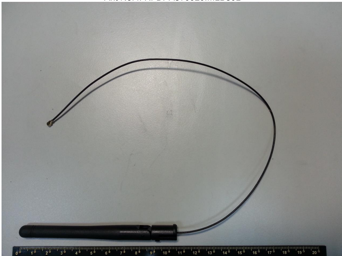
Ant No.4: RFDPA870920IMLB301
