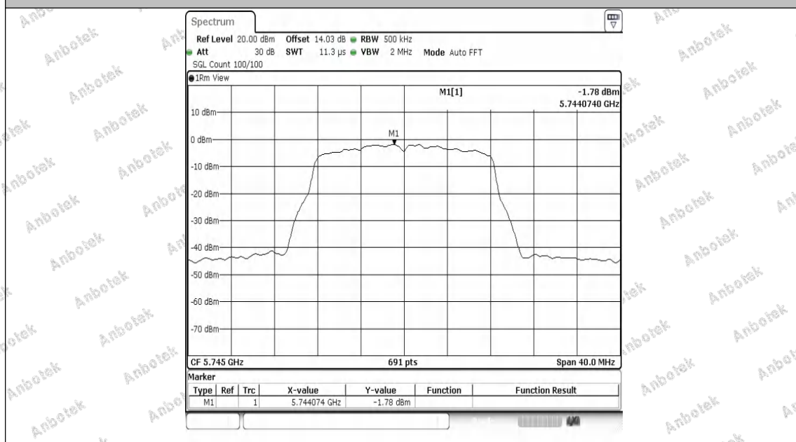
11A-Ant1-5745-PASS
