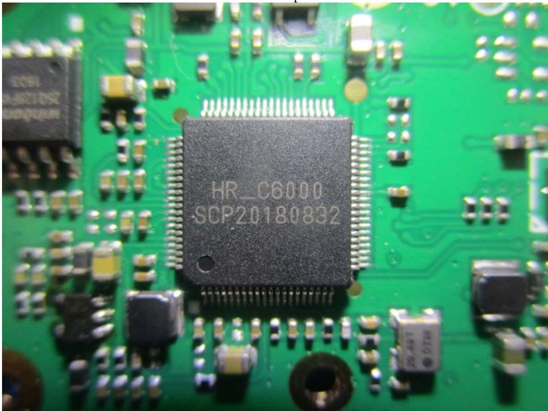
RF Chip
