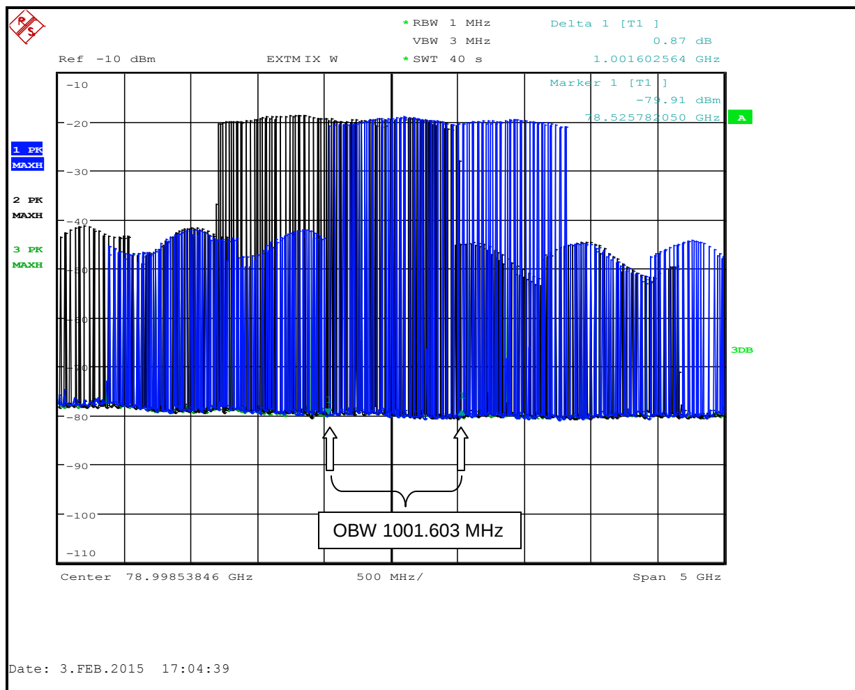
Plot 3-2: 10 dB Modulated Bandwidth – TC #2
