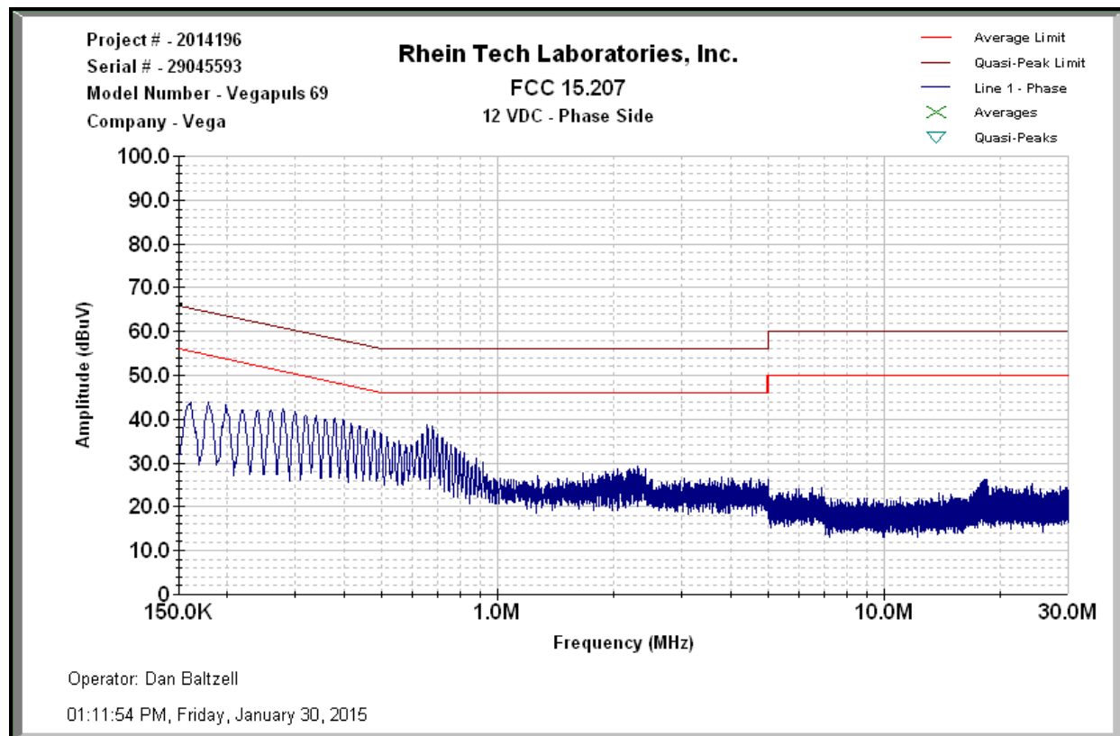
Plot 6-1: Conducted Emissions Transmit - Phase (TC #1)
