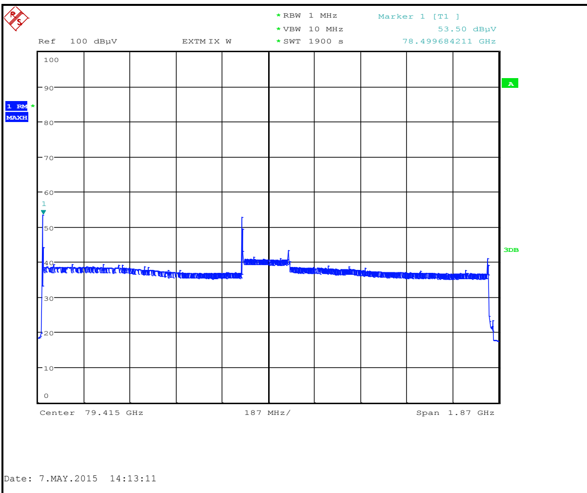
Plot 4-4: Radiated Fundamental (EIRP in 1 MHz) (TC #2)
