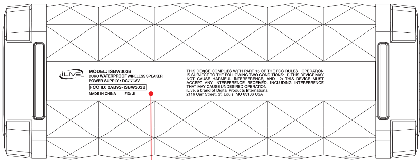
BOTTOM VIEW
