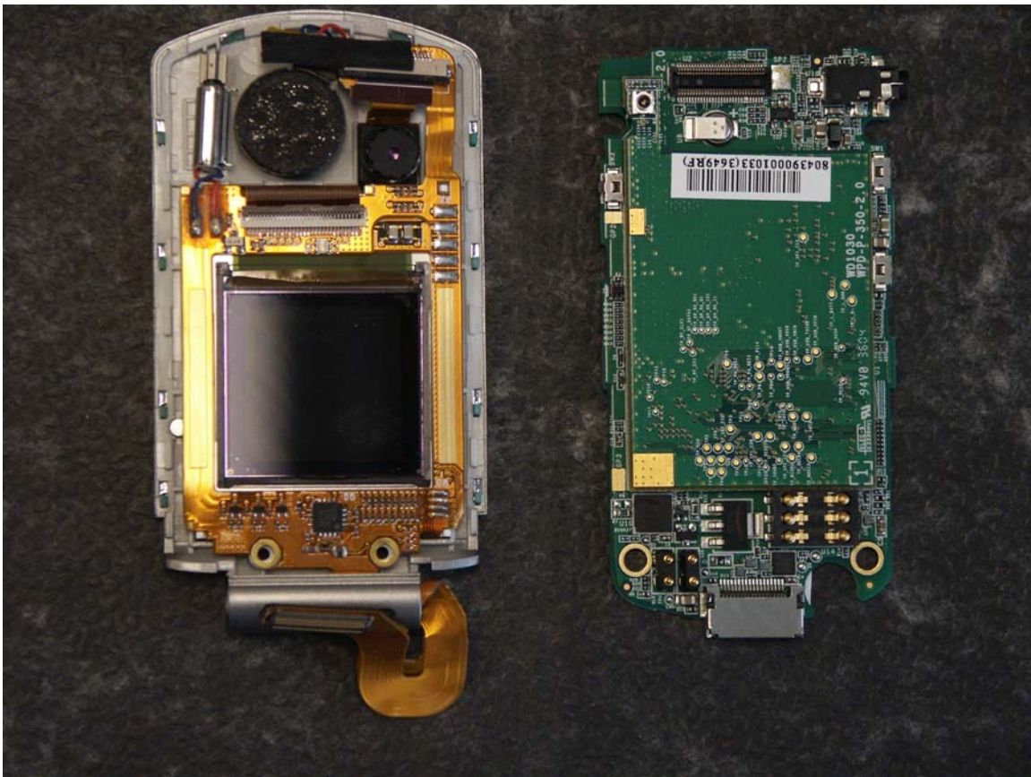
Photo 3. External Display and Flexible PCB (left) Radio Board attached to Keypad board (right)
