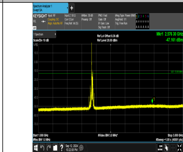
Band4_20MHz_QPSK_20300_1RB#0_1000-3000_1000-3000
