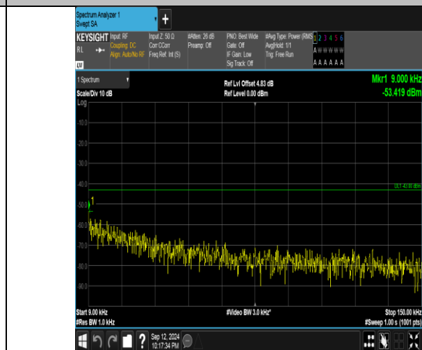
Band4_20MHz_16QAM_20175_1RB#0_0.009-0.15_0.009-0.15
