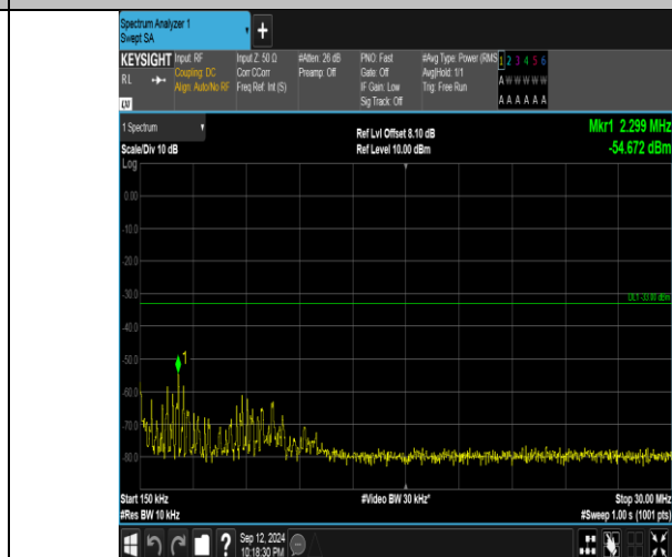
Band4_20MHz_QPSK_20175_1RB#99_0.15~30_0.15~30
