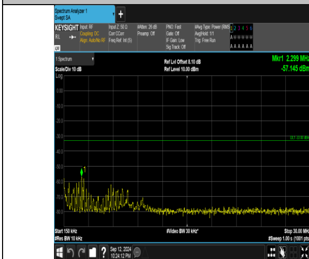
Band4_20MHz_16QAM_20300_1RB#99_0.15~30_0.15~30
