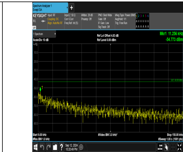
Band4_20MHz_16QAM_20175_100RB#0_0.009~0.15_0.009~0.15
