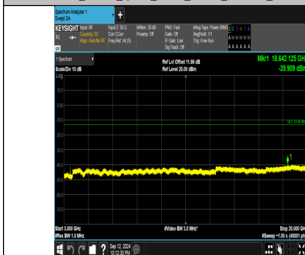
Band4_20MHz_QPSK_20050_1RB#0_3000-20000_3000-20000
