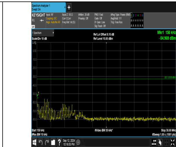
Band4_20MHz_QPSK_20175_1RB#0_0.15-30_0.15-30
