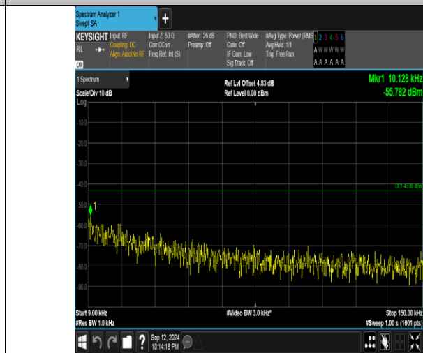
Band4_20MHz_16QAM_20050_1RB#99_0.009~0.15_0.009~0.15
