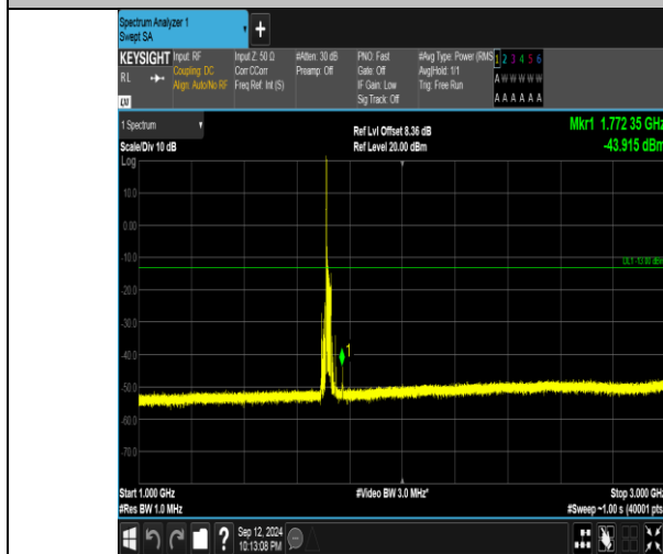
Band4_20MHz_16QAM_20050_1RB#0_1000~3000_1000~3000
