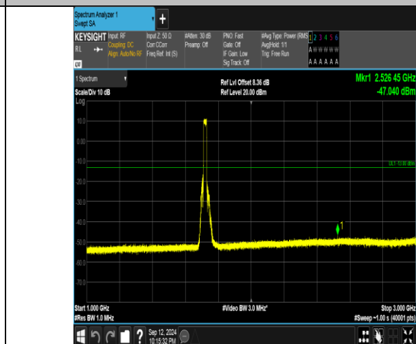
Band4_20MHz_QPSK_20050_100RB#0_1000~3000_1000~3000
