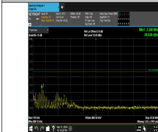
Band4_20MHz_16QAM_20050_1RB#99_0.15~30_0.15~30
