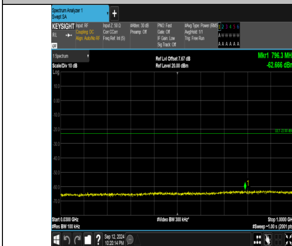
Band4_20MHz_QPSK_20175_100RB#0_30~1000_30~1000
