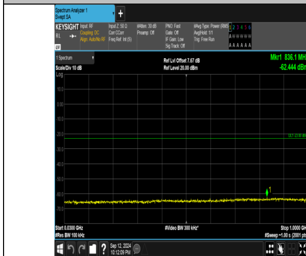
Band4_20MHz_QPSK_20050_1RB#0_30-1000_30-1000
