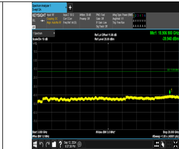
Band4_15MHz_16QAM_20325_1RB#74_3000~20000_3000~20000
