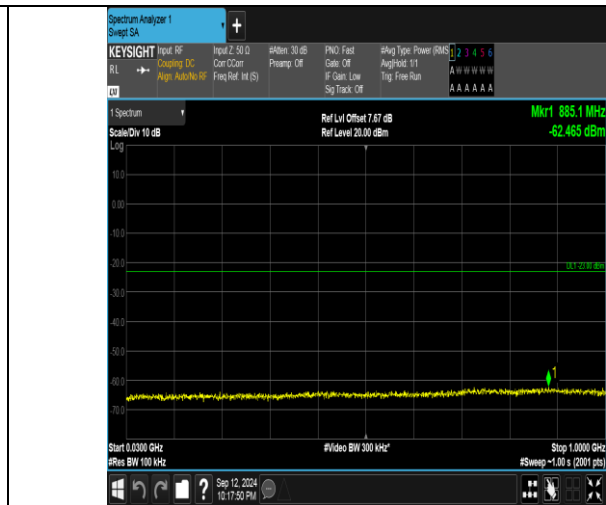
Band4_20MHz_16QAM_20175_1RB#0_30~1000_30~1000
