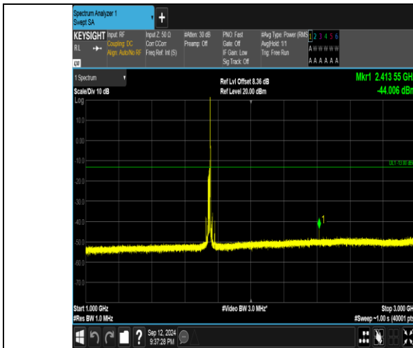
Band4_15MHz_16QAM_20325_1RB#74_1000~3000_1000~3000
