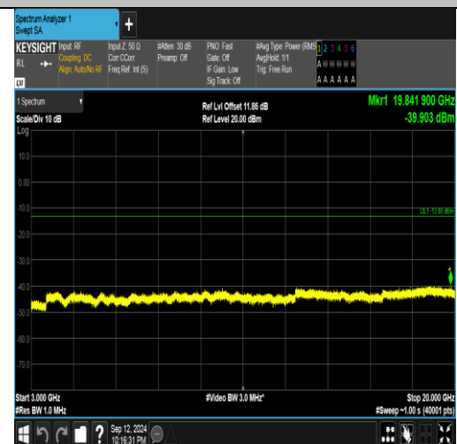
Band4_20MHz_16QAM_20050_100RB#0_3000~20000_3000~20000
