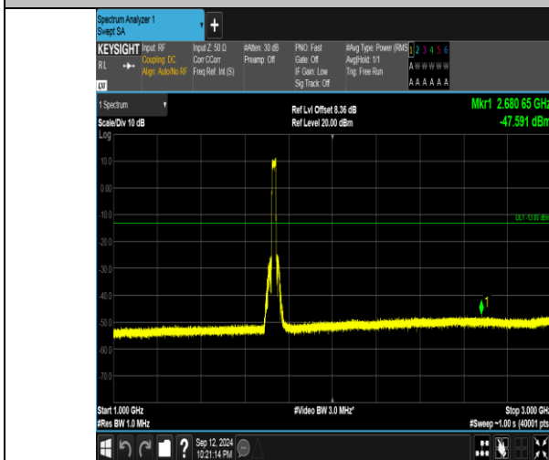
Band4_20MHz_16QAM_20175_100RB#0_1000~3000_1000~3000
