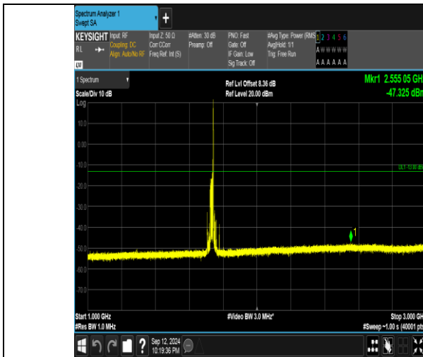
Band4_20MHz_16QAM_20175_1RB#99_1000~3000_1000~3000
