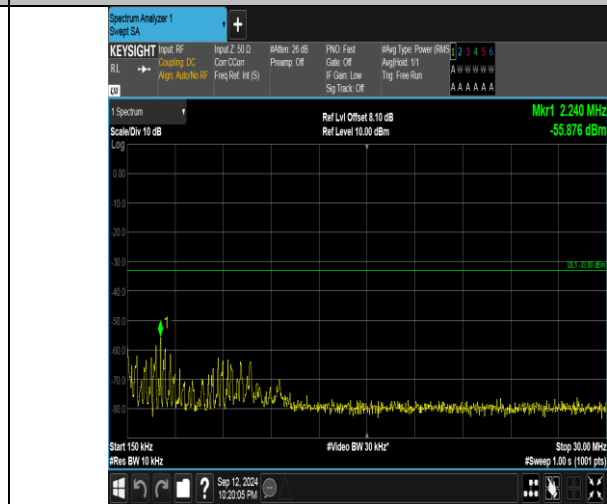
Band4_20MHz_QPSK_20175_100RB#0_0.15~30_0.15~30
