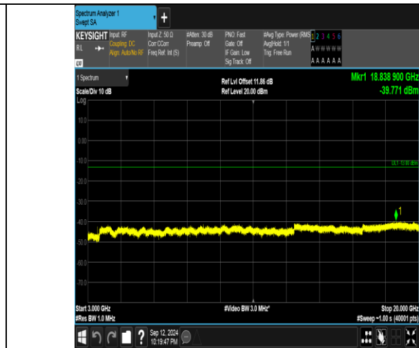
Band4_20MHz_16QAM_20175_1RB#99_3000~20000_3000~20000
