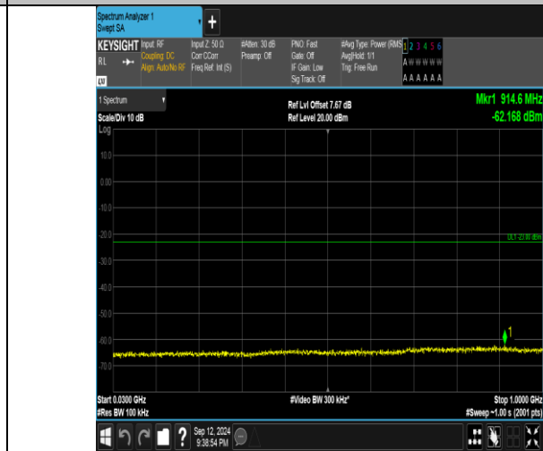
Band4_15MHz_16QAM_20325_75RB#0_30~1000_30~1000
