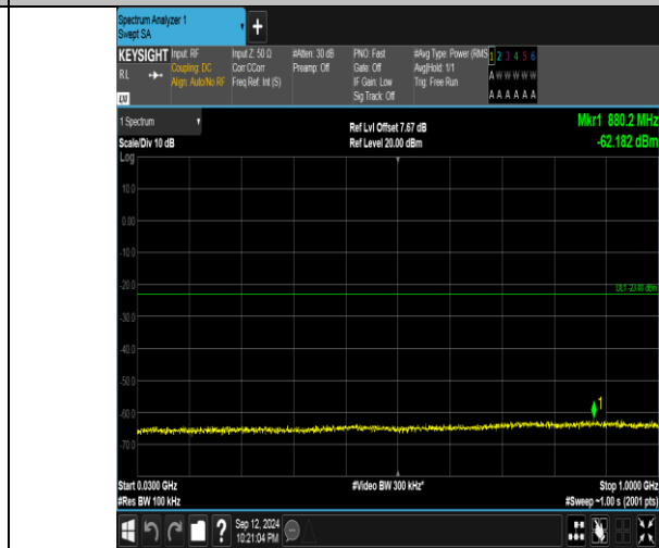
Band4_20MHz_16QAM_20175_100RB#0_30~1000_30~1000
