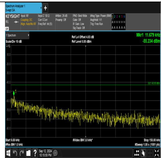
Band4_20MHz_16QAM_20050_100RB#0_0.009~0.15_0.009~0.15
