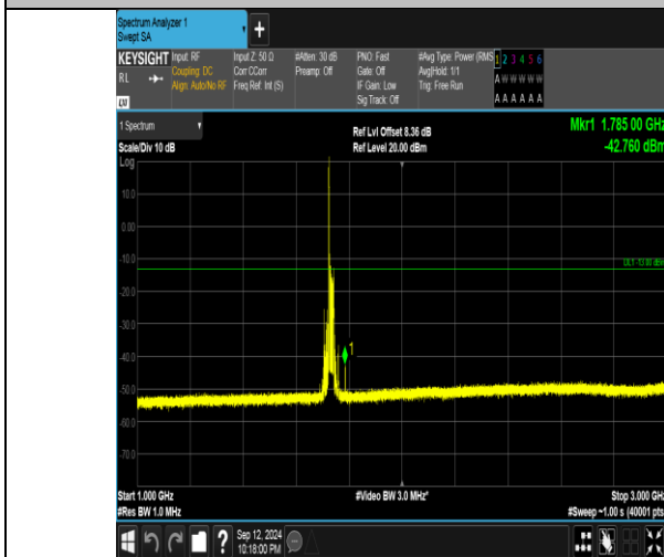
Band4_20MHz_16QAM_20175_1RB#0_1000~3000_1000~3000
