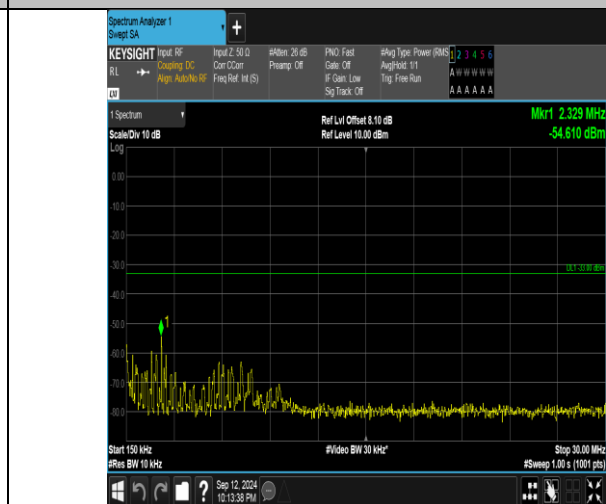
Band4_20MHz_QPSK_20050_1RB#99_0.15~30_0.15~30
