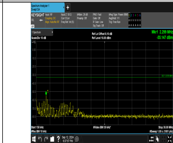
Band4_15MHz_QPSK_20325_75RB#0_0.15~30_0.15~30
