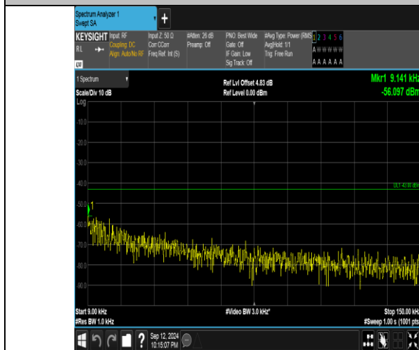
Band4_20MHz_QPSK_20050_100RB#0_0.009~0.15_0.009~0.15
