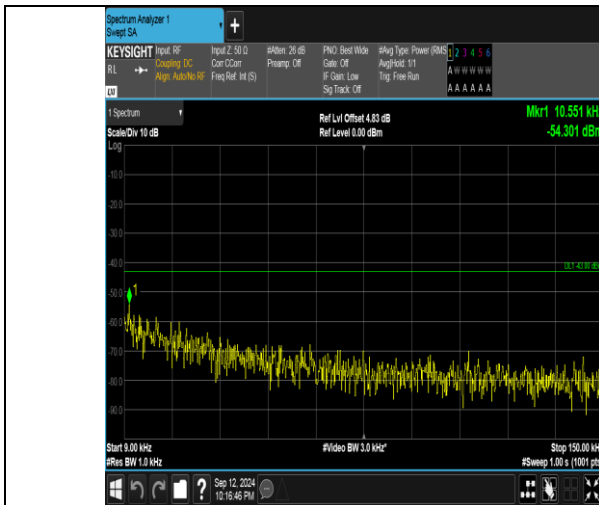
Band4_20MHz_QPSK_20175_1RB#0_0.009-0.15_0.009-0.15
