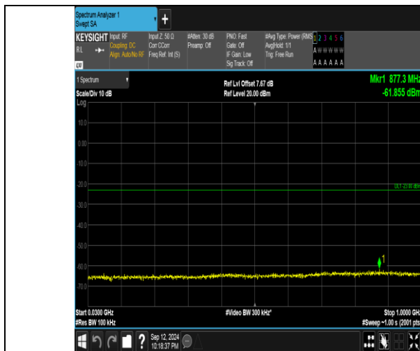
Band4_20MHz_QPSK_20175_1RB#99_30~1000_30~1000
