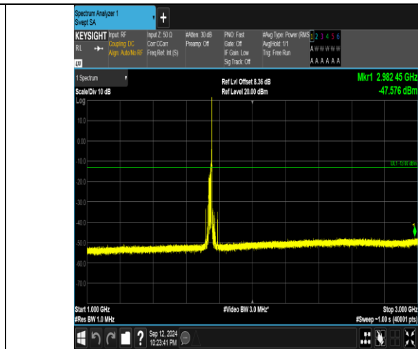
Band4_20MHz_QPSK_20300_1RB#99_1000~3000_1000~3000
