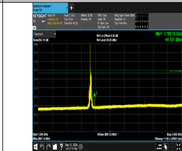
Band4_20MHz_QPSK_20175_1RB#0_1000-3000_1000-3000
