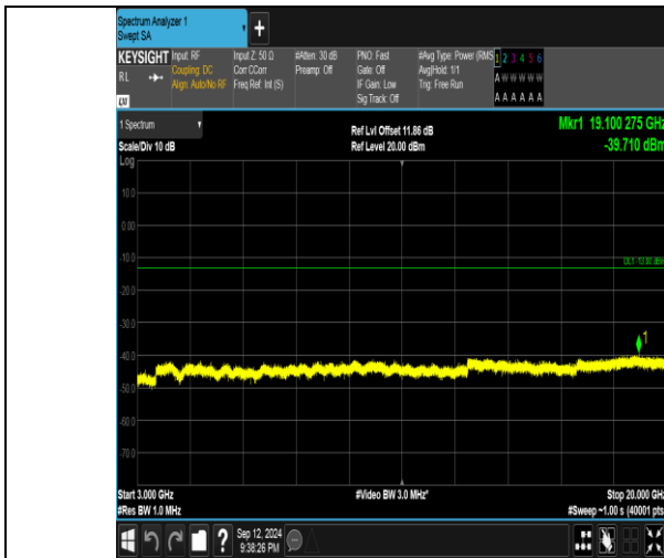
Band4_15MHz_QPSK_20325_75RB#0_3000~20000_3000~20000
