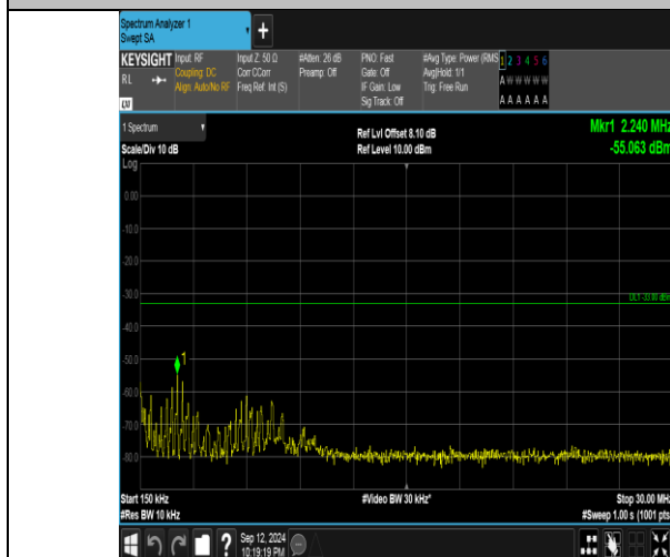
Band4_20MHz_16QAM_20175_1RB#99_0.15~30_0.15~30
