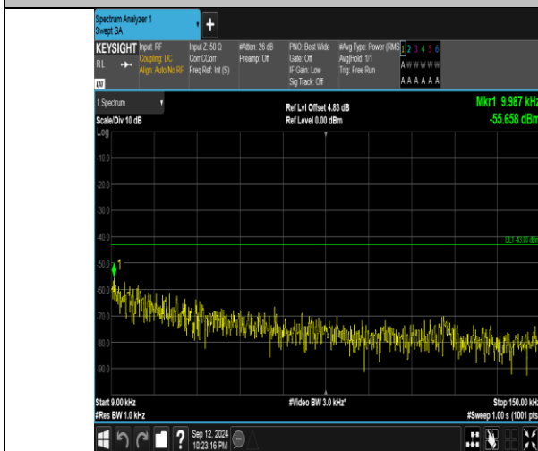
Band4_20MHz_QPSK_20300_1RB#99_0.009~0.15_0.009~0.15
