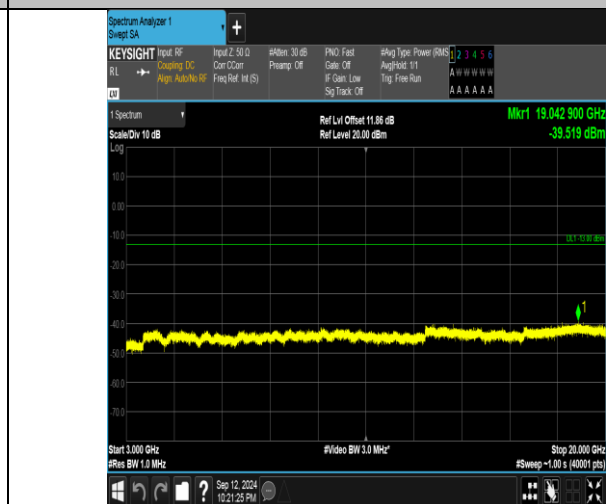
Band4_20MHz_16QAM_20175_100RB#0_3000~20000_3000~20000
