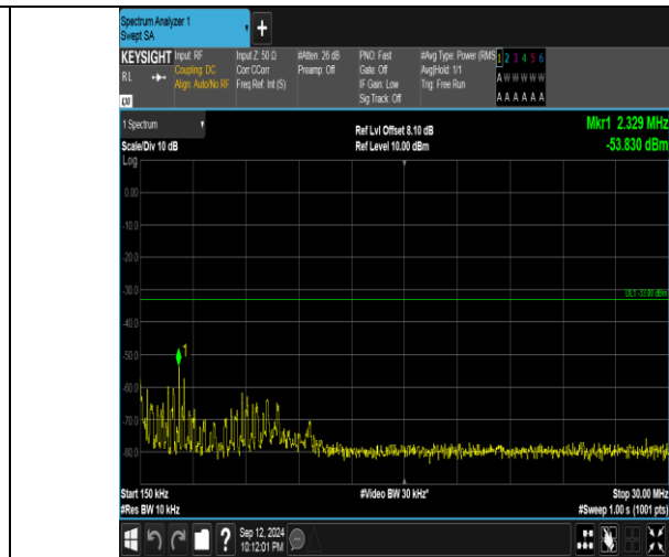
Band4_20MHz_QPSK_20050_1RB#0_0.15-30_0.15-30
