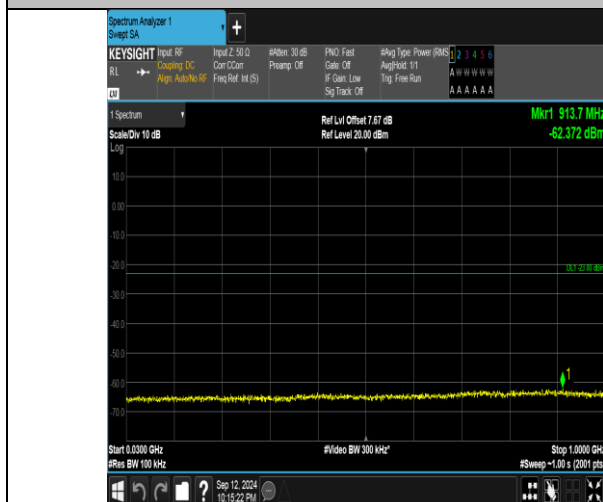
Band4_20MHz_QPSK_20050_100RB#0_30~1000_30~1000
