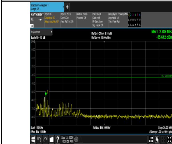
Band4_20MHz_16QAM_20175_100RB#0_0.15~30_0.15~30
