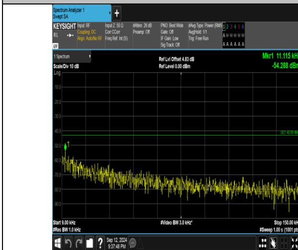
Band4_15MHz_QPSK_20325_75RB#0_0.009~0.15_0.009~0.15
