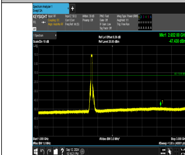
Band4_20MHz_16QAM_20050_100RB#0_1000~3000_1000~3000
