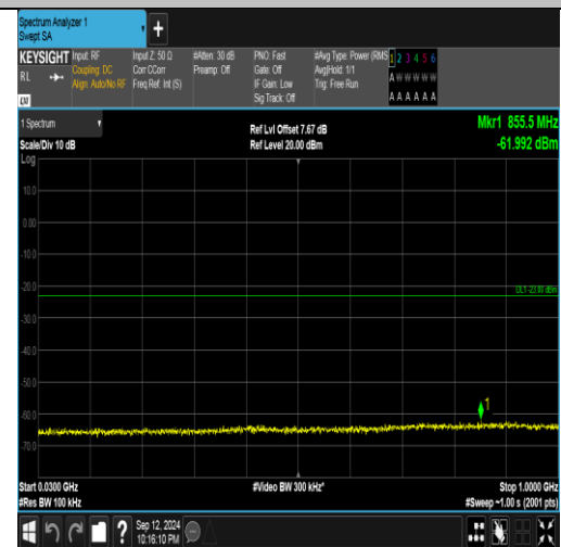
Band4_20MHz_16QAM_20050_100RB#0_30~1000_30~1000
