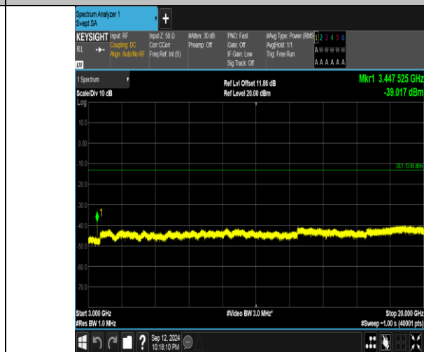
Band4_20MHz_16QAM_20175_1RB#0_3000~20000_3000~20000
