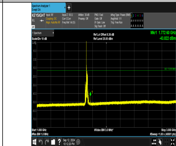
Band4_20MHz_QPSK_20050_1RB#0_1000-3000_1000-3000
