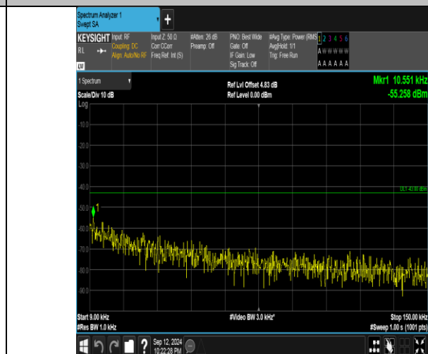
Band4_20MHz_16QAM_20300_1RB#0_0.009-0.15_0.009-0.15
