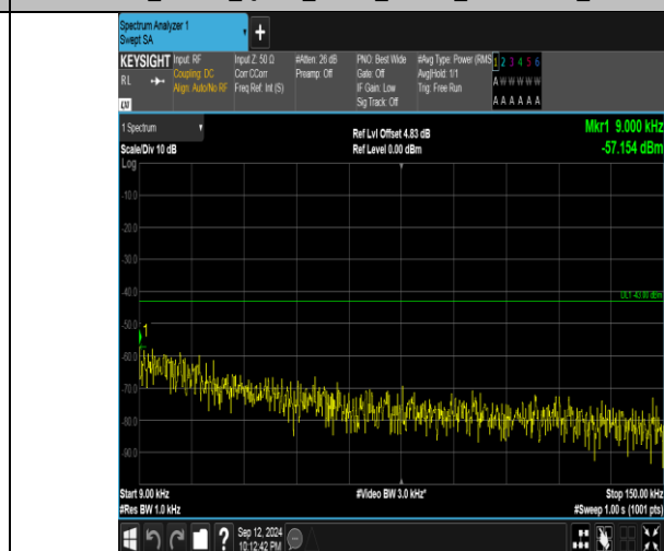
Band4_20MHz_16QAM_20050_1RB#0_0.009-0.15_0.009-0.15
