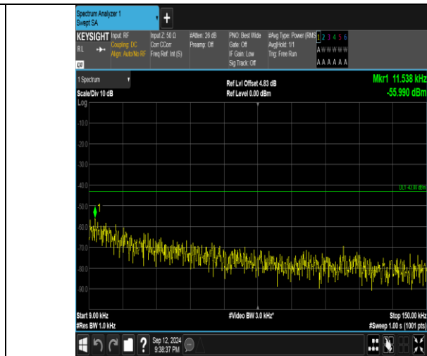
Band4_15MHz_16QAM_20325_75RB#0_0.009~0.15_0.009~0.15
