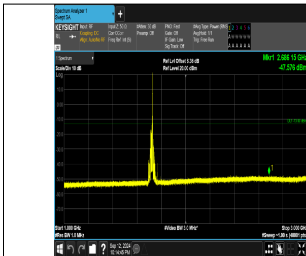
Band4_20MHz_16QAM_20050_1RB#99_1000~3000_1000~3000
