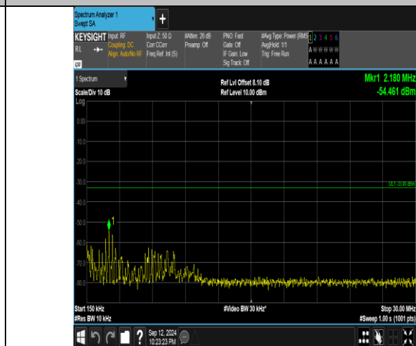
Band4_20MHz_QPSK_20300_1RB#99_0.15~30_0.15~30
