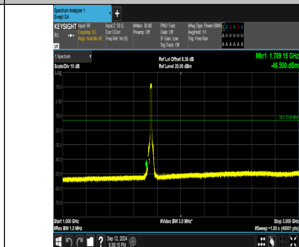
Band4_15MHz_QPSK_20325_75RB#0_1000~3000_1000~3000
