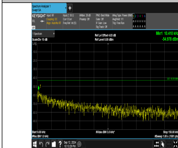
Band4_20MHz_QPSK_20050_1RB#99_0.009~0.15_0.009~0.15
