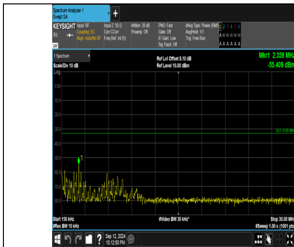
Band4_20MHz_16QAM_20050_1RB#0_0.15~30_0.15~30
