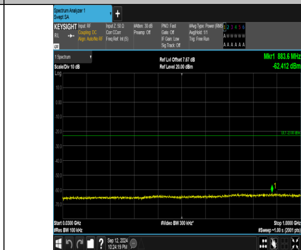
Band4_20MHz_16QAM_20300_1RB#99_30~1000_30~1000
