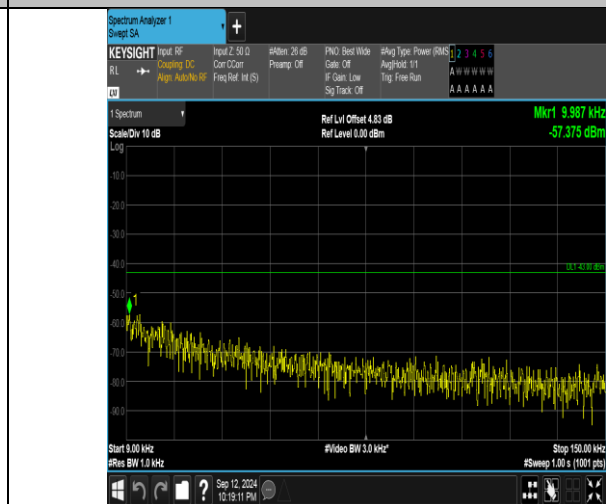
Band4_20MHz_16QAM_20175_1RB#99_0.009~0.15_0.009~0.15
