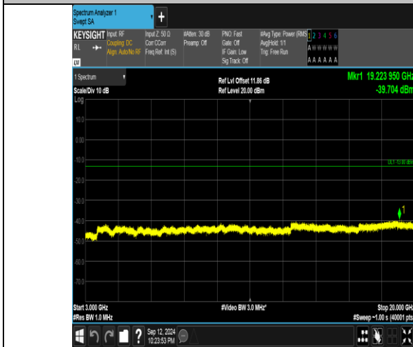
Band4_20MHz_QPSK_20300_1RB#99_3000~20000_3000~20000
