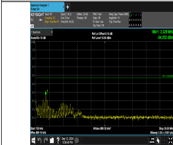
Band4_15MHz_16QAM_20325_75RB#0_0.15~30_0.15~30
