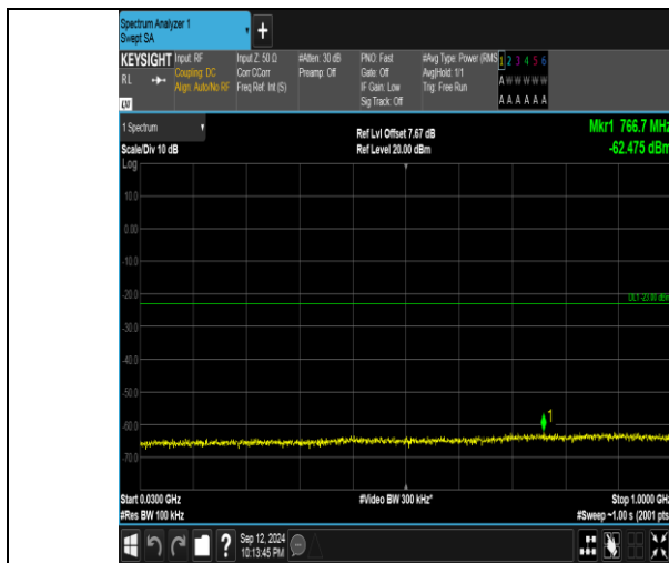
Band4_20MHz_QPSK_20050_1RB#99_30~1000_30~1000
