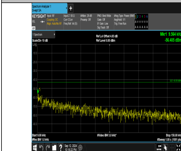
Band4_20MHz_QPSK_20175_1RB#99_0.009~0.15_0.009~0.15
