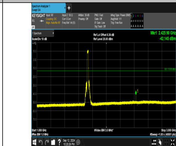
Band4_20MHz_QPSK_20175_100RB#0_1000~3000_1000~3000
