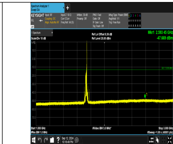
Band4_20MHz_QPSK_20175_1RB#99_1000~3000_1000~3000
