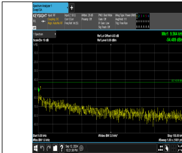
Band4_20MHz_QPSK_20300_1RB#0_0.009-0.15_0.009-0.15
