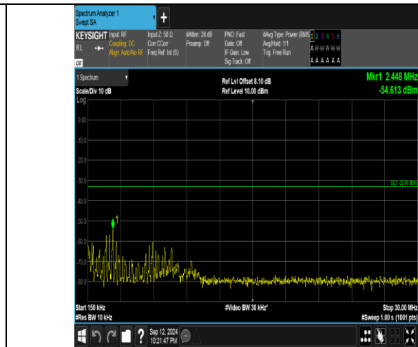
Band4_20MHz_QPSK_20300_1RB#0_0.15-30_0.15-30
