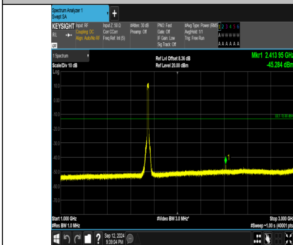
Band4_15MHz_16QAM_20325_75RB#0_1000~3000_1000~3000
