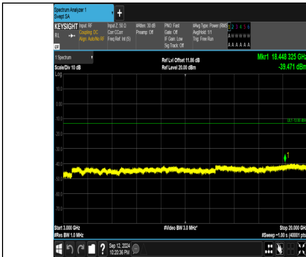
Band4_20MHz_QPSK_20175_100RB#0_3000~20000_3000~20000
