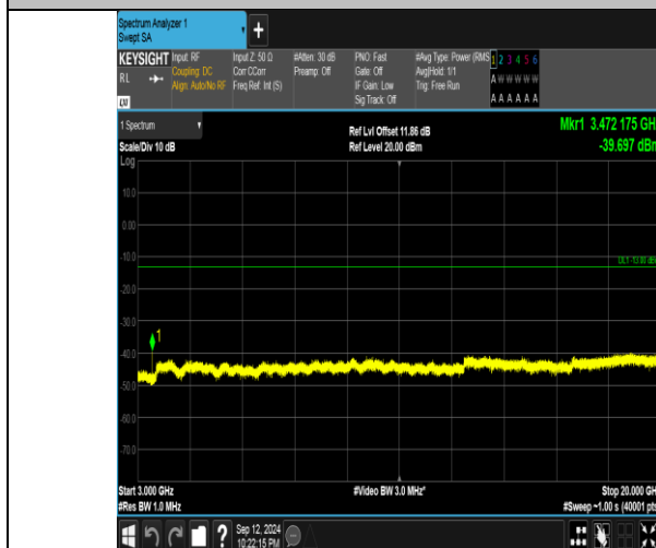
Band4_20MHz_QPSK_20300_1RB#0_3000-20000_3000-20000
