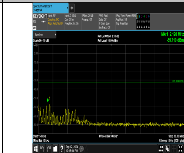
Band4_20MHz_QPSK_20050_100RB#0_0.15~30_0.15~30
