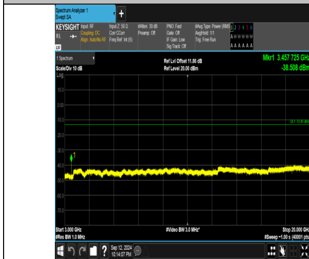
Band4_20MHz_QPSK_20050_1RB#99_3000~20000_3000~20000
