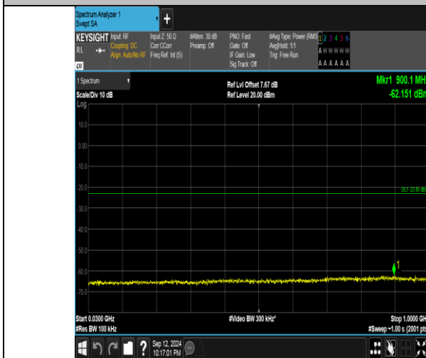
Band4_20MHz_QPSK_20175_1RB#0_30-1000_30-1000
