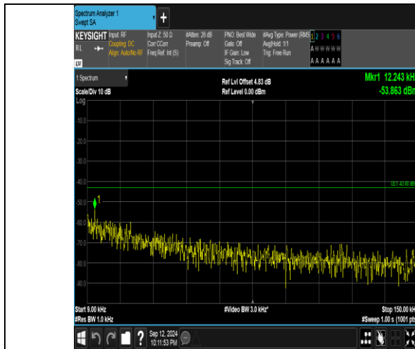
Band4_20MHz_QPSK_20050_1RB#0_0.009-0.15_0.009-0.15
