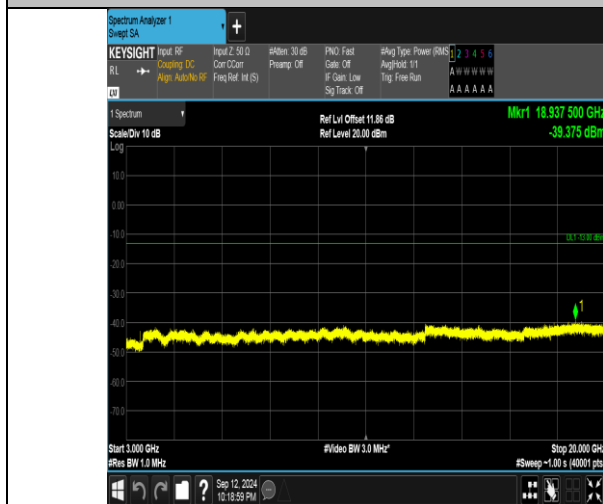
Band4_20MHz_QPSK_20175_1RB#99_3000~20000_3000~20000
