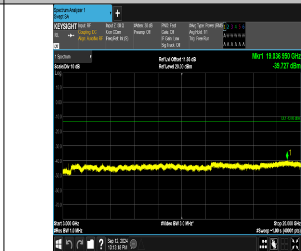
Band4_20MHz_16QAM_20050_1RB#0_3000~20000_3000~20000
