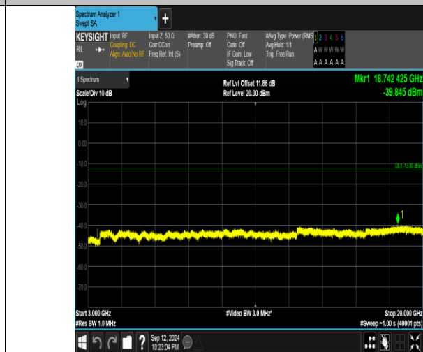
Band4_20MHz_16QAM_20300_1RB#0_3000~20000_3000~20000
