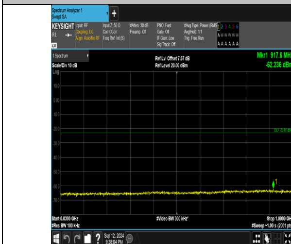
Band4_15MHz_QPSK_20325_75RB#0_30~1000_30~1000
