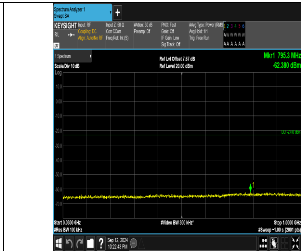
Band4_20MHz_16QAM_20300_1RB#0_30~1000_30~1000
