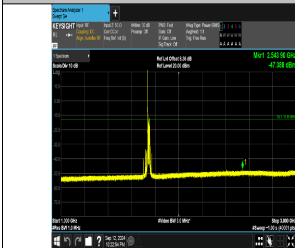
Band4_20MHz_16QAM_20300_1RB#0_1000~3000_1000~3000
