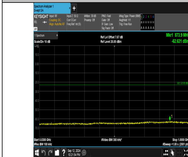
Band4_20MHz_QPSK_20300_1RB#0_30-1000_30-1000
