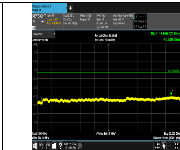
Band4_20MHz_16QAM_20050_1RB#99_3000~20000_3000~20000
