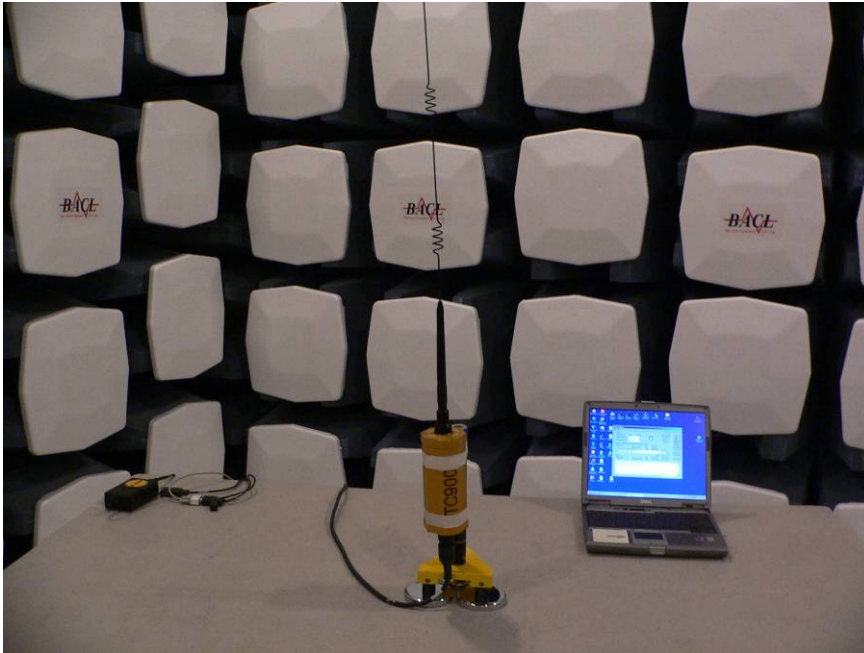
Radiated Emissions - Front View with dipole whip antenna
