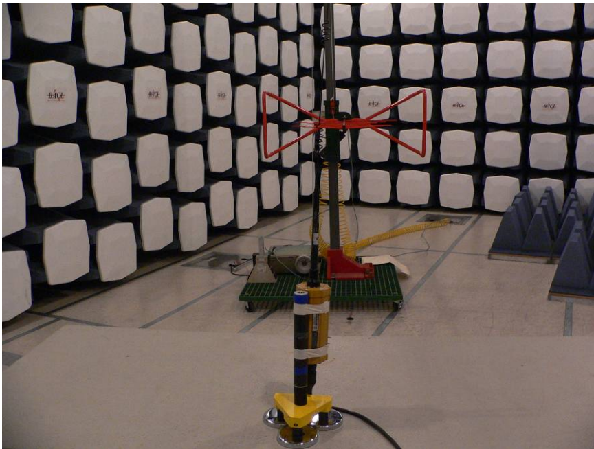
Radiated Emissions - Rear View with dipole whip antenna
