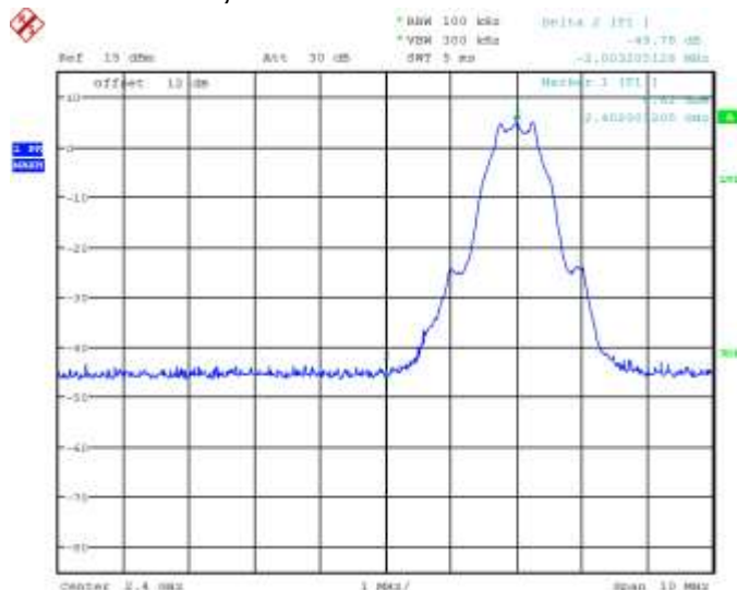
Figure 5-53: Band Edge Compliance LE, Channel 0
