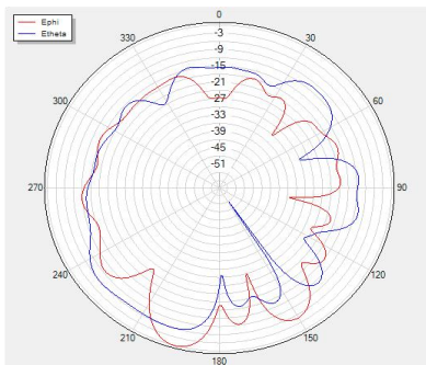
Phi=90 freq=2400MHz
