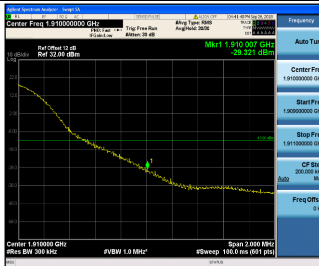
Band2_20MHz_16QAM_19100_1RB#99
