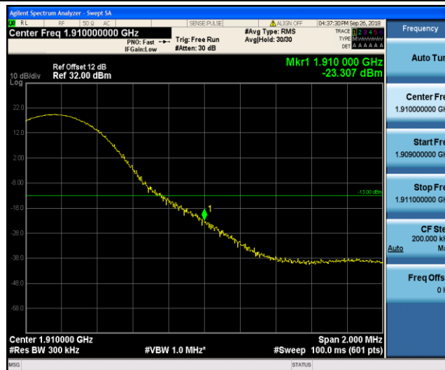
Band2_15MHz_QPSK_19125_1RB#74
