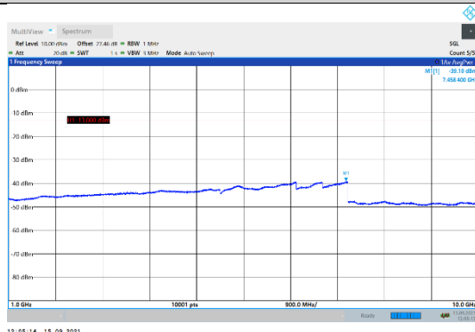
N5-15kHz-20MHz-DFT-QPSK-Low-Edge_1RB_Left-1000-10000-PASS
