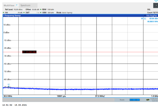
N7-15kHz-10MHz-DFT-QPSK-Mid-Edge_1RB_Left-30-1000-PASS
