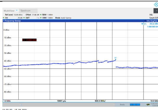
N5-15kHz-15MHz-DFT-QPSK-Mid-Edge_1RB_Left-1000-10000-PASS
