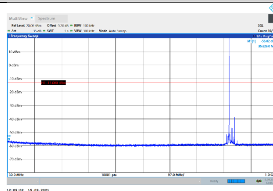
N5-15kHz-20MHz-DFT-QPSK-Low-Edge_1RB_Left-30-1000-PASS
