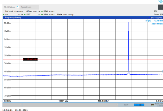
N7-15kHz-10MHz-DFT-QPSK-High-Edge_1RB_Left-1000-3000-PASS
