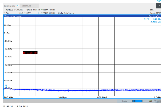
N7-15kHz-5MHz-DFT-QPSK-High-Edge_1RB_Left-30-1000-PASS
