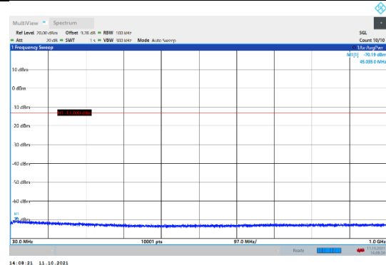
N66-15kHz-20MHz-DFT-QPSK-High-Edge_1RB_Left-30-1000-PASS
