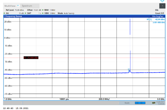
N7-15kHz-5MHz-DFT-QPSK-High-Edge_1RB_Left-1000-3000-PASS
