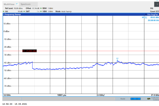
N7-15kHz-15MHz-DFT-QPSK-Low-Edge_1RB_Left-3000-27000-PASS
