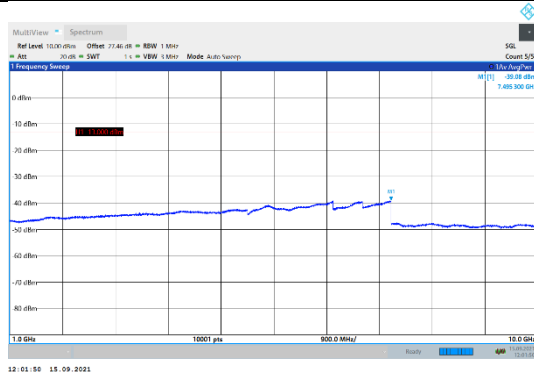
N5-15kHz-15MHz-DFT-QPSK-Low-Edge_1RB_Left-1000-10000-PASS
