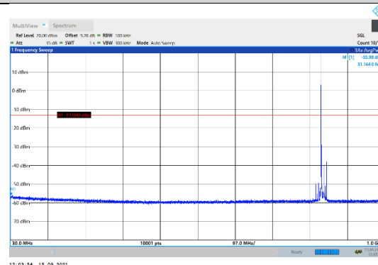
N5-15kHz-15MHz-DFT-QPSK-High-Edge_1RB_Left-30-1000-PASS
