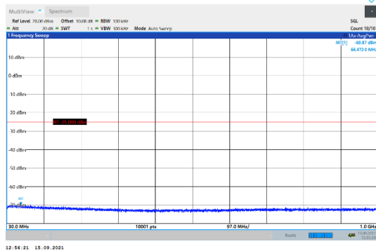
N7-15kHz-15MHz-DFT-QPSK-High-Edge_1RB_Left-30-1000-PASS
