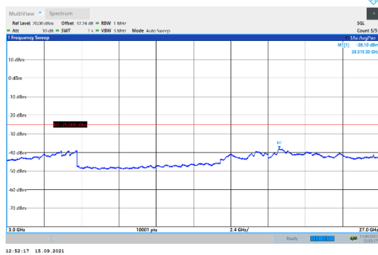
N7-15kHz-10MHz-DFT-QPSK-Mid-Edge_1RB_Left-3000-27000-PASS
