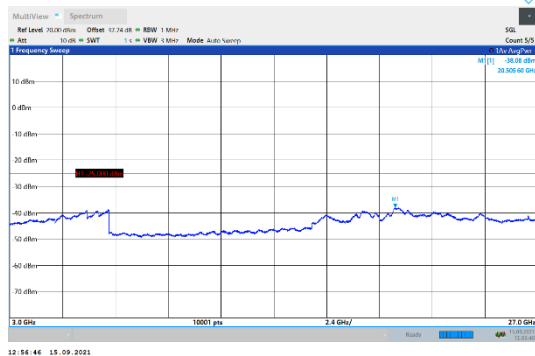
N7-15kHz-15MHz-DFT-QPSK-High-Edge_1RB_Left-30-1000-PASS
