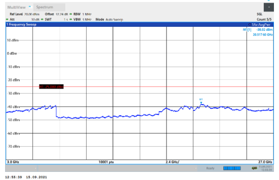
N7-15kHz-15MHz-DFT-QPSK-Mid-Edge_1RB_Left-3000-27000-PASS
