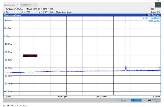
N7-15kHz-15MHz-DFT-QPSK-High-Edge_1RB_Left-1000-3000-PASS
