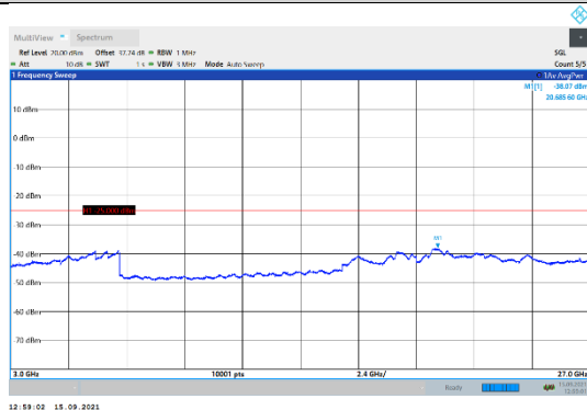
N7-15kHz-20MHz-DFT-QPSK-Mid-Edge_1RB_Left-3000-27000-PASS
