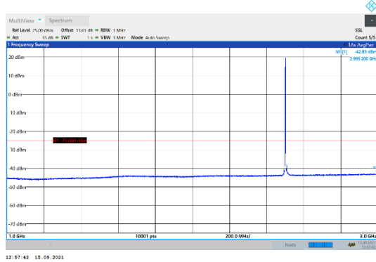
N7-15kHz-20MHz-DFT-QPSK-Low-Edge_1RB_Left-1000-3000-PASS
