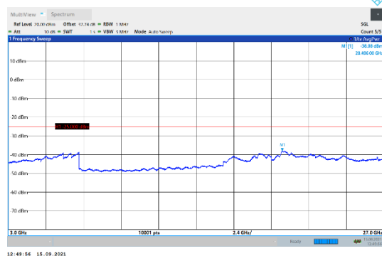
N7-15kHz-5MHz-DFT-QPSK-High-Edge_1RB_Left-3000-27000-PASS
