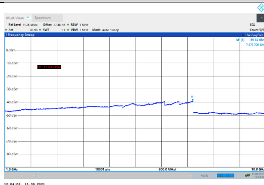
N5-15kHz-15MHz-DFT-QPSK-High-Edge_1RB_Left-1000-10000-PASS
