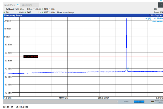
N7-15kHz-5MHz-DFT-QPSK-Mid-Edge_1RB_Left-1000-3000-PASS
