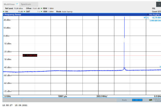
N7-15kHz-15MHz-DFT-QPSK-Mid-Edge_1RB_Left-1000-3000-PASS
