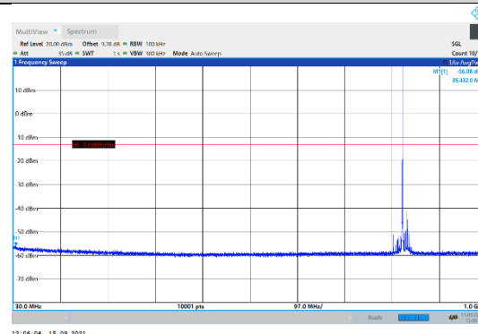
N5-15kHz-20MHz-DFT-QPSK-Mid-Edge_1RB_Left-30-1000-PASS
