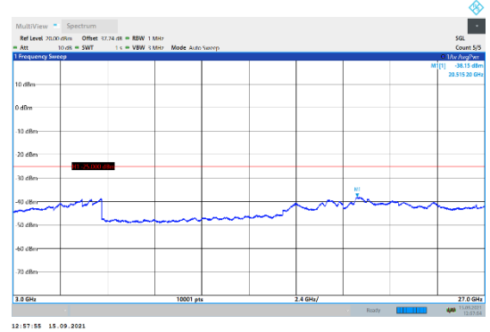
N7-15kHz-20MHz-DFT-QPSK-Low-Edge_1RB_Left-3000-27000-PASS
