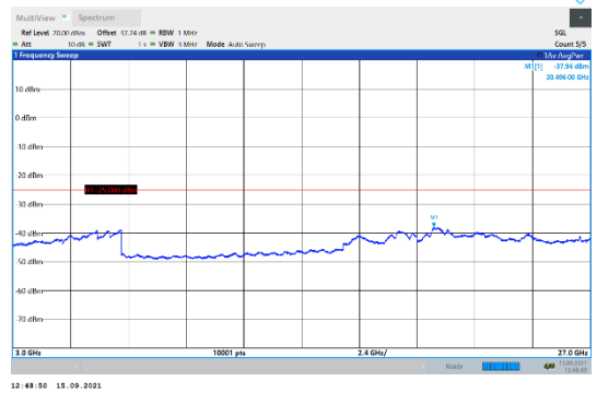
N7-15kHz-5MHz-DFT-QPSK-Mid-Edge_1RB_Left-3000-27000-PASS
