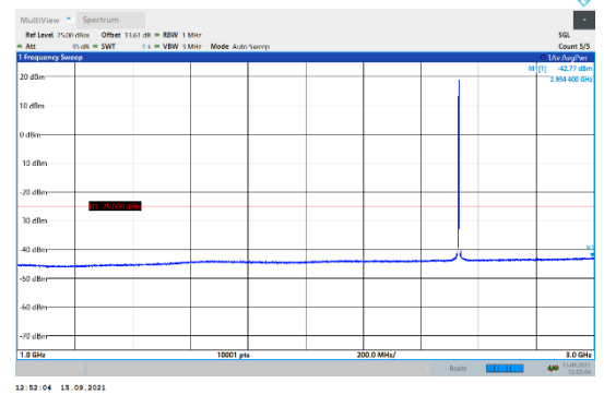
N7-15kHz-10MHz-DFT-QPSK-Mid-Edge_1RB_Left-1000-3000-PASS
