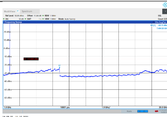
N66-15kHz-20MHz-DFT-QPSK-High-Edge_1RB_Left-1000-20000-PASS
