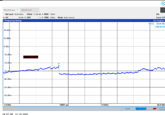
N66-15kHz-20MHz-DFT-QPSK-Mid-Edge_1RB_Left-1000-20000-PASS
