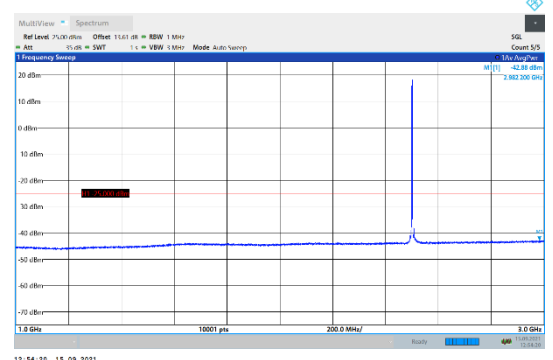
N7-15kHz-10MHz-DFT-QPSK-High-Edge_1RB_Left-3000-27000-PASS
