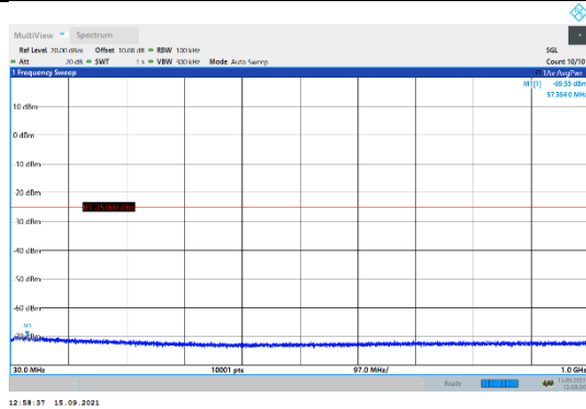
N7-15kHz-20MHz-DFT-QPSK-Mid-Edge_1RB_Left-30-1000-PASS
