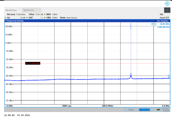
N7-15kHz-20MHz-DFT-QPSK-Mid-Edge_1RB_Left-1000-3000-PASS
