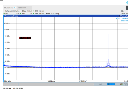
N5-15kHz-15MHz-DFT-QPSK-Mid-Edge_1RB_Left-30-1000-PASS
