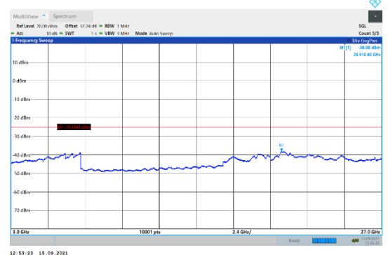
N7-15kHz-10MHz-DFT-QPSK-High-Edge_1RB_Left-3000-27000-PASS
